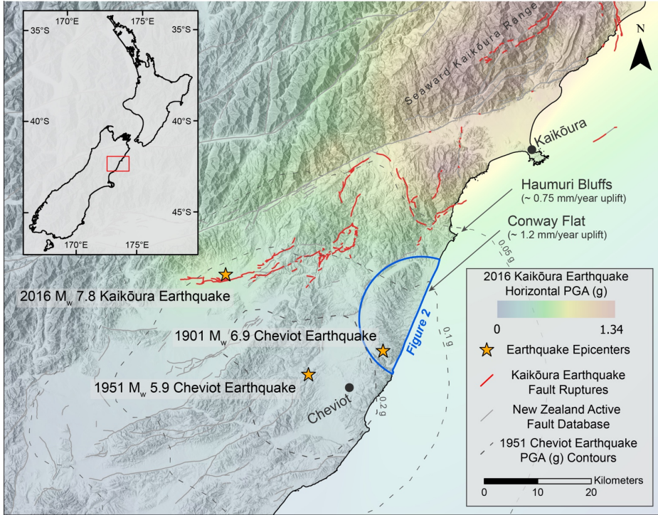
90 Figure 1: Overview of the Kaikōura Coast. Horizontal Peak Ground Acceleration (PGA) from the 2016 Mw 7.8 Kaikōura Earthquake (Bradley et al., 2017) is shown as a color ramp over a multidirectional hillshade derived from an 8 m DEM (LINZ, 2022). PGA from the 1951 Mw 5.9 Cheviot Earthquake (ShakeMapNZ; Horspool et al., 2015) is shown as dashed grey contours radiating away from the earthquake epicenter. Faults in the New Zealand Active Fault Database (Langridge et al., 2016) are shown as solid grey lines while faults that ruptured to the surface during the 2016 Kaikōura earthquake (Litchfield et al. 2018) are 95 shown as solid red lines. Late Pleistocene uplift rates are reported at Haumuri Bluffs and Conway Flat (Barrell et al., 2022). The location of Figure 2 is shown as a solid semi-circular blue outline.
