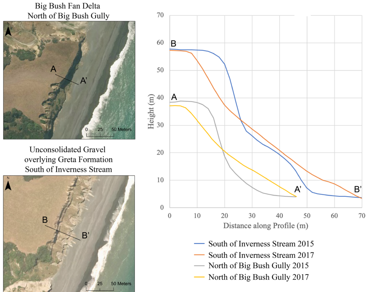
Figure R2. Comparative Cliff Profiles. Profile A is taken from a cliff face that consists entirely of fan delta deposits. Profile B is taken from a cliff face that consists of Greta Formation overlain by unconsolidated gravels. The contact between underlying Greta and overlying unconsolidated sediment occurs at approximately 30 m height in Profile B.
