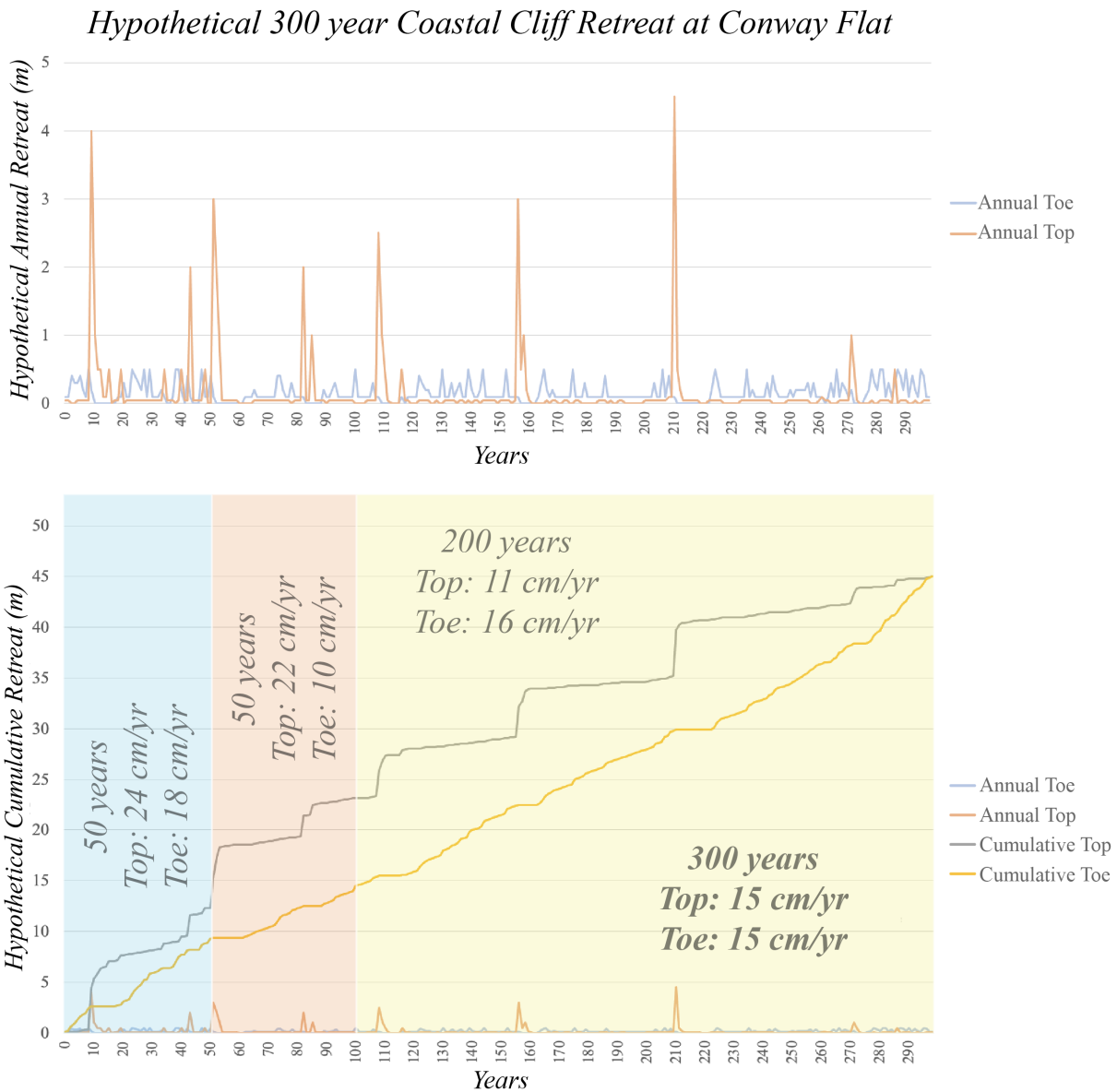
Figure R1. Hypothetical cliff-toe and cliff-top retreat and cumulative retreat at Conway Flat. Over multidecadal timescales, variability in cliff-top and cliff-toe retreat can result in substantially different retreat rates.
