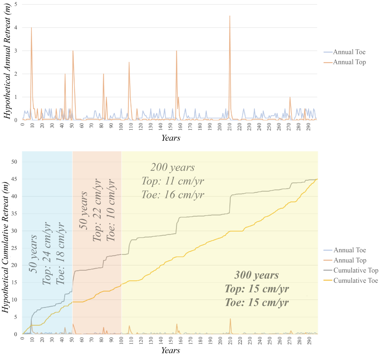
Figure R1. Hypothetical cliff-toe and cliff-top retreat and cumulative retreat at Conway Flat. Over multidecadal timescales, variability in cliff-top and cliff-toe retreat can result in substantially different retreat rates.
