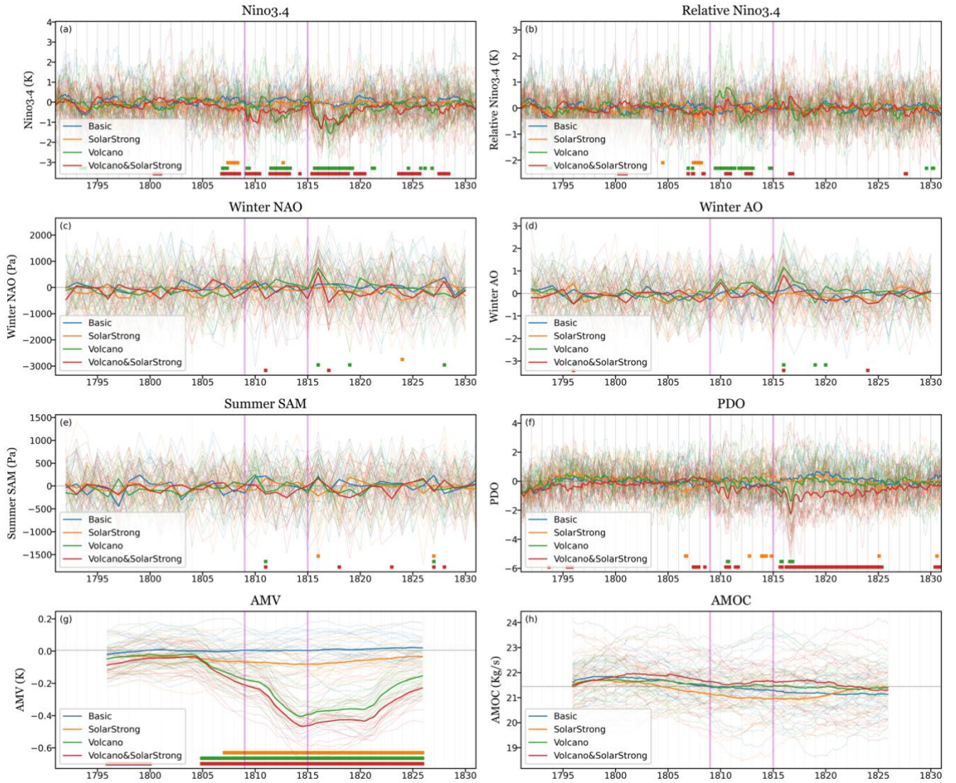
690 Figure 10: As in Figure 2, but for (a) the Niño3.4 index (K), (b) Relative Niño3.4 index (K), (c) Winter NAO index (Pa), (d) Winter AO index, (e) Summer SAM index (Pa), (f) PDO index, (g) AMV index (K), (h) AMOC index (kg s -1 ). The Basic experiment is in blue, SolarStrong is in orange, Volcano is in green, and Volcano&SolarStrong is in red.
