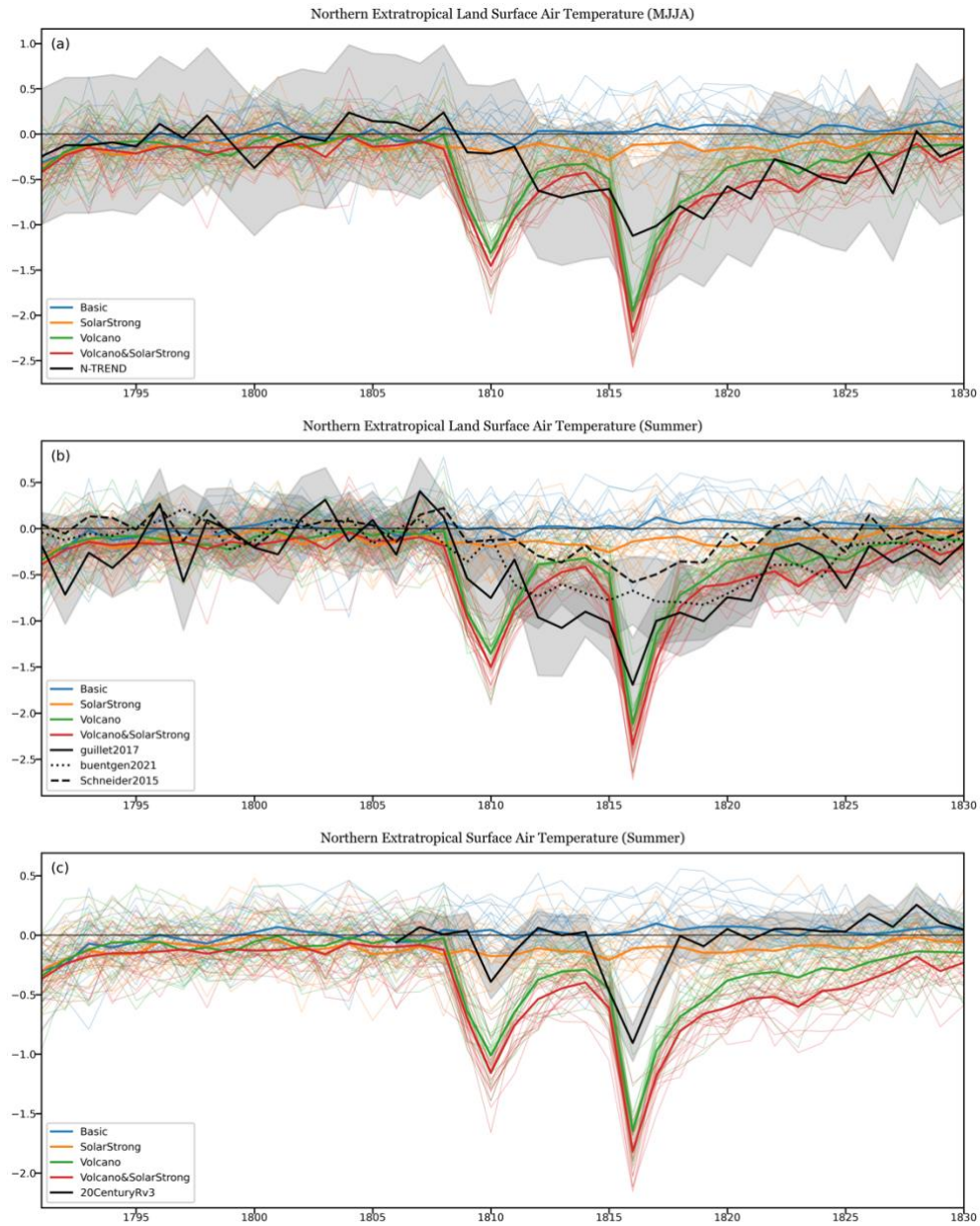
705 Figure 12: (a) Northern extratropical ( 30^{\circ} N to 90^{\circ} N) May to August land surface air temperature anomalies Basic (blue), SolarStrong (orange), Volcano (green), and Volcano&SolarStrong (red) experiments, (b) for northern extratropical summer land 710 surface air temperature, (c) for northern extratropical summer surface air temperature. The black lines are for the anomalies from reconstruction projects and the gray shadings are the uncertainties. The reconstruction anomalies are offset with the difference from the ensemble mean of the Basic experiment over 1800-1808 for lining with the Basic experiment. In (a), the uncertainty of the N- TREND (Wilson et al., 2016) is provided in the dataset. In (b), the uncertainty of guillet2017 (solid; Guillet et al., 2017) is provided in the dataset and the uncertainty for the buentgen2021 is calculated by the one standard deviation of the 15 ensemble members (R1 to R15; dotted; Büntgen et al, 2021). And Schneider2015 is dashed (Schneider et al., 2015). In (c), the spread of 20th Century Reanalysis v3 (20CenturyRv3) is calculated by the one standard deviation of the 80 ensemble members.
