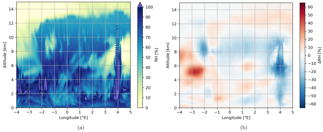
Figure 8. Vertical cross-sections on along 44°N of (a) the AROME background RH and (b) the difference of analysis minus background RH. Sawtooth features visible at 4°E are interpolation artefacts caused by the grid's irregularity. Results for 08 Aug. 2018, 23:00 UTC and model experiment LDA n C .
