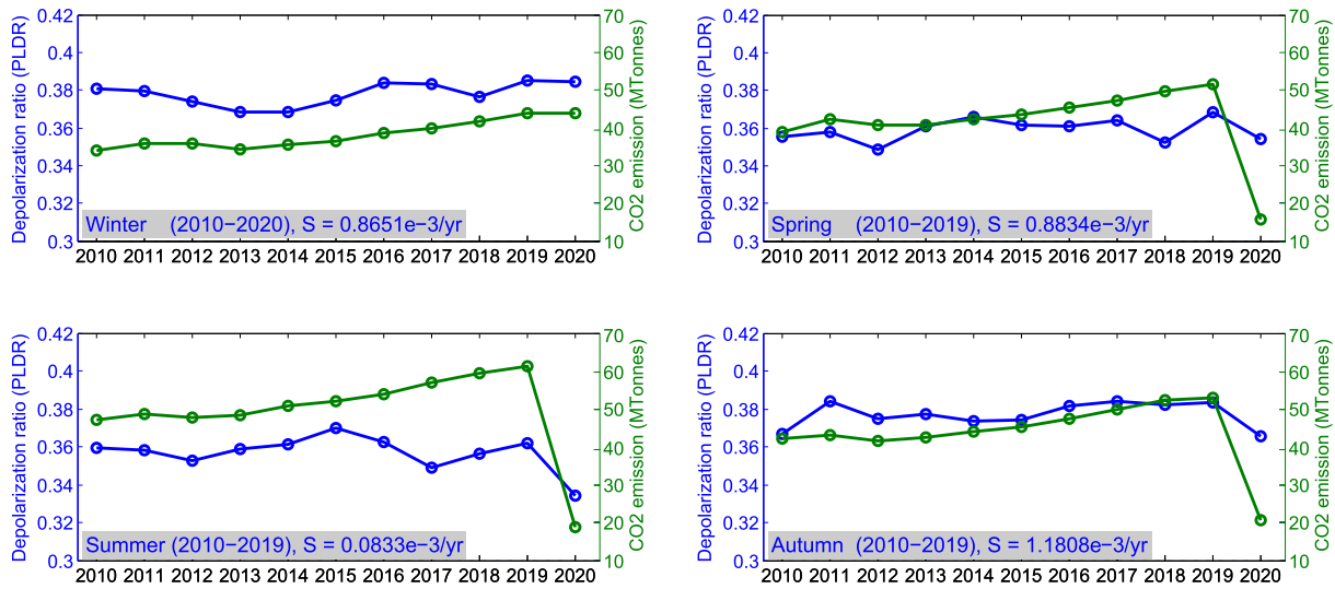
Figure 10. Long-term trends in cirrus PLDR in different seasons and their correlations with the corresponding CO2 emissions from aviation in Europe. There are increasing trends in PLDR as well as CO2 emissions from aviation in all seasons in the 10 years before COVID-19. The correlation analysis between both parameters shows a strong correlation in winter, spring, and autumn, but a weak correlation in summer.
