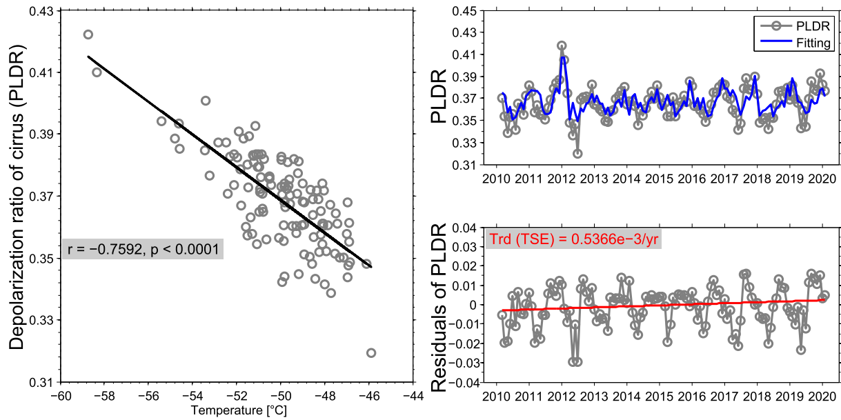
Figure 8. Left panel: The gray circles stand for the correlation between the monthly medians of cirrus PLDR and the corresponding ambient temperatures and the black line for the linear fitting line derived from all data points. Right panels: the monthly medians of cirrus PLDR during the period from March 2010 to February 2020 are shown in gray and the regressed values with the first degree polynomial in blue (Right-upper panel); The residuals after removing the regressed values from the monthly medians of PLDR are shown in gray and the linear fitting line with the Theil-Sen estimator (TSE) method in red, with the long-term trend of 0.54e-3/\text{yr} indicated on the plots (Right-lower panel).
