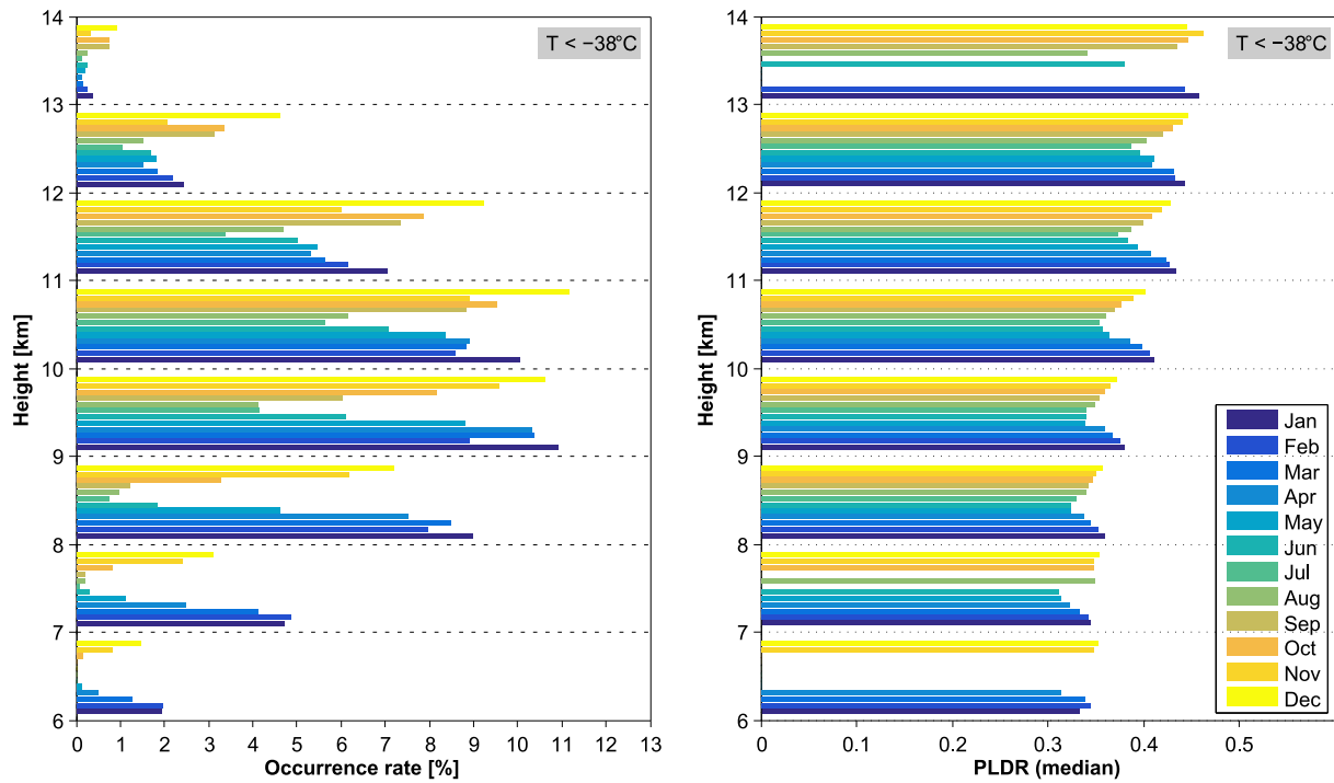
Figure 4. Distributions of the occurrence rate (OR) and PLDR of cirrus clouds in each 1-km altitude bin. Both parameters follow a seasonal cycle: cirrus clouds in winter are characterized by larger values of PLDR and higher occurrence rates than in summer. Furthermore, cirrus clouds appear within the full altitude range from 6 to 13 km in the winter months but only within the altitudes from \sim 9 to 12.5 km in summer.
