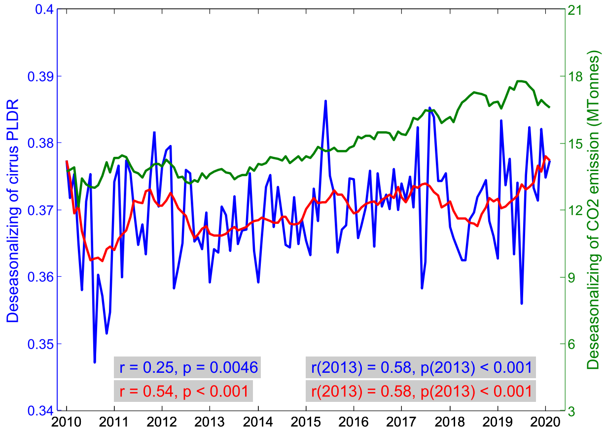
Figure 9. Comparison between the deseasonalized time series of cirrus PLDR (in blue) and the corresponding deseasonalized CO 2 emissions from aviation in Europe (in green). The annual mean variations of the deseasonalized PLDR are overplotted with a 12-point moving average smooth. The correlation coefficients between both parameters for a full period as well as for a shorter period from January 2013 are calculated and indicated on the plot, which are all at the confidence level above 99.5%.
