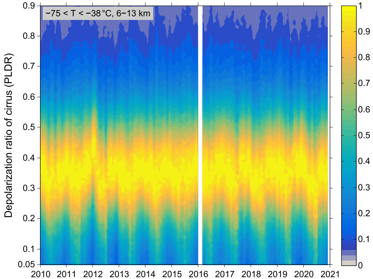
Figure 3. Number densities of the cirrus PLDR distribution normalized for each month from January 2010 to December 2020. The data are derived from the observations at the typical cirrus heights from 6 to 13 km and at temperatures between -75 and -38^{\circ}\text{C} . The color codes are used to visualize the relative number densities of scatter point data, with the maximum number density indicated by 1 in the color bar.
