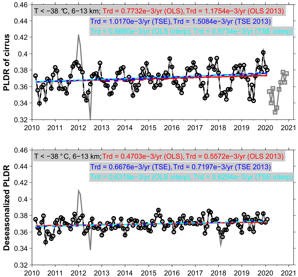
Figure 5. Upper panel: Medians of cirrus PLDR in different month from March 2010 to February 2020 shown in gray lines and during the COVID-19 pandemic starting from March 2020 shown in squares. The results are derived from both day- and night-time lidar measurements of CALIPSO. Both OLS and TSE methods are applied to determine the long-term trends (i.e., slopes) of the cirrus PLDR (medians) and the results are indicated on the plot (see text for details). Lower Panel: The long-term trends determined from the deseasonalized time series of cirrus PLDR (medians).
