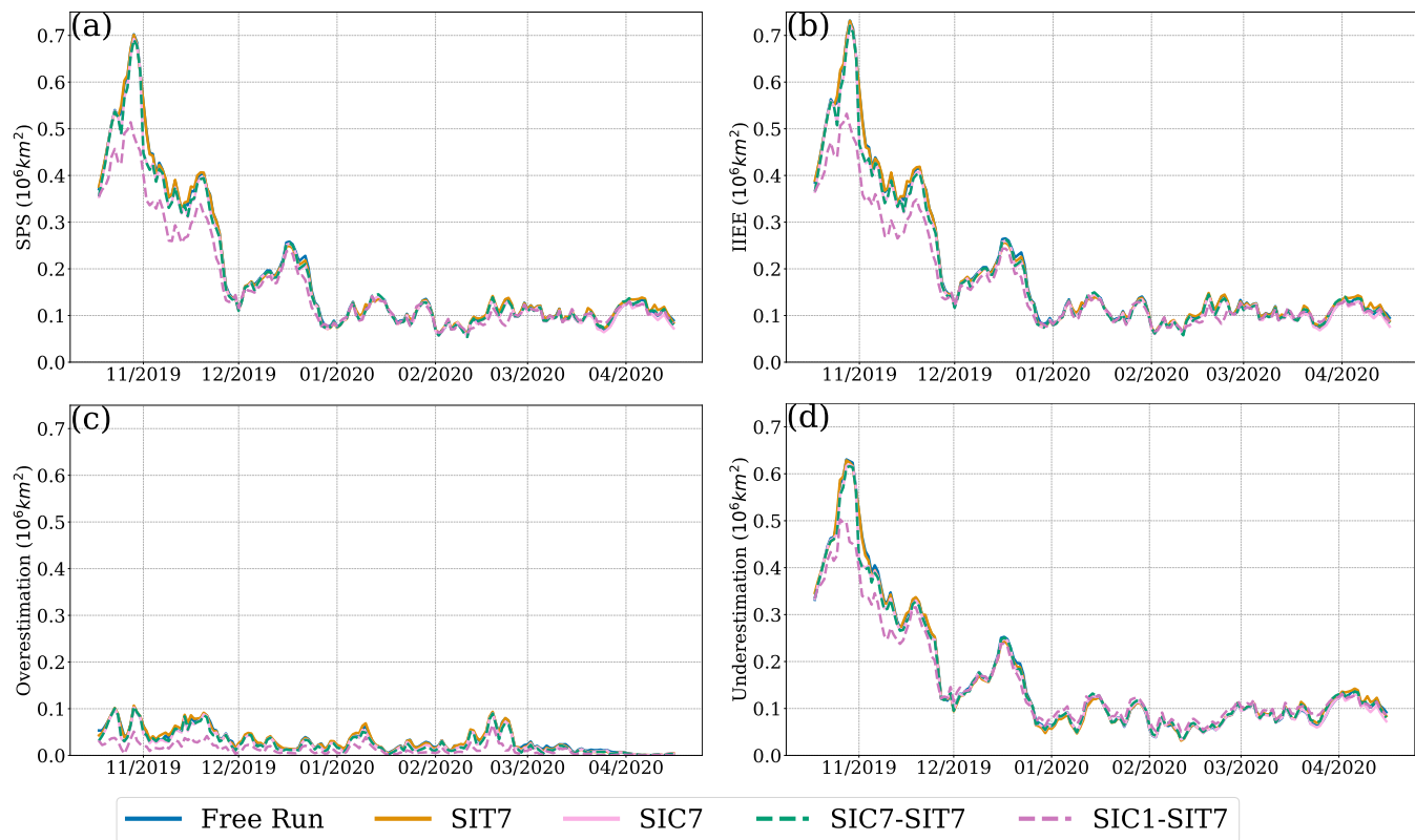
Figure 4. Metrics of sea ice extent extent validated against OSI-SAF SIC over time. (a) Spatial probability score (SPS) is calculated using the full ensemble forecasts; (b) Integrated ice-edge error (IIEE) is calculated using the ensemble means and split between its over- and underestimation components in panels(c)(d), respectively, which indicate the amounts of over-and underestimated in modeled SIE from the observations.
