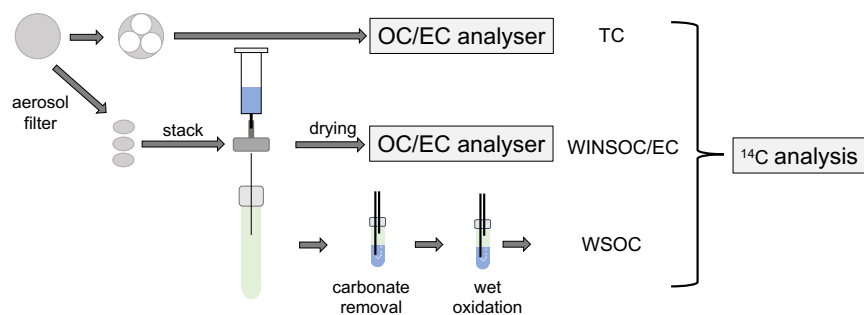
955 960 Figure 1: Separation of the different fractions for ^{14}\text{C} analysis starting from the aerosol filters. One or multiple circular quartz fibre filter punches are stacked and intercalated in the water extraction set-up. The residual filter material used for WINSOC and EC analysis after drying, and the extract oxidised by chemical wet oxidation. The remaining filter material is used for TC analysis.
