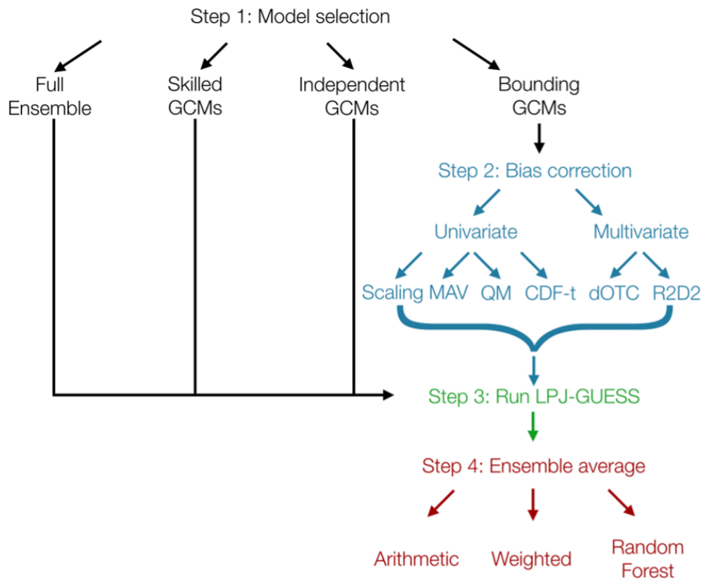
Figure 1. Schematic for study set-up. All terms are defined in the text and the key steps are described in the text. GCM refers to Global circulation models . MAV, QM, CDF-t, dOTC and R2D2 represent five different bias correction methods (Mean and Variance, Quantile Mapping, Cumulative Distribution Function, Dynamical Optimal Transport Correction, and Rank Resampling For Distributions and Dependences, respectively).
