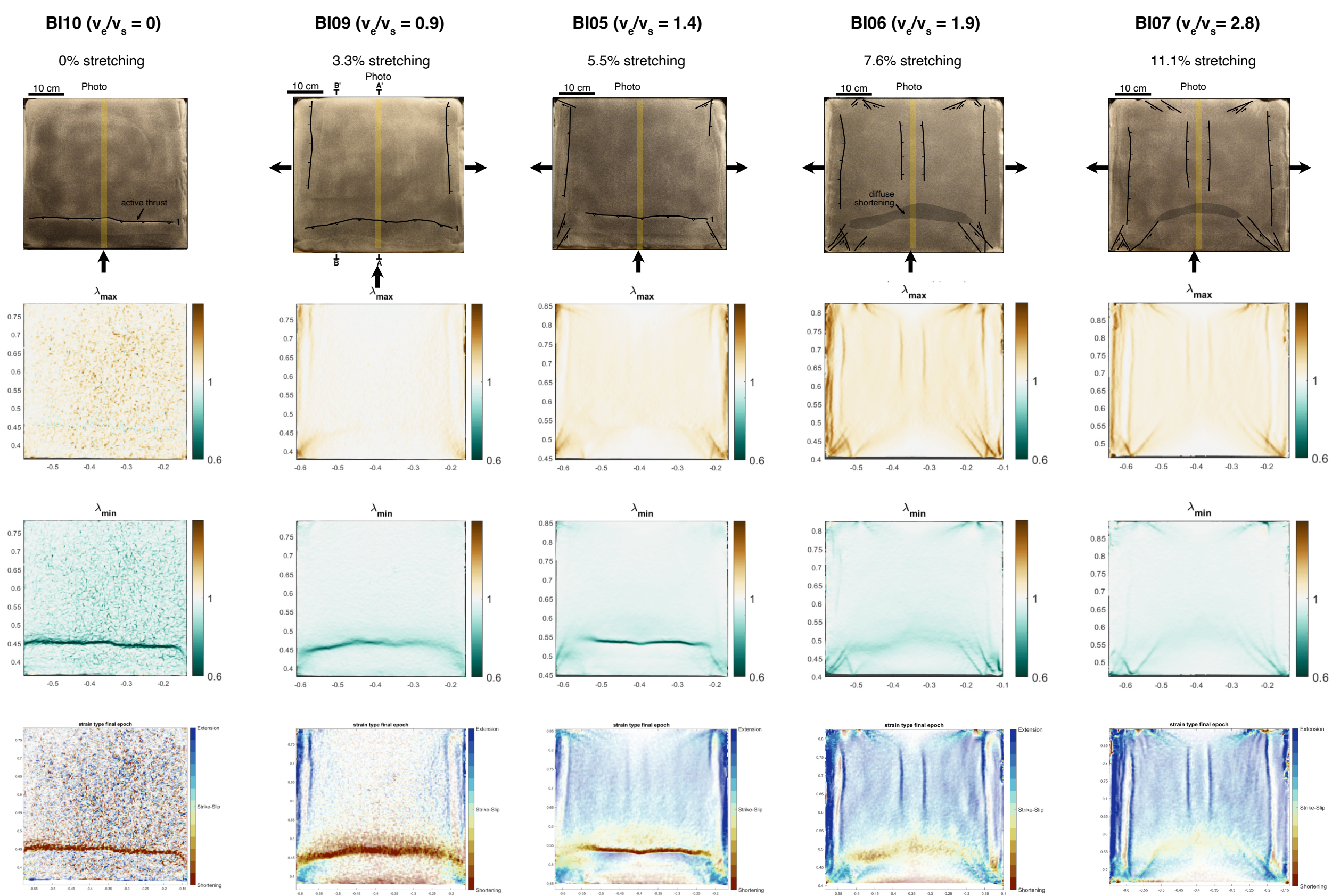
Fig. SM1: Interpreted pictures, principal stretches \lambda_{\max} , \lambda_{\min} ( \lambda = 1 represents no length change) and strain type after 4% of along-y shortening for brittle models BI10, BI09, BI05, BI06, and BI07: shortening (red), strike-slip (green) and stretching (blue), with intermediate, oblique deformation at intermediate colors. The corresponding amount of along-x stretching is indicated at the top.
