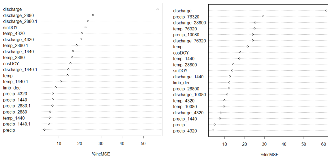
Figure 2 Left: Variable importance at gauge Vent. Right: Variable importance at gauge Vernagt
