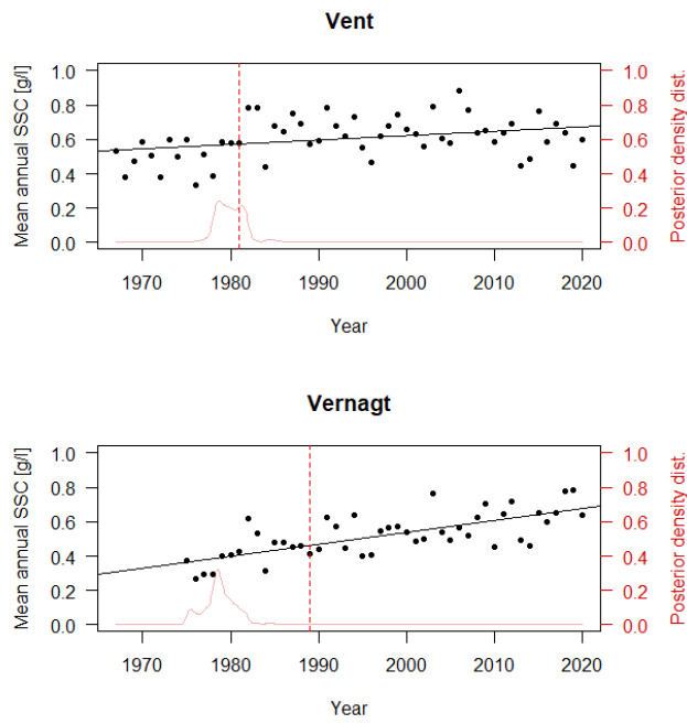
Figure 1 Mean annual SSC estimates over time with change points determined by Pettitt test (dashed) and with the mcp package (solid line).
