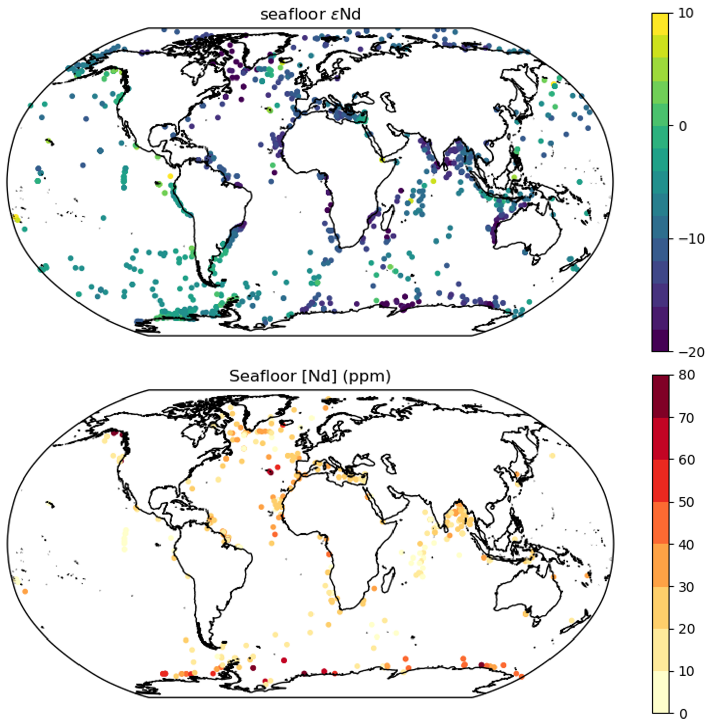
Figure 1: seafloor \epsilon\text{Nd} and seafloor Nd concentration provided by Robinson et al. (2021)
