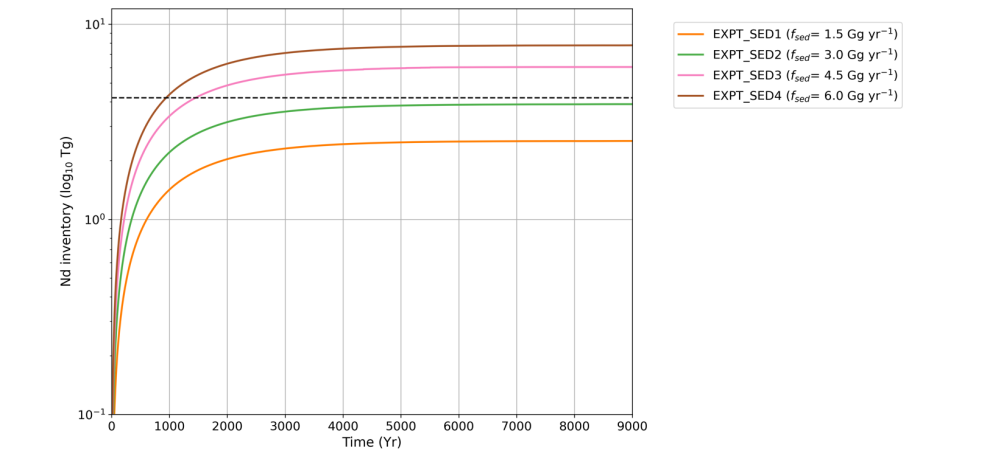
Figure 13: Global Nd inventory (Tg) simulated with different values for the total sediment flux tuning parameter ( f_{sed} ) as indicated. Dashed line represents the estimated global marine Nd inventory of 4.2 Tg from Tachikawa et al. (2003) used as an approximate target for the simulations. Note the logarithmic y-axis scale.
