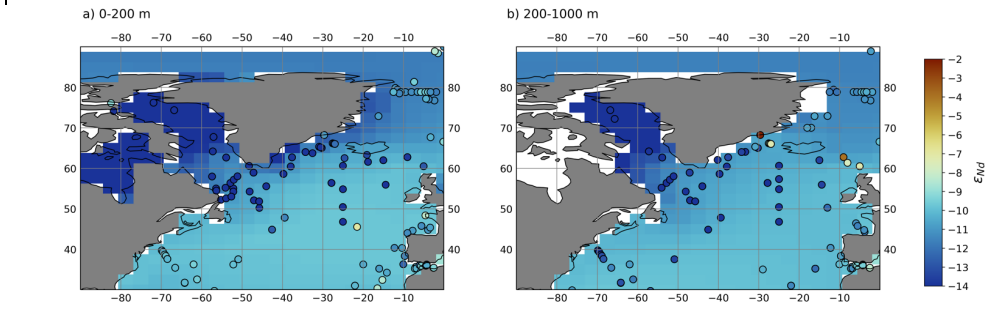
Figure 17: Volume-weighted distributions of \epsilon_{Nd} in simulation EXPT_SED2 split into two different depth bins, (a) shallow (0-200 m), and (b) intermediate (200-1,000 m) within the North Atlantic and Labrador Sea basins. Water column measurements from within each depth bin (Osborne et al., 2017, 2015; GEOTRACES Intermediate Data Product Group, 2021) are superimposed as filled circles on the same colour scale. Note that Iceland is not resolved in FAMOUS (Jones, 2003).
