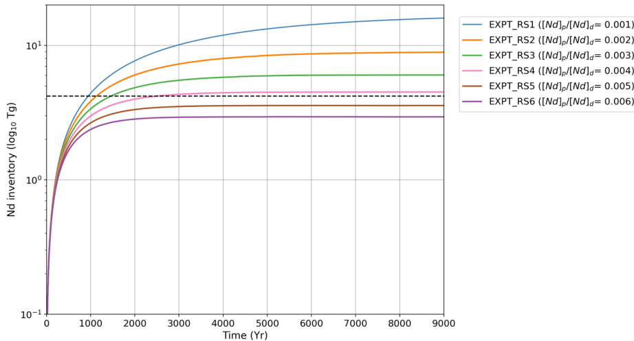
Figure 9: Global Nd inventory (g) simulated with different values for the reversible scavenging tuning parameter, [Nd]_p/[Nd]_d , as indicated. Dashed line represents the estimated global marine Nd inventory of 4.2 \times 10^{12} g by Tachikawa et al. (2003) used as a first-order target for our simulations.
