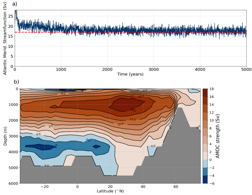
305 Figure 3: Atlantic Meridional streamfunction for a 5,000-year simulation using control (XPDA), showing (a) the maximum 310 streamfunction in time series (red dashed line indicates RAPID-AMOC 2004-2012 averaged AMOC strength at 26.5° N of 17.2 Sv; McCarthy et al., 2015), and (b) the zonal integration calculated from the last one hundred years.
