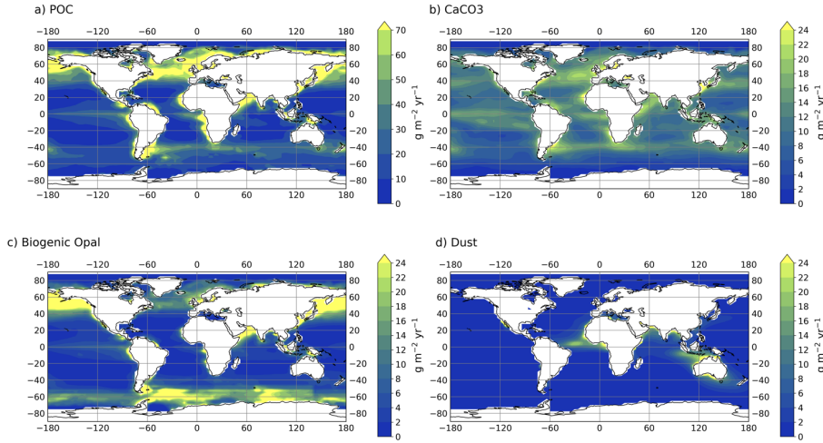
Figure 7: Particle export fields from the ocean surface ( \text{g m}^{-2} \text{yr}^{-1} ). Biogenic particle fields are prescribed using satellite-derived export productivity fields for (a) POC, (b) \text{CaCO}_3 and (c) opal (Dunne et al., 2007, 2012). The dust input fields (d) are annual mean dust deposition simulated for the pre-industrial by the HadGEM2-A GCM (Hopcroft et al., 2015). Note the different scale used for panel (a).
