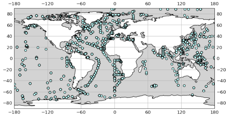
725 Figure 8: Location of marine observational records used in this study, (a) filled orange triangles show the location of dissolved Nd concentration records, and (b) filled sky-blue circles show the location of dissolved \epsilon_{Nd} records.
