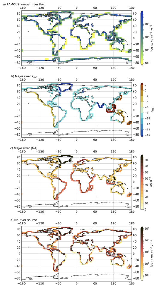
415 Figure 5: (a) Simulated river outflow (RIVER) in FAMOUS, (b) major river \epsilon_{\text{Nd}} , (c) major river [Nd], and (d) the resulting riverine Nd source. The coastal grids in (b) and (c) are prescribed following average [Nd] and \epsilon_{\text{Nd}} estimates of dissolved river runoff to each of the oceans by Goldstein and Jacobsen (1987; see Table 3).
