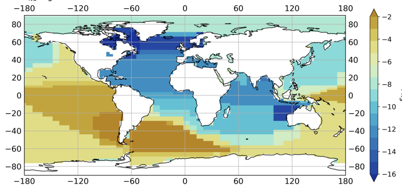
Figure 4: (a) Annual dust deposition taken from the pre-industrial annual mean dust deposition simulated by HadGEM2-A GCM (Hopcroft et al., 2015), and (b) \epsilon_{Nd} signal from dust deposition following Tachikawa et al. (2003) and updated with information from Mahowald et al. (2006) and Blanchet (2019).
