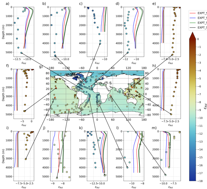
Figure 16: Central panel (g) displays \epsilon_{Nd} at the seafloor (i.e., lowermost box of the ocean model) in simulation EXPT_SED2 (100-year mean from the end of the run), with superimposed water column measurements (Osborne et al., 2017, 2015; GEOTRACES Intermediate Data Product Group, 2021) from \geq 3,000 m shown by filled coloured circles on the same colour scale. Surrounding panels (a-f) and (h-m) display depth profiles of simulated (coloured lines, one per sensitivity simulation with varied f_{sed} ) and measured (filled circles) \epsilon_{Nd} . Larger shifts in the \epsilon_{Nd} between simulations highlight regions most sensitive to the magnitude of the seafloor sediment source.
