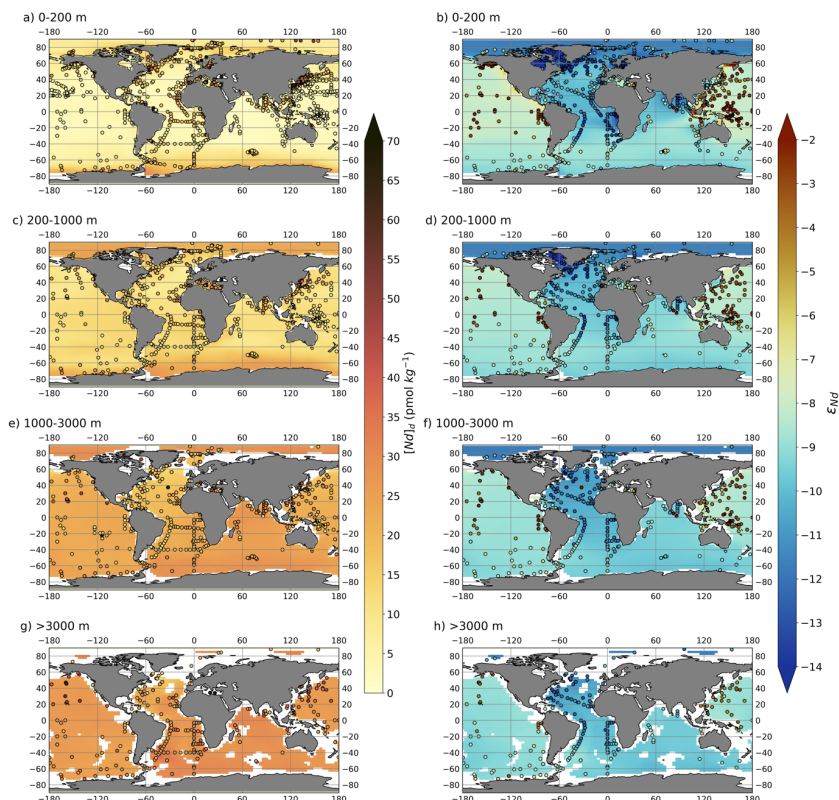
Figure 14: Maps of [Nd]_d (left) and \epsilon_{Nd} (right) in simulation EXPT_SED2 split into four different depth bins, (a-b) shallow (0-200 m), (c-d) intermediate (200-1,000 m), (e-f) deep (1,000-3,000 m), and (g-h) deep abyssal ocean (>3,000 m). Water column measurements from within each depth bin (Osborne et al., 2017, 2015; GEOTRACES Intermediate Data Product Group, 2021) are superimposed as filled circles using the same colour scale.
