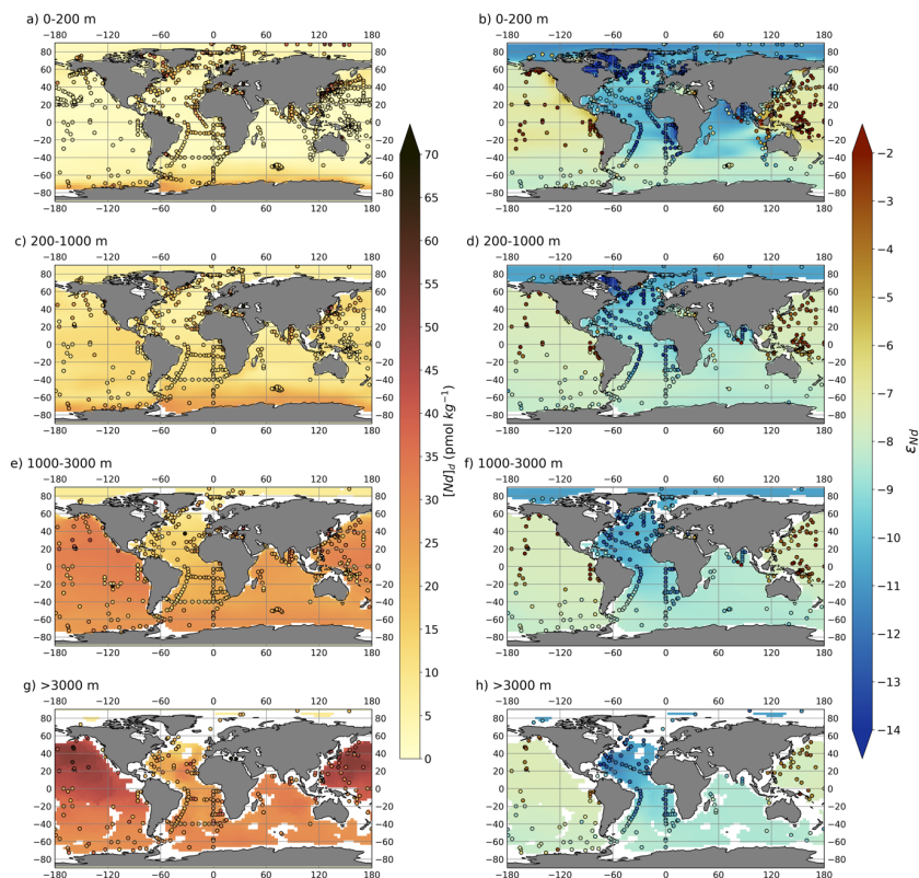
Figure 10: Maps of [Nd]_d (left) and \epsilon_{Nd} (right) in simulation EXPT_RS4 split into four different depth bins, (a-b) shallow (0-200 m), (c-d) intermediate (200-1,000 m), (e-f) deep (1,000-3,000 m), and (g-h) deep abyssal ocean (>3,000 m). Water column measurements from within each depth bin (Osborne et al., 2017, 2015; GEOTRACES Intermediate Data Product Group, 2021) are superimposed as filled circles using the same colour scale.
