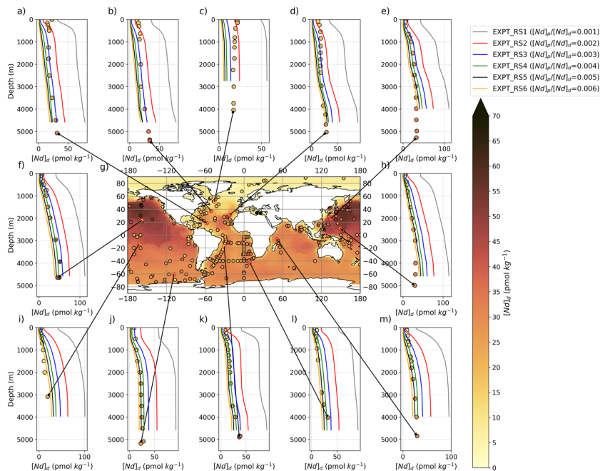
Figure 11: Central panel (g) displays [Nd]_d at the seafloor (i.e., lowermost box of the ocean model), in simulation EXPT_RS4 (100-year mean from the end of the run), with superimposed water column measurements (Osborne et al., 2017, 2015; GEOTRACES Intermediate Data Product Group, 2021) from \geq 3,000 m shown by filled coloured circles on the same colour scale. Surrounding panels (a-f) and (h-m) display depth profiles of simulated (coloured lines, one per sensitivity simulation with varied [Nd]_p/[Nd]_d ) and measured (filled circles) [Nd]_d . Larger shifts in the [Nd]_d between simulations highlight regions most sensitive to the efficiency of reversible scavenging.
