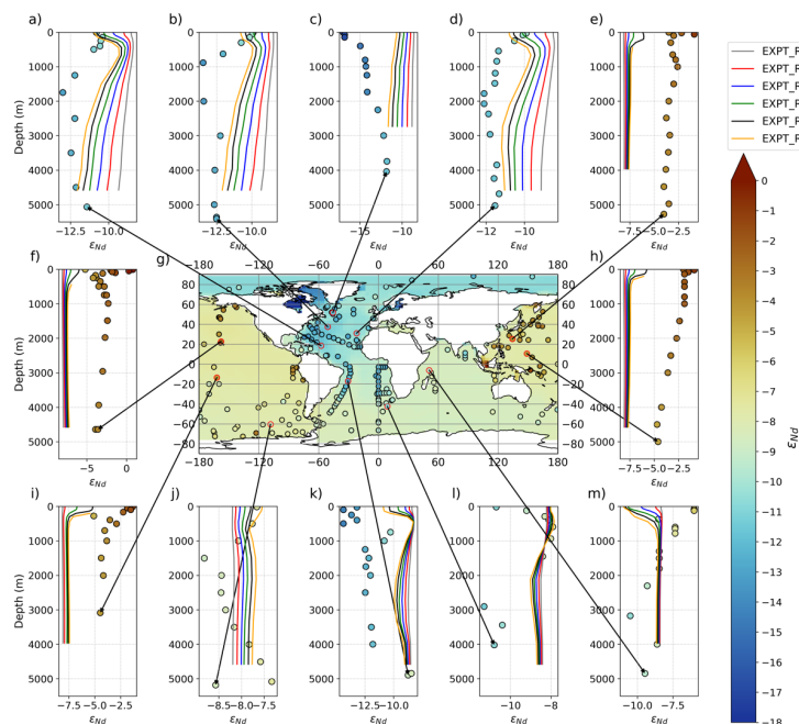
Figure 12: Central panel (g) displays \epsilon_{Nd} at the seafloor (i.e., lowermost box of the ocean model), in simulation EXPT_RS4 (100-year mean from the end of the run), with superimposed water column measurements (Osborne et al., 2017, 2015; GEOTRACES Intermediate Data Product Group, 2021) from \geq 3,000 m shown by filled coloured circles on the same colour scale. Surrounding panels (a-f) and (h-m) display depth profiles of simulated (coloured lines, one per sensitivity simulation with varied [Nd]_p/[Nd]_d ) and measured (filled circles) \epsilon_{Nd} . Larger shifts in the \epsilon_{Nd} between simulations highlight regions most sensitive to the efficiency of reversible scavenging.
