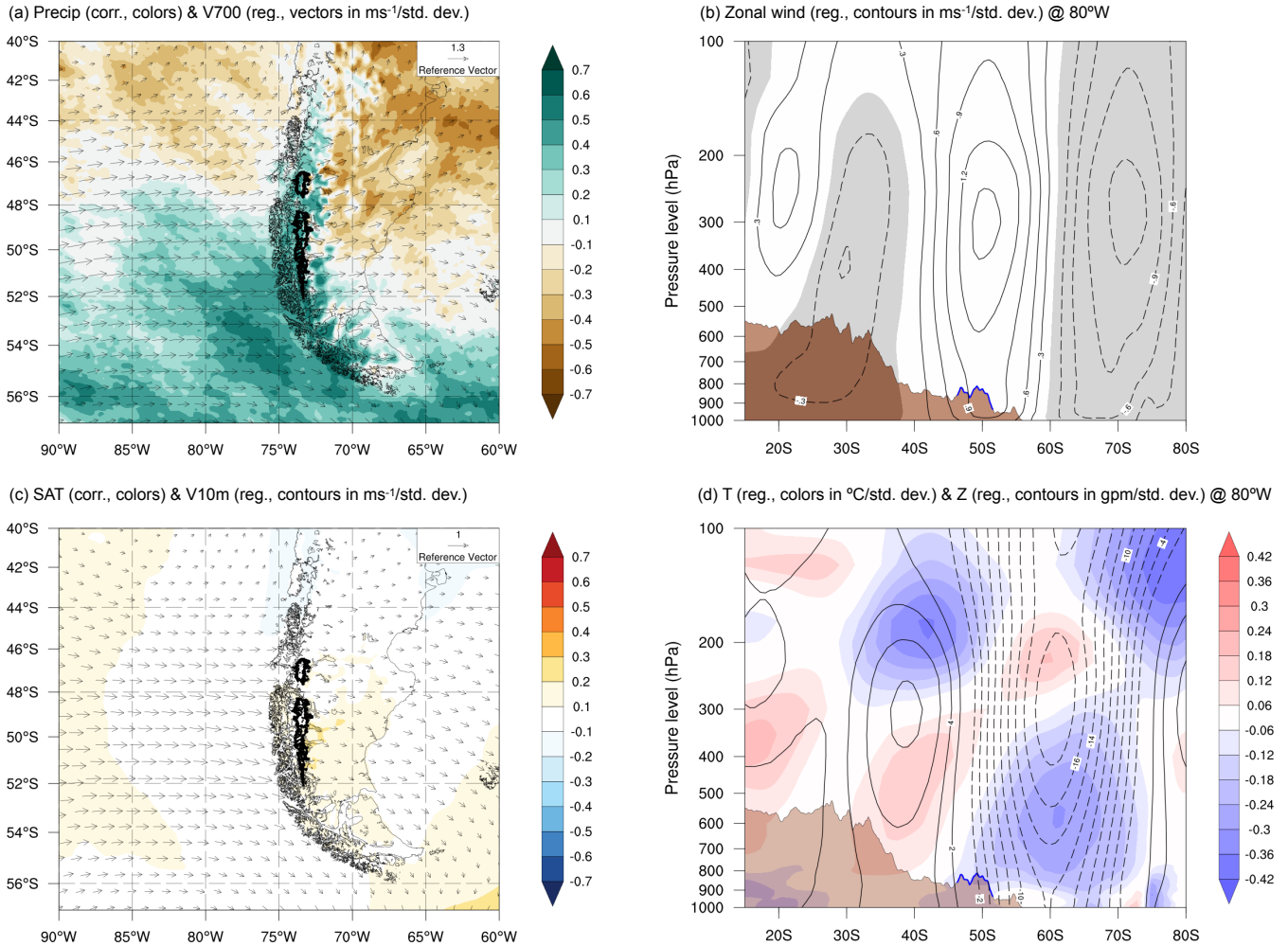
Figure 6. The same as in Fig. 5 but for the winter (April to September).
