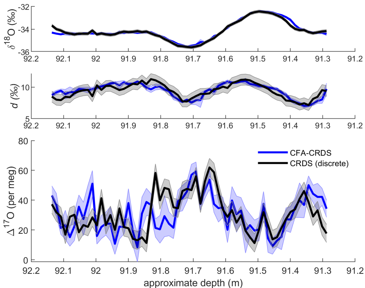
640 Figure 4: Comparison of discrete CRDS ice core measurements (black) with calibrated CFA-CRDS data averaged over 1.39-cm intervals (blue). Corresponding \delta^{18}\text{O} and d data are shown for seasonal context. Discrete CRDS measurements are shown with the root mean square error of corresponding reference water measurements (grey shading), and CFA-CRDS measurements are shown as the mean of nine measurements with the standard error (blue shading). Note that \delta^{18}\text{O} and d are reported in ‰ and that \Delta^{17}\text{O} is measured in per meg; each vertical axis uses different scaling.
