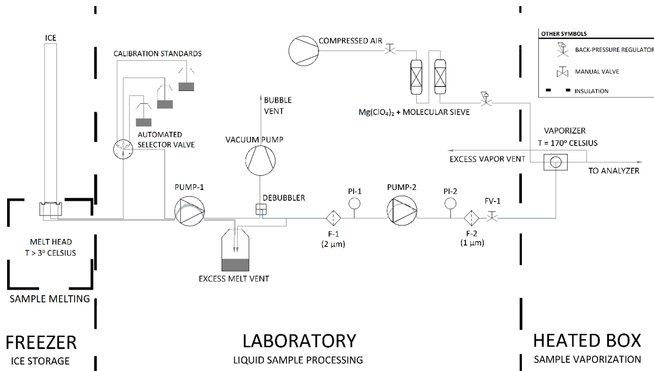
620 Figure 1: Process flow diagram for our CFA system. Thick dashed lines indicate transitions between temperature-controlled process spaces. Note that F-1 and F-2 are filters, PI-1 and PI-2 are pressure sensors, and FV-1 is a flow valve.
