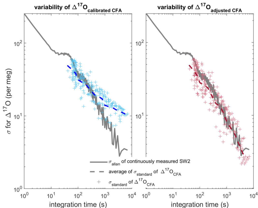
660 Figure 7: Comparison of Allan deviation of continuous reference water measurements and standard deviation of nine duplicate CFA ice core measurements. In both left and right images, the Allan deviation line (solid grey) for a long measurement of SW2 is overlain by the standard deviation of the CFA-CRDS ice core measurements (crosses) and the mean of the standard deviations for each integration time (dashed line). The \Delta^{17}\text{O}_{\text{calibrated CFA}} and \Delta^{17}\text{O}_{\text{adjusted CFA}} data are shown in blue and red similarly to Figs. 5 and 6. The standard deviation on the left is calculated from calibrated replicate CFA-CRDS measurements and shows the total variability between CFA-CRDS replications along the depth of the core. The standard deviation information in the right plot is calculated from 665 calibration-adjusted datasets so that the effect of the calibration offset error is removed; this analysis is still dependent upon instrumental noise, CFA errors, depth registration errors, and natural variability within the core.
