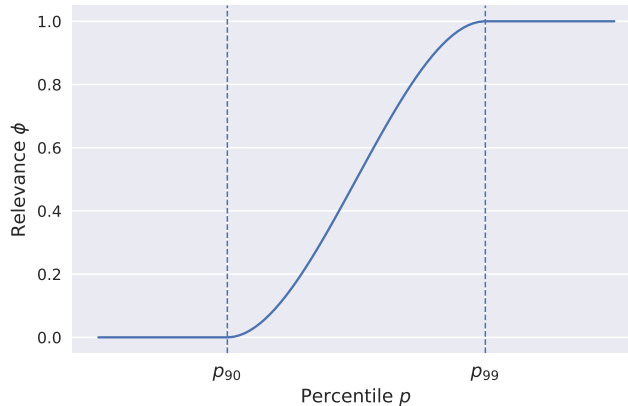
Figure 5. The relevance function \phi obtained by interpolating the 90 th percentile ( p_{90} ) as control-point of minimum relevance and the 99 th percentile ( p_{99} ) as control-point of maximum relevance, using the pchip interpolation algorithm of Ribeiro and Moniz (2020).
