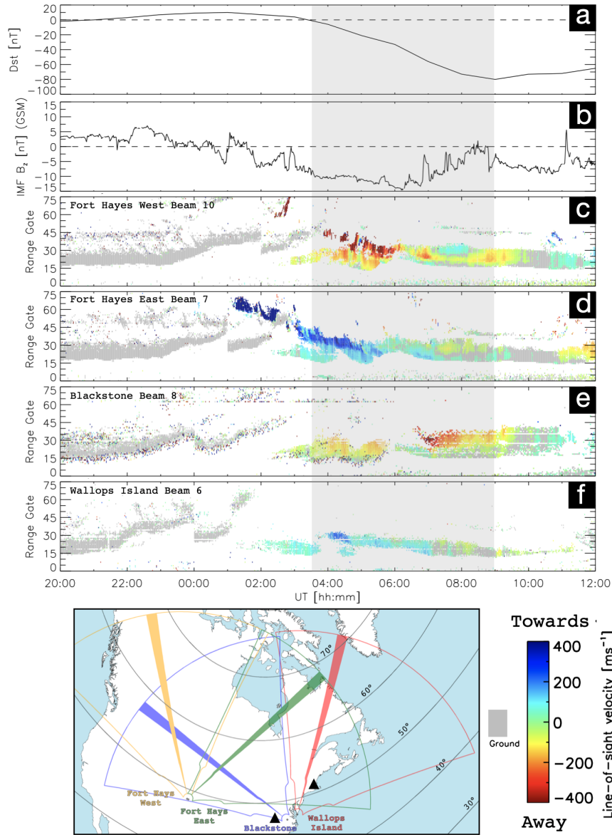
Figure 2. SAPS event overview, starting at the 20:00 on November 8th and ending at 12:00 November 9th, 2013. [a] Disturbance storm time (Dst) index. [b]: IMF B_z in geocentric solar magnetospheric coordinates (GSM). [c,d,e,f]: Range-time plots of the LOS plasma velocity from beams 10, 7, 8 and 6 of the Fort Hayes West, Fort Hayes East, Blackstone and Wallops Island SuperDARN radars, respectively. Blue indicates plasma moving towards the radar site, whilst red means away. Grey indicates data that has been flagged as ground scatter. The diagram at the bottom shows the orientations of the chosen beams for [c,d,e,f]. The grey shaded region is the geomagnetic storm “main phase”, as dictated by the Dst index.
