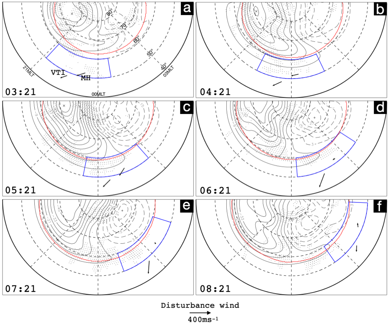
Figure 5. Polar plots in the same format as Figure 4, except with the SuperDARN global fitted electric potential contours (in kV) instead of the radar LOS data. Black dots are the locations of SuperDARN radar LOS data which contributed to the fit. The blue box is the region over which the fitted plasma velocity was averaged for the purpose of cross-correlation, results of which are shown in Figure 6.
