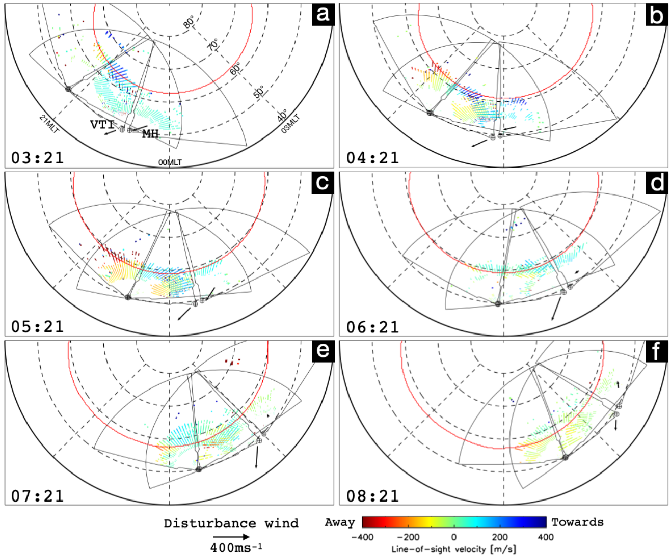
Figure 4. Nightside polar plots of plasma velocity data from four SuperDARN radars, as well as disturbance neutral wind velocity vectors from the VTI and MH FPIs (black arrows) for times on November 9th, 2013. The red circle is the approximate location of the auroral oval lower-latitude boundary, derived from SSUSI data onboard whichever DMSP satellite (F-16, F-17 or F18) last crossed the pole. Six times are shown 1 hour apart each, the coordinate system is AACGM latitude-magnetic local time and the concentric dashed lines separate 10^\circ of latitude. Data in each SuperDARN radar beam has been made thinner to help show which radar it was measured by, and thus the LOS direction. The VTI FPI is the arrow with a base at a slightly lower latitude, compared to the MH FPI.
