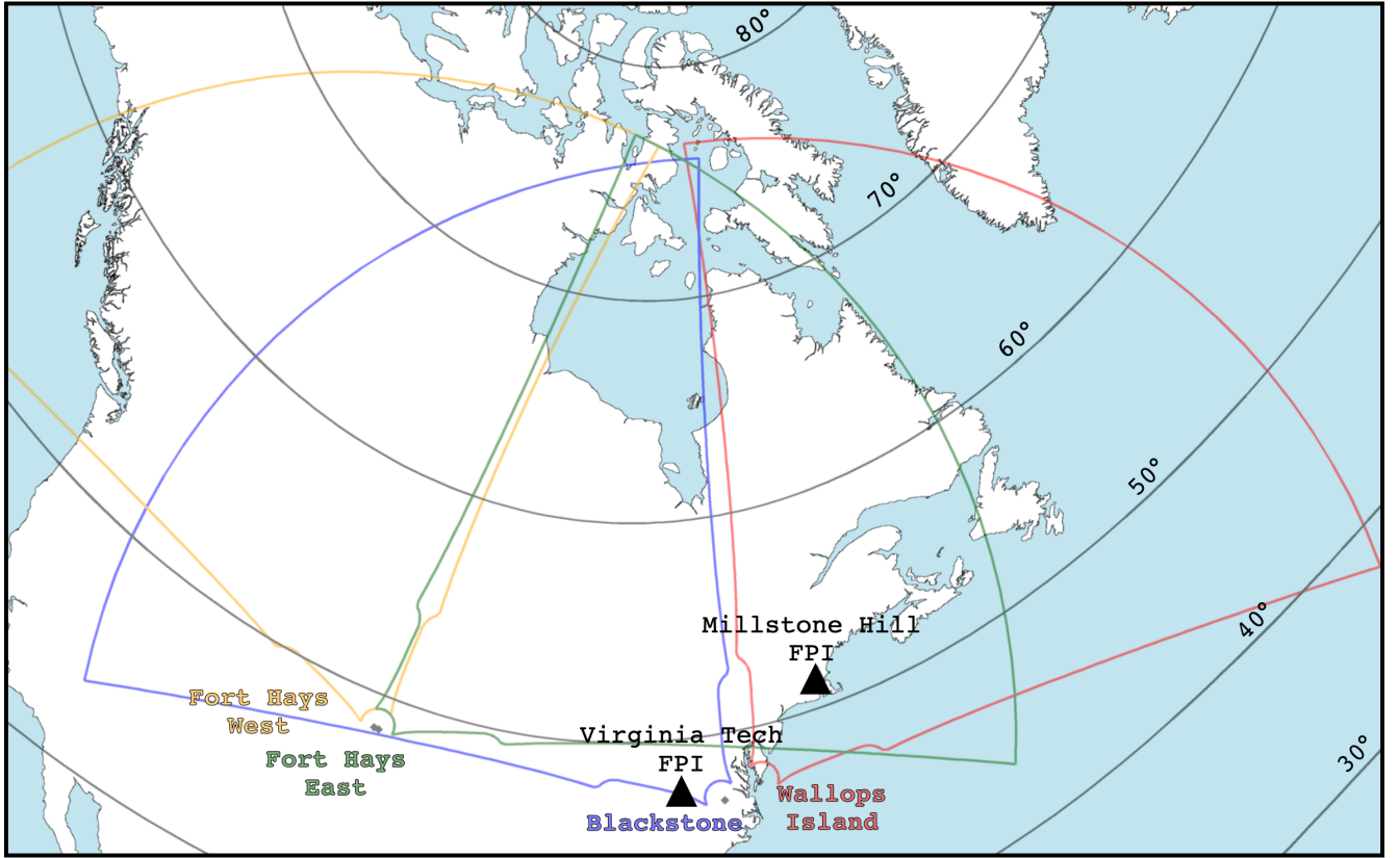
Figure 1. The fields of view of the Fort Hays West, Fort Hays East, Blackstone and Wallops Island SuperDARN radars, up to range gate 75 (each gate being 45 km wide). Also shown are the locations of two FPIs (black triangles), one at Millstone Hill Geospace Facility and the other at Virginia Tech (November 2013). Black lines indicate parallels of constant AACGM latitude.
