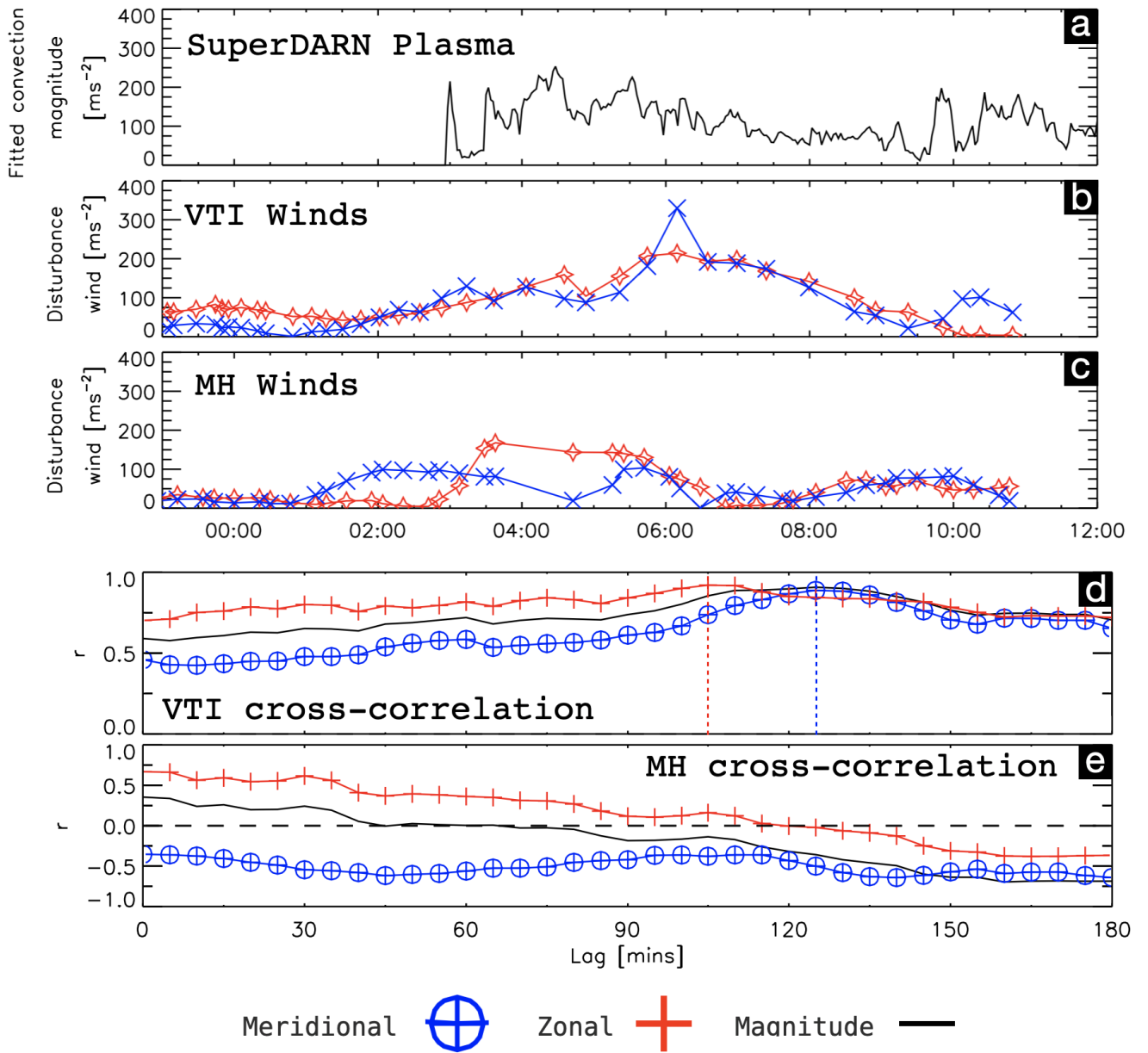
Figure 6. [a]-[c]: Timeseries used in the cross-correlation for the [a] Average fitted convection magnitude within the blue box region in Figure 5, [b] VTI disturbance winds and [c] MH disturbance winds. [d] and [e]: Cross-correlation results from the meridional, zonal and magnitude disturbance winds from [d] VTI and [e] MH. Winds are lagged backwards up to 180 minutes in 5-minute steps, against the plasma velocities shown in [a]. Vertical dashed lines in [d] indicate the lags with the highest r -values for the meridional and zonal components.
