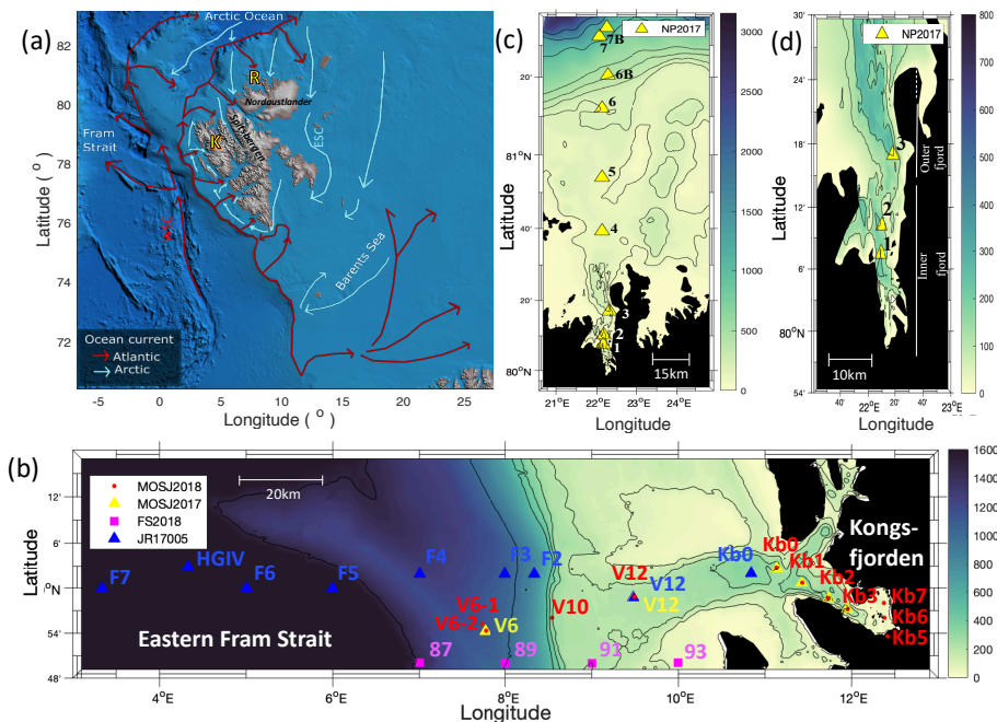
Figure 1. Maps of the Norwegian archipelago of Svalbard, including close-ups of the two study fjords, Kongsfjorden and Rijpfjorden with an indication of sampling sites. In (a), Atlantic and Arctic Water currents are depicted in red and blue, respectively. K denotes Kongsfjorden; R denotes Rijpfjorden, WSC, West Spitsbergen Current; ESC, East Spitsbergen Current. This subplot is based on Hop et al. (2019), Eriksen et al. (2018) and Leifer et al. (2018) and was designed using Global Mapper software (v.20.0, 2018), bathymetry data from IBCAO v.3 by Jakobsson et al. (2012). In (b), the bathymetric map of Kongsfjorden, Svalbard, and the eastern side of Fram Strait, illustrates sampling sites of the Norwegian Polar Institute Monitoring Cruises (2017, yellow triangles; 2018, red dots) for \delta^{15}\text{N-NO}_3^- and \delta^{18}\text{O-NO}_3^- determination. Samples were taken in the fjord (Kb0-3,5-7), as well as on the shelf (V12) and continental slope (V10 and V6). Data from sampling sites of FS2018 (pink squares) and JR17005 (blue triangles) cruises were also used for better coverage of offshore conditions. Shipboard measurements from cruise JR17005 were taken from the RSS James Clark Ross as part of the UK Changing Arctic Oceans programme in May-June 2018. Cruise FS2018 took place on the R.V Kronprins Haakon as part of the Fram Strait Arctic Outflow Observatory in August-September 2018. Colour coding corresponds to depth in metres. In (c) and (d), the bathymetric map of Rijpfjorden, Svalbard, illustrates sampling sites of the Norwegian Polar Institute monitoring cruises (NP2017, yellow triangles) for \delta^{15}\text{N-NO}_3^- and \delta^{18}\text{O-NO}_3^- determination. In (c) all sample locations are shown, namely in the inner fjord (R1-2), outer fjord (R3) as well as on the shelf (R4-R5) and continental slope (R6-R7B). In (d) a zoom-in map of inner and outer fjord region is shown. Colour coding corresponds to depth in metres.
