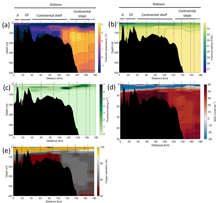
Figure 4. Cross-sections across Rijpfjorden of (a) potential temperature ( ^{\circ}\text{C} ); (b) salinity (PSU); (c) fluorescence ( \text{mg m}^{-3} ), (d) apparent oxygen utilisation (AOU, \mu\text{mol kg}^{-1} ), (e) oxygen saturation (%). Data from CTD casts from NP2017 cruise. Grey vertical lines indicate the individual CTD casts where water samples were collected for isotopic analysis, with sampling depths indicated by the black dots and station number indicated above each line. Distance is shown as cumulative distance between successive stations. 'If', inner fjord; 'Of', outer fjord.
