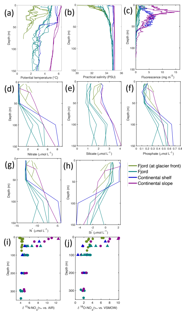
Figure 5. Depth profiles of (a) Temperature (°C), (b) salinity (PSU), (c) fluorescence (mg L -1 ), (d) nitrate (μmol L -1 ), (e) silicate (μmol L -1 ), (f) phosphate (μmol L -1 ), (g) N* (μmol L -1 ), (h) Si* (μmol L -1 ), (i) δ 15 N-NO 3 - (‰) and (j) δ 18 O-NO 3 - (‰) from Kongsfjorden using NP2018 (circles and solid lines) and NP2017 (triangles) cruise samples. Colour denotes locations in Kongsfjorden at glacier fronts, fjord, continental shelf and slope. Note: Standard deviations of the isotopic values reported in (i) and (j) are 0.33 and 0.47 ‰ for δ 15 N and δ 18 O, respectively.
