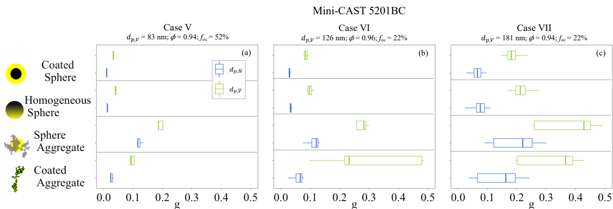
730 Figure 11. The asymmetry parameter g is modelled using the four representations of coated BC i.e., ‘coated sphere’, ‘homogeneously mixed sphere’, ‘coated aggregate’, and ‘aggregate and sphere’. For each representation, the g is modelled using monodisperse particles (with d_{p,\bar{N}} and d_{p,\bar{V}} ). The results are shown for E2 cases V – VII: mini-CAST 5201BC d_{p,\bar{V}} = 83 nm (a); mini-CAST 5201BC d_{p,\bar{V}} = 126 nm (b); and mini-CAST 5201BC d_{p,\bar{V}} = 181 nm (c).
