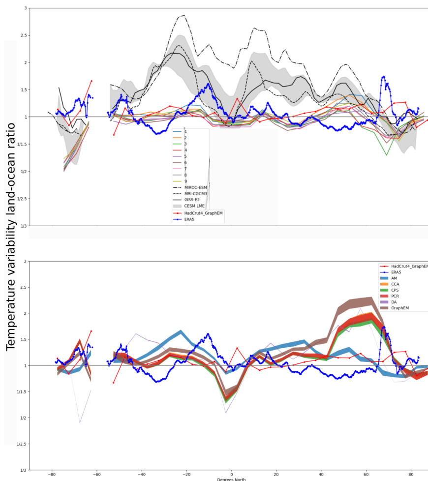
Figure 7. Zonally averaged contrast in land-ocean temperature variability as a function of latitude over the observational period (>1850). Atmospheric 2-m temperatures over the oceans are used to calculate ocean temperature variability. Results are shown for the 9-members perturbed-parameter i LOVECLIM ensemble (numbers 1 to 9 in top panel), for four different CMIP5 last millennium simulations (top panel) and the results for the six different CFR methods (lower panel). For comparison, in both panels results are shown for the ERA5 and HadCrut4 observational data sets. Note that the ERA5 data-set covers only the period 1979 to 2019. Grey (colored) shading in the top (lower) panel shows the 1-sigma range of all CESM (CFR) ensemble members. Note that the y-axis scale in the right-hand panel is non-linear with for instance 1/1.5 or 1/2 meaning that there is 50% or 100% more variability over the ocean than there is over the continents.
