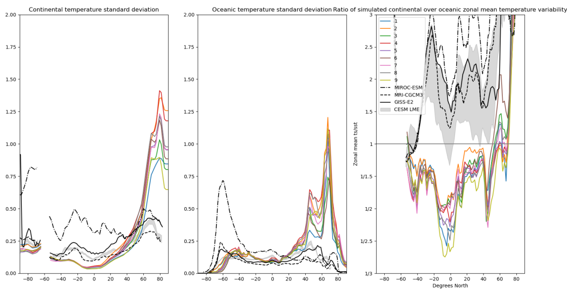
Figure A8. Simulated zonally averaged contrast in land-ocean temperature variability as a function of latitude. Depicted are continental variability (left-hand column), ocean variability (middle column) and the ratio of continental over ocean variability (right-hand-column). SSTs are used to calculate ocean temperature variability. Results are shown for the 9-members perturbed-parameter i LOVECLIM ensemble (colors) and for three different CMIP5 simulations for the last 1000 years. Grey shading shows the 1-sigma range of all CESM ensemble members. Note that the y-axis scale in the right-hand panel is non-linear with for instance 1/1.5 or 1/2 meaning that there is 50% or 100% more variability over the ocean than there is over the continents.
