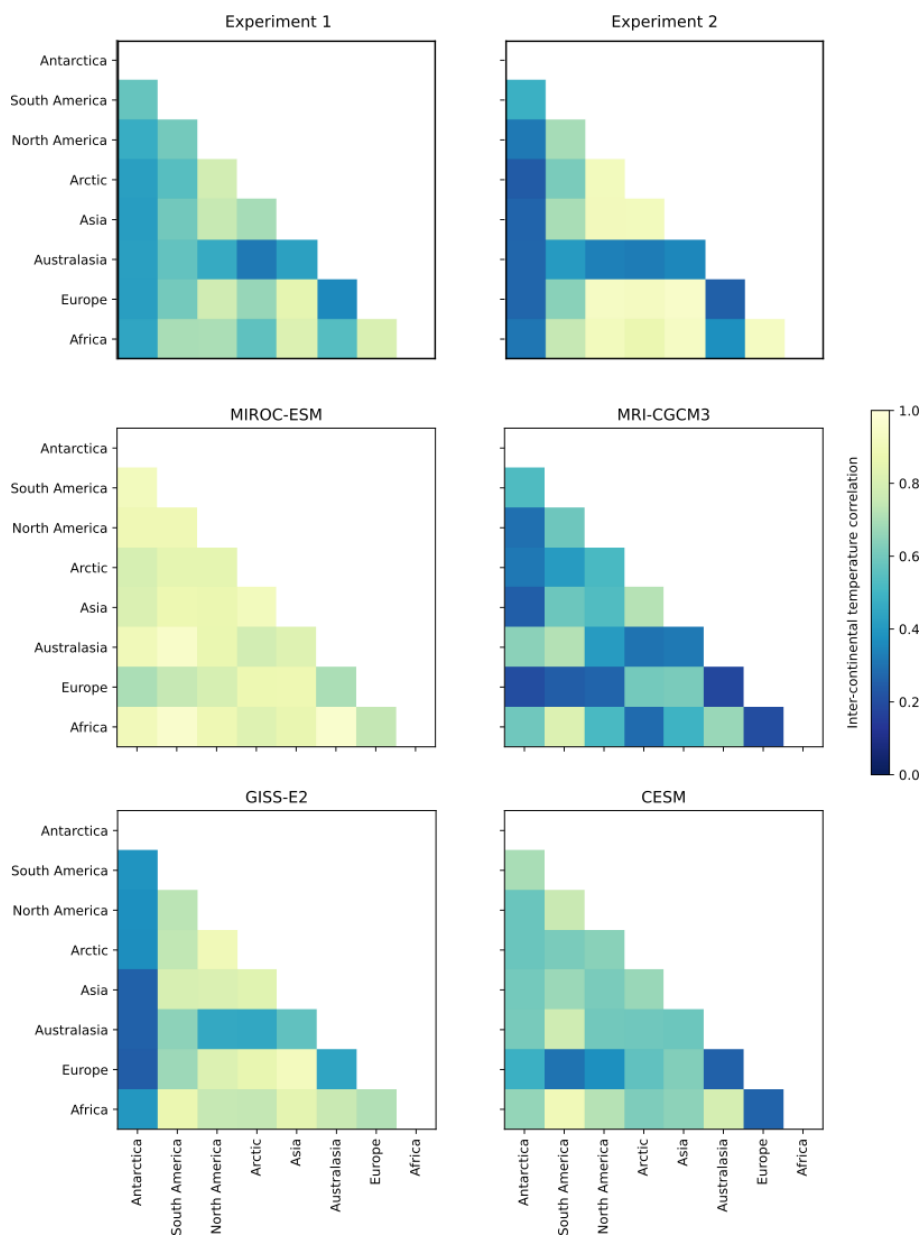
Figure 5. Inter-continental temperature correlations for i LOVECLIM ensemble members 1 and 2, and for the CMIP5 last millennium simulations. For the CESM results ensemble mean values were first calculated per grid cell before calculating the inter-continental correlations. The i LOVECLIM results shown here are lagged correlations. See Figure A2 for the results of all i LOVECLIM ensemble members and see Figure A3 for the non-lagged correlations.
