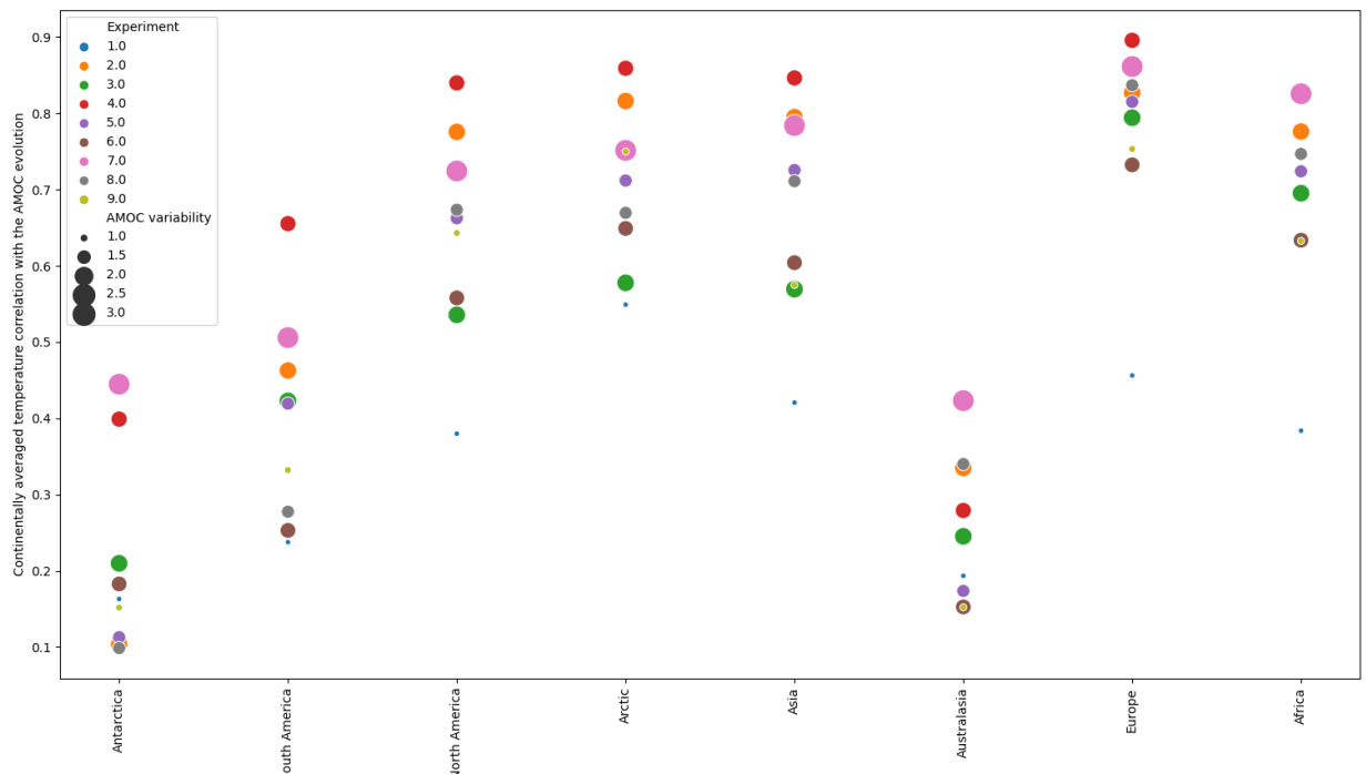
Figure 2. Correlation of regional temperature time-series with AMOC evolution in the iLOVECLIM ensemble. The different experiments are shown in colors and the amount of AMOC variability ( S_v ) in the different experiment by the marker size. These results are lagged correlations per continental time serie.
