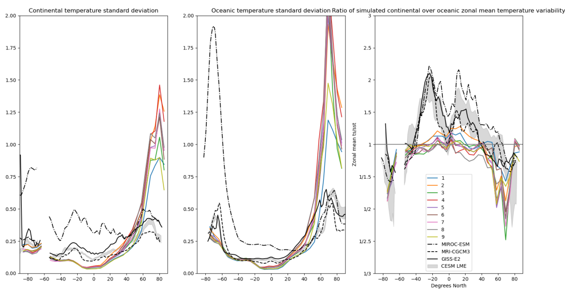
Figure A7. Simulated zonally averaged contrast in land-ocean temperature variability as a function of latitude. Depicted are continental variability (left-hand column), ocean variability (middle column) and the ratio of continental over ocean variability (right-hand-column). Atmospheric 2-m temperatures over the oceans are used to calculate simulated ocean temperature variability. Results are shown for the 9-members perturbed-parameter iLOVECLIM ensemble (colors) and for three different CMIP5 simulations for the last 1000 years. Grey shading shows the 1-sigma range of all CESM ensemble members. Note that the y-axis scale in the right-hand panel is non-linear with for instance 1/1.5 or 1/2 meaning that there is 50% or 100% more variability over the ocean than there is over the continents.
