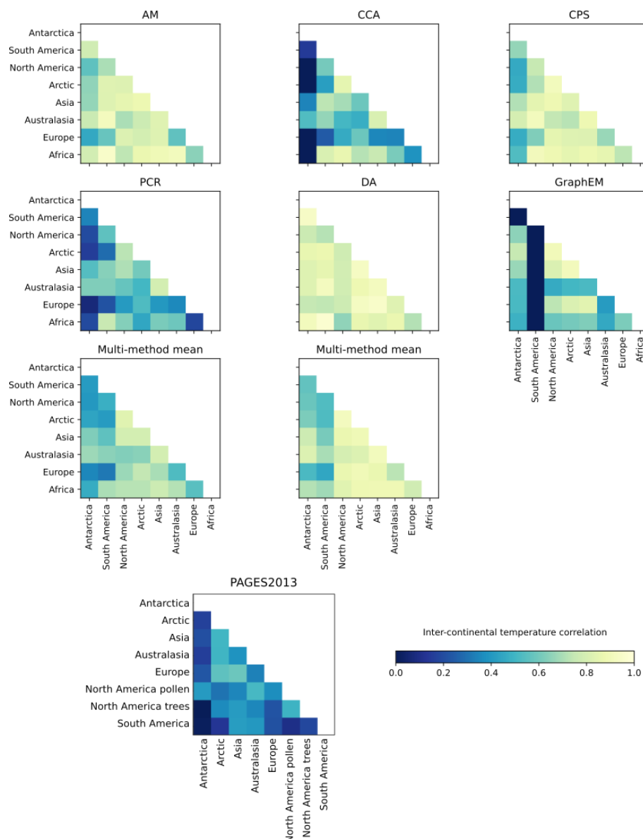
Figure 6. Reconstruction based inter-regional temperature correlations. Shown are the PAGES-2K results for the individual CFR methods (Neukom et al., 2019), two different ways to calculate the multi-method-multi-ensemble-mean, and the results based on the original PAGES-2K temperature time series (Ahmed et al., 2013). The top six panels show the results in which individual inter-regional temperature correlations are calculated for every ensemble member, after which the results are averaged for a single CFR. The multi-method-mean of those results is shown on the left of the third row. Another method is to calculate ensemble mean temperature time series for every grid cell, then regional averages and finally calculate inter-regional temperature correlations. The corresponding multi-method-mean is shown here in the middle of the third row while the corresponding results for the individual CFRs are shown in Figure A4. Note that these results are non-lagged correlations and that for the he results based on the original PAGES-2K temperature time series partially different continental-scale regions are shown.
