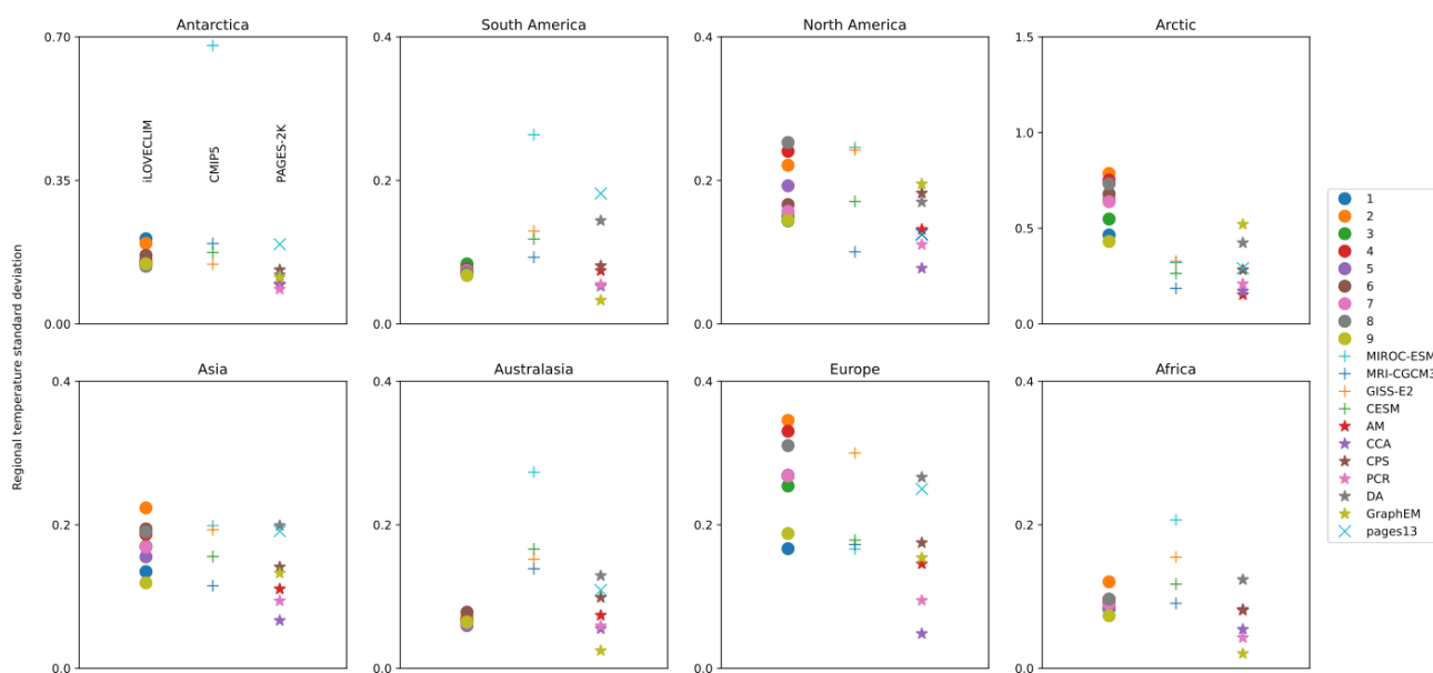
Figure 1. Temperature variability (standard deviation in K) for different continental regions. Shown are the nine iLOVECLIM ensemble members (left), results for the CMIP5 simulations (middle), ensemble means for the six different CFR-based results from the PAGES-2K data-set (right; Neukom et al., 2019) and the temperature variability based on the original PAGES-2K time-series (Ahmed et al., 2013) for the continental-scale regions for which this data is available. For North America, both the pollen-based and tree-based results are shown. For the CESM results we show the mean of the standard deviation over the ensemble. Note the different y-axis. A 50-year butterworth filter was applied to all results except for the original PAGES-2K time-series which are 30-year averages.
