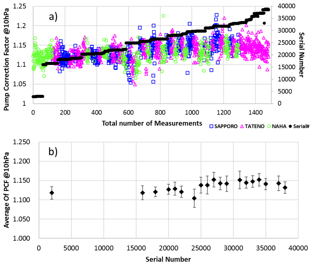
Figure 15: a): Pump correction factors at 10 hPa from 2009 to 2022 sorted by ozone sensor serial number. b): The same averaged for each bin of 1000 of ozonesonde serial numbers for 2009 - 2022. Error bars represent standard deviation.
