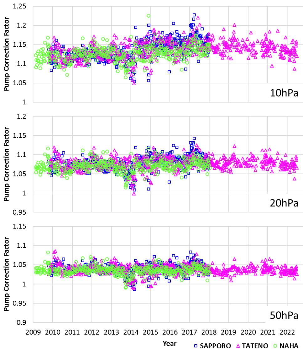
370 Figure 14: Pump correction factors for 2009 - 2022 (top to bottom: 10, 20 and 50 hPa). Over this 11 year period, the factor has changed by + 1% at 50hPa, + 2% at 20hPa and + 4% at 10hPa.
