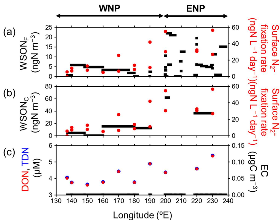
Figure 5: Longitudinal distributions of mass concentrations of (a) WSON_F (black) and (b) WSON_C (black), together with N_2 -fixation rate in the SSW samples (red solid circle), (c) DON (red solid circle) and TDN (blue solid circle) concentrations in surface seawater and aerosol EC concentrations (black) during the entire cruise.
