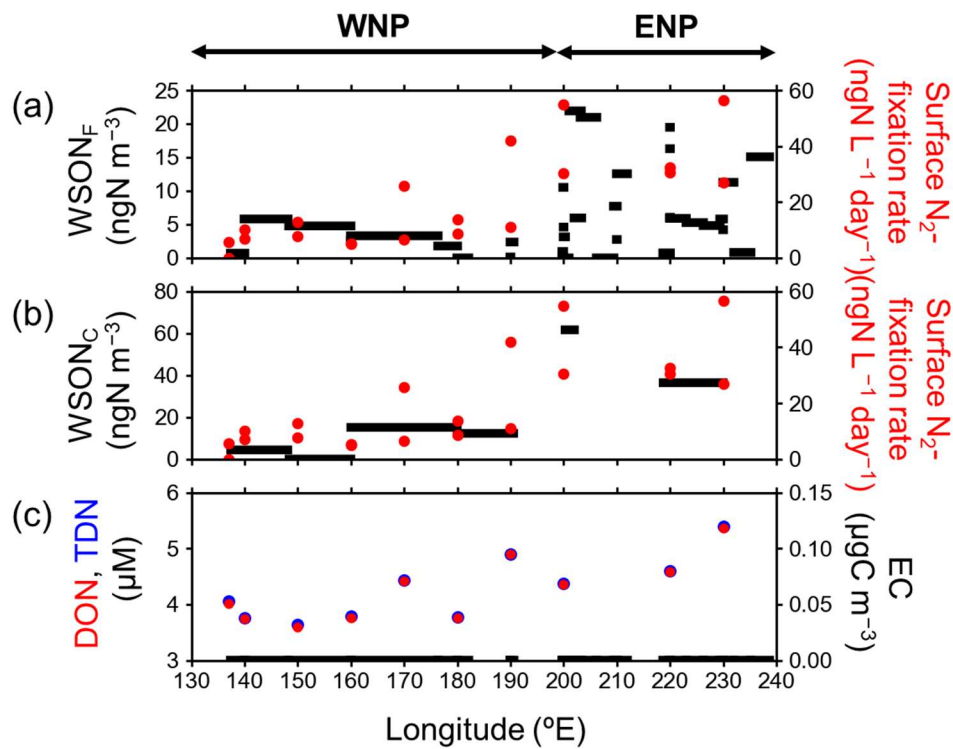
Revised Figure 5: Longitudinal distributions of mass concentrations of (a) WSON F (black) and (b) WSON C (black), together with \text{N}_2 -fixation rate in the SSW samples (red solid circle), (c) DON (red solid circle) and TDN (blue solid circle) concentrations in surface seawater and aerosol EC concentrations (black) during the entire cruise.
