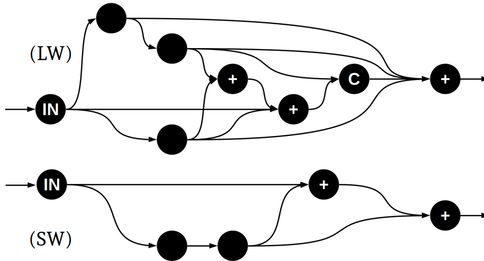
Figure 3. Wiring patterns of the three-two (longwave and shortwave) randomly generated neural networks that were selected for use in the optics emulator. Nodes represent “dense” (fully connected) layers. “C” and “+” indicate whether inbound tensors are combined by concatenation or addition. All hidden layers have the same number of neurons within each network: SW: 26, LW1: 1754, LW2LW: 2532 (the nine inputs are padded to reach the appropriate size and the output layer has either 3 (SW) or 1 (LW) neurons).
