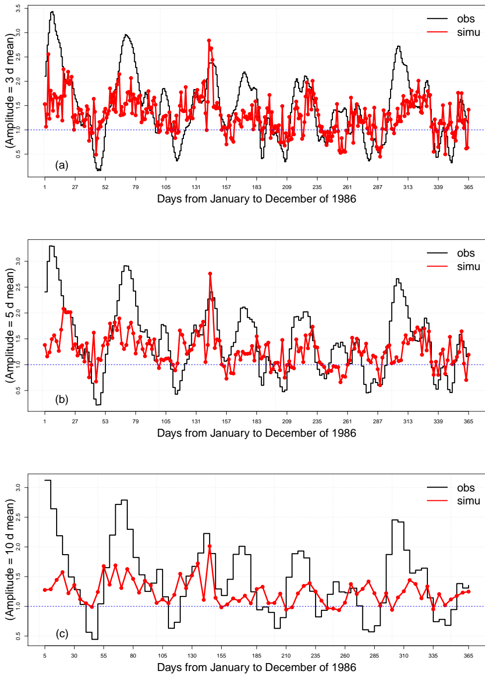
Figure A3. Time series of observations and simulations of the MJO Amplitude computed from analogs of OLR, for lead time of 3, 5 and 10 days, respectively (a), (b) and (c), for the year 1986. The red line represents the mean of the 100 simulations, the black line represents the observations, and the blue line indicates the threshold of the MJO activity A(t) \geq 1 .
