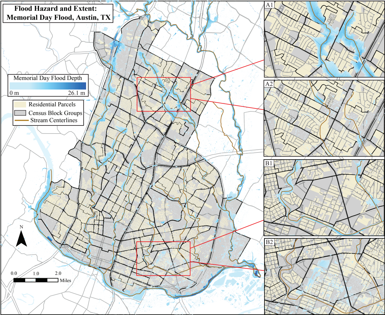
Figure 4. Fluvial and Pluvial flood depths and extent in Austin, Texas during the 2015 Memorial Day flood. Insets A1 and B1 show only the fluvial inundation component, while insets A2 and B2 show only the pluvial inundation component of the flood event.
