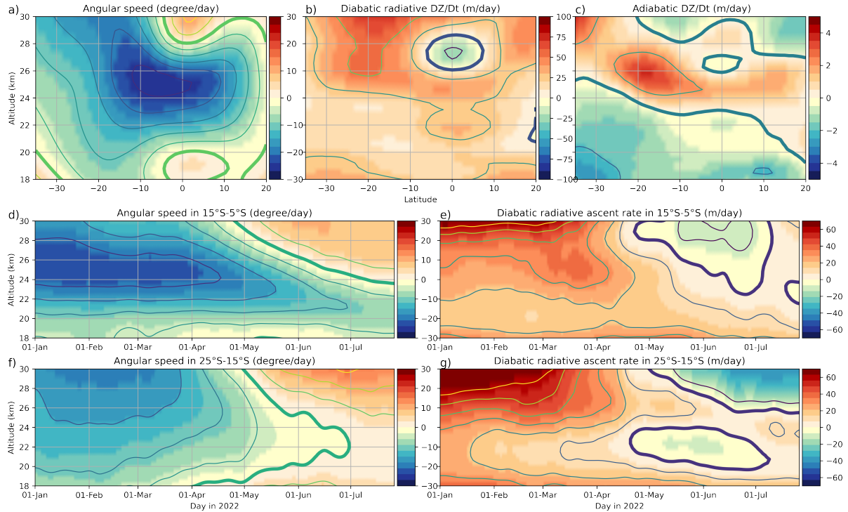
Figure A1. (a) Zonal mean angular rotation speed \omega = \frac{U}{R_{\text{Earth}} \cos(\phi)} from ERA5 averaged between 15 January 2022 and 15 March 2022 (in degree day -1 ). (b) Same for the diabatic ascent calculated from the total all-sky ERA5 heating rate (in m day -1 ). (c) Same for the adiabatic ascent due to motion of the isentropic surfaces with respect to the geopotential surfaces (in m day -1 ). (d) Daily zonal and altitude band average angular speed between 15°S and 5°S as a function of time (in degree day -1 ). (e) Same as d) for the diabatic ascent (in m day -1 ). (f-g) same as d-e) for the latitude band between 25°S and 15°S.
