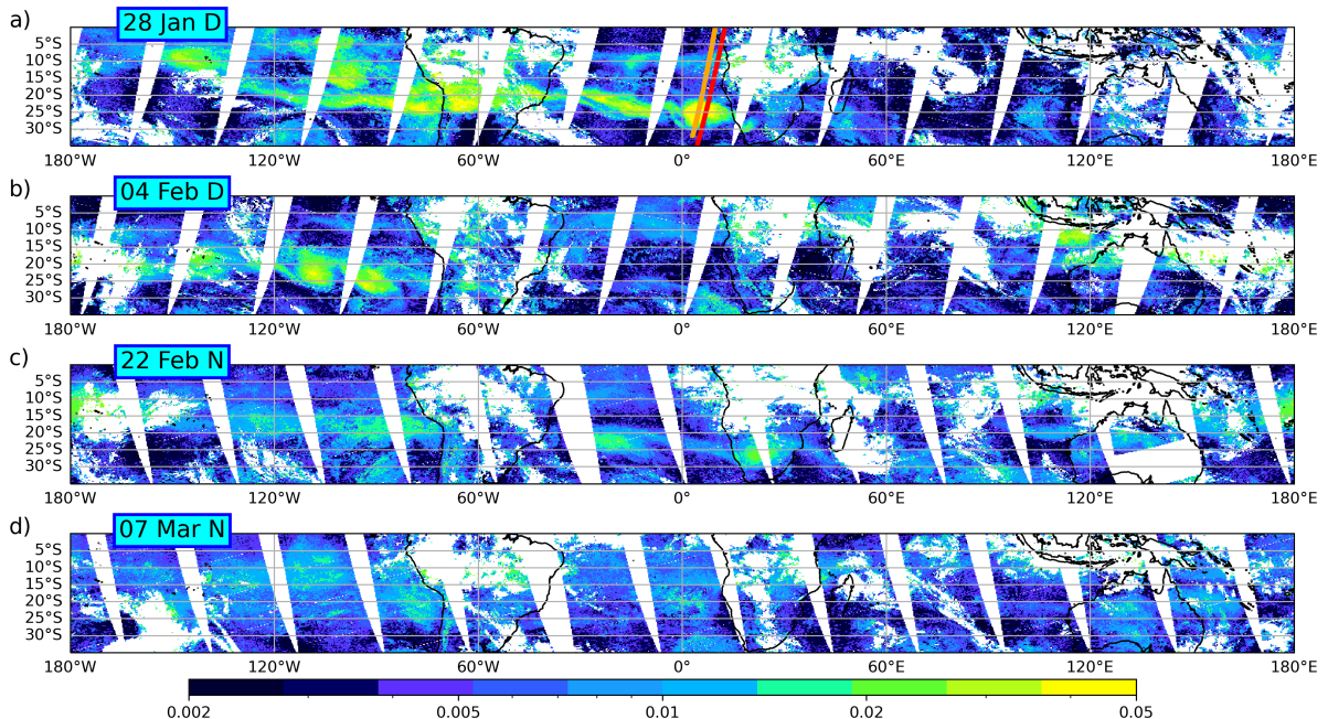
Figure 5. SA/OD from IMS in the latitude range 0°-35°S at four different dates as indicated. Panels (a-b) are drawn for day swaths whereas panels (c-d) are drawn for night swaths. The time progresses from right to left and the interval between two adjacent swaths is 1h52.
