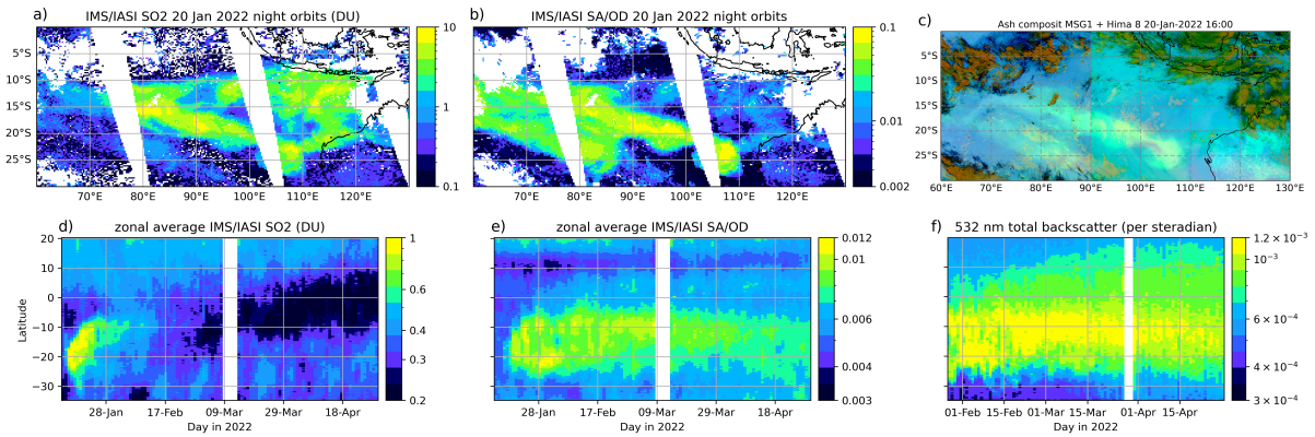
Figure 4. (a-b) SA/OD and SO 2 from IMS on 20 January 2022 for three night orbits crossing equator at 14:06 UTC (right swath), 15:48 UTC (middle swath) and 17:29 UTC (left swath). (c) RGB-Ash composite from Meteosat-8 and Himawari-8 at 16:00 UTC on the same day. (d-e) Zonal average SA/OD and SO 2 from 13 January 2022 to 30 April 2022. (f) CALIOP 532 nm attenuated backscatter integrated between 18 and 30 km from 27 January 2022 to 30 April 2022 (per steradian).
