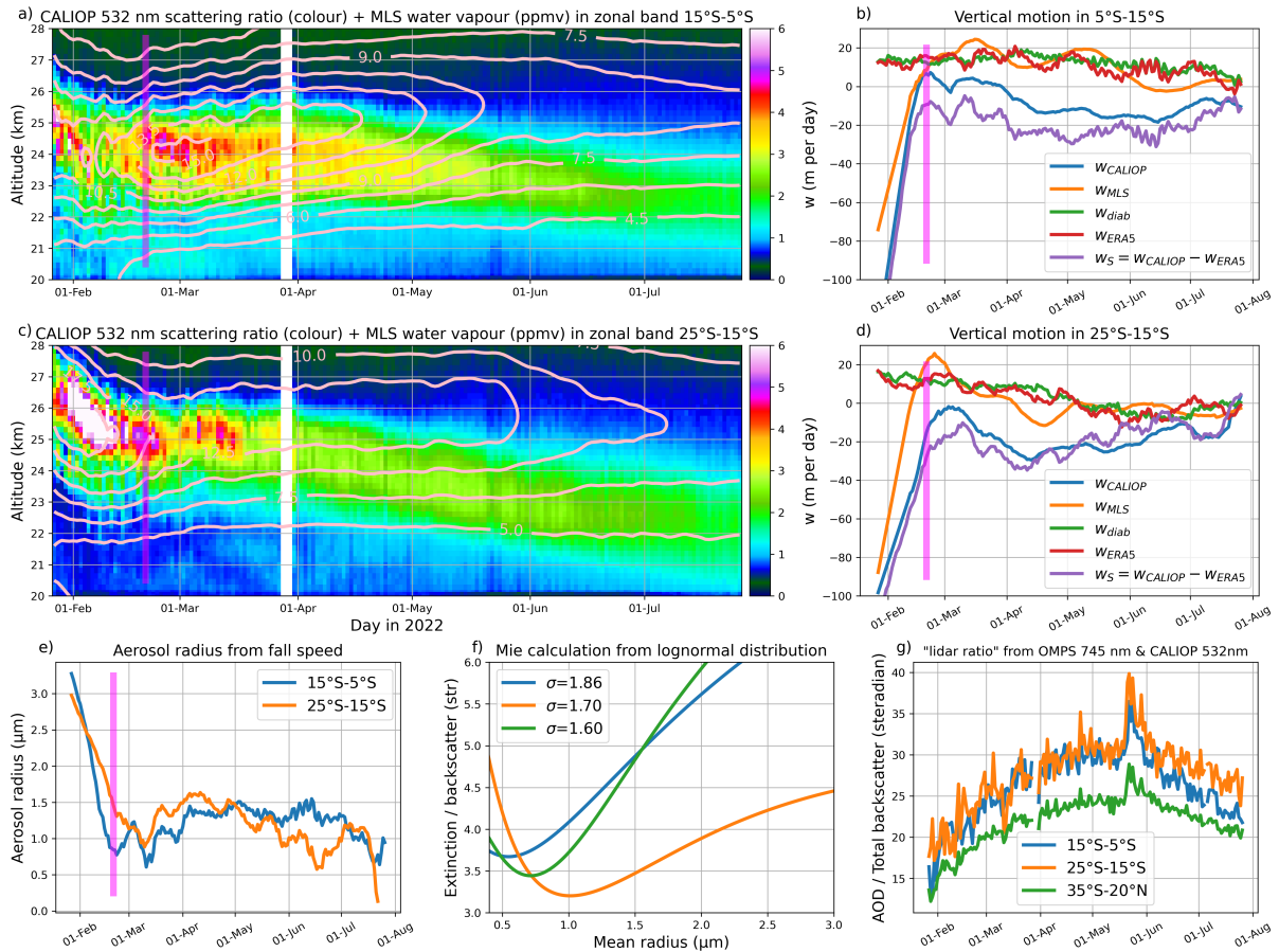
Figure 2. (a) and (c) Zonal and latitude band averages as a function of time for CALIOP 532 nm scattering ratio (colour) and MLS water vapour (contours, ppmv) for, respectively 15^{\circ}\text{S}-5^{\circ}\text{S} and 25^{\circ}\text{S}-15^{\circ}\text{S} latitude bands. (b) and (d) Vertical motions for the same two latitude bands: W_{\text{CALIOP}} for aerosol plume and W_{\text{MLS}} for water vapour plume deduced from a) and c), W_{\text{diab}} and W_{\text{ERA5}} for ERA5 diabatic and total (diabatic + adiabatic) ascent rates, and W_S = W_{\text{CALIOP}} - W_{\text{ERA5}} for the resulting vertical motion of the aerosol plume with respect to the ERA5 air (e) Aerosol radius deduced from w_S interpreted as aerosol fall speed and using Eq. (9.42) of Seinfeld and Pandis (2016). (f) Ratio of the theoretical 745 nm aerosol extinction and 532 nm aerosol backscatter cross sections, calculated using a Mie code (see Appendix A4) with three values of the standard deviation \sigma . (g) Ratio of the 745 nm OMPS LP aerosol optical depth and 532 nm CALIOP integrated attenuated backscatter, both over the range 18 to 30 km. The curves are shown for the same latitude bands as in a) and c) and for band 35^{\circ}\text{S}-20^{\circ}\text{N} that encompasses also the periphery of the aerosol plume. In panels (a-e), a vertical line is drawn on 20 February to indicate the separation between the two phases of the vertical motion as discussed in Sec. 2.
