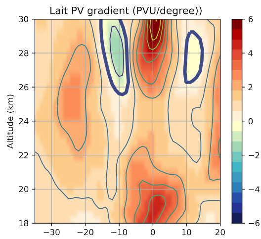
Figure 8. Meridional gradient of the zonal and time average average-averaged Lait PV defined in Appendix A2. The unit is PVU per degree where 1 PVU = 10^6 \text{ m}^2 \text{ K s}^{-1} \text{ kg}^{-1} .
