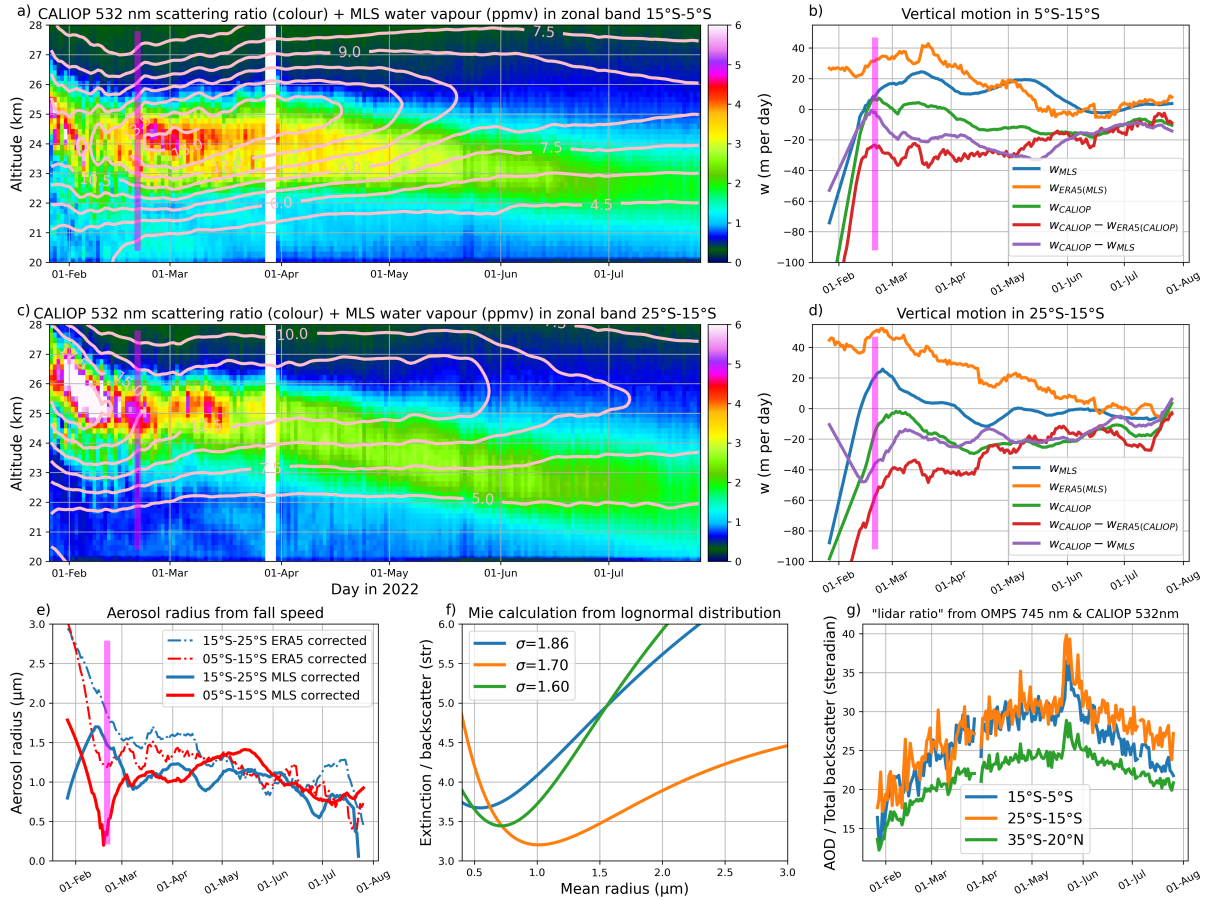
Figure 3. (a) and (c): Zonal and latitude band averages as a function of time for CALIOP 532 nm scattering ratio (colour) and MLS water vapour (contours, ppmv) for, respectively, the 15°S-5°S and 25°S-15°S latitude bands, respectively. (b) and (d): Vertical motions for the same two latitude bands: W_{\text{CALIOP}} for aerosol plume and W_{\text{MLS}} for water vapour plume deduced from (a) and (c) (Appendix A3), W_{\text{diab}} and W_{\text{ERA5}} - W_{\text{ERA5(MLS)}} for ERA5 diabatic and total ascent rate (diabatic + adiabatic Appendix A2) ascent rates, and W_S = W_{\text{CALIOP}} - W_{\text{ERA5}} for at the resulting vertical motion location of the aerosol-MLS plume, W_{\text{CALIOP}} - W_{\text{ERA5(CALIOP)}} and W_{\text{CALIOP}} - W_{\text{MLS}} for the CALIOP sedimentation speed estimated, respectively, with respect to the ERA5 air ascent rate and the MLS water ascent rate (Appendix A3). (e): Aerosol radius deduced from w_s the aerosol sedimentation speed interpreted as an aerosol fall speed and using Eq. (9.42) of Seinfeld and Pandis (2016). The dash lines show the estimate for the ERA5 correction which is applicable after May when the aerosol and moist layers are separated and the water vapour cooling has ceased and the solid lines show the estimate for the MLS correction which is valid as long as the aerosol and moist layers overlap (Appendix A3). (f): Ratio of the theoretical 745 nm aerosol extinction and 532 nm aerosol backscatter cross sections, calculated using a Mie code (see Appendix A4) with three values of the standard deviation \sigma . (g): Ratio of the 745 nm OMPS LP aerosol optical depth and 532 nm CALIOP integrated attenuated backscatter, both over the vertical range 18 to 30 km. The curves are shown for the same latitude bands as in a) and c) and for band the 35°S-20°N band that encompasses also the periphery of the aerosol plume. In panels (a-e), a vertical line is drawn on 20 February to indicate the separation between the two phases of the vertical motion as discussed in Sec. 2. During the last third of May, both OMPS LP and CALIOP are perturbed by the intensified solar activity and the peak seen in panel (g) at such dates must be considered as spurious.
