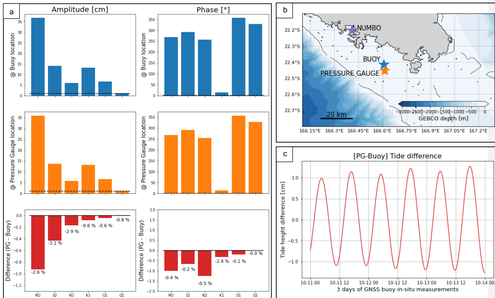
200 Figure D4. (a) Amplitude and phase of the six main tide constituents extracted from SCHISM hydrodynamic model at the buoy (blue) and pressure gauge location (orange). The red bar plot show amplitude and phase of the tide gradient between these two points. / (b) Location of the sensors. Note stars colours correspond to bar plot colours. / (c) Tide reconstruction over the 3 days of the GNSS buoy measurements using amplitude and phase of the tide gradient.
