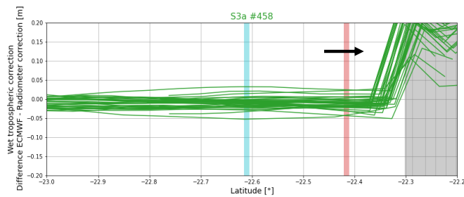
Figure E2. Evolution of the difference between ECMWF and the radiometer correction along the altimetric tracks used in our study (red for Jason 3 #162, orange for Sentinel-3a #359 and green for Sentinel-3a #458). The grey vertical bar represents the main island overfly, the red vertical bar represents the comparison point location and the blue vertical bar corresponds to the reef barrier overfly. Arrows symbolize the satellite direction of flight.
