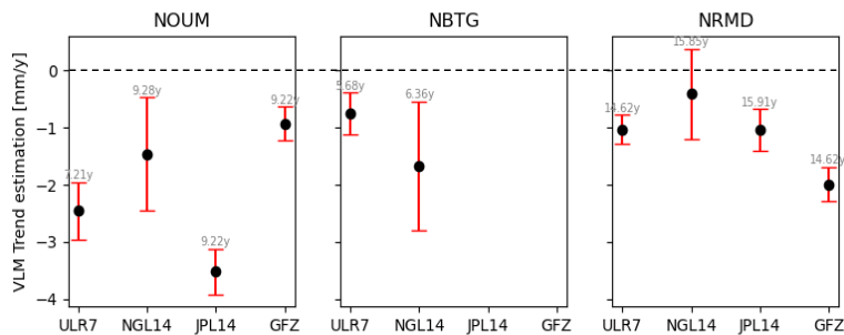
Figure A2. VLM trend estimation at three GNSS station in Noumea from 4 different solutions : SONEL-ULR7 solution from Gravelle et al. (2022) / NGL - NGL14 solution from Blewitt et al. (2016) / JPL - JPL14 solution from Heflin et al. (2020) / GFZ – GT3 solution from Männel et al. (2022). The red bar represents the uncertainty associated with each estimate, and the number shows the length of the observation years used to estimate the trend.
