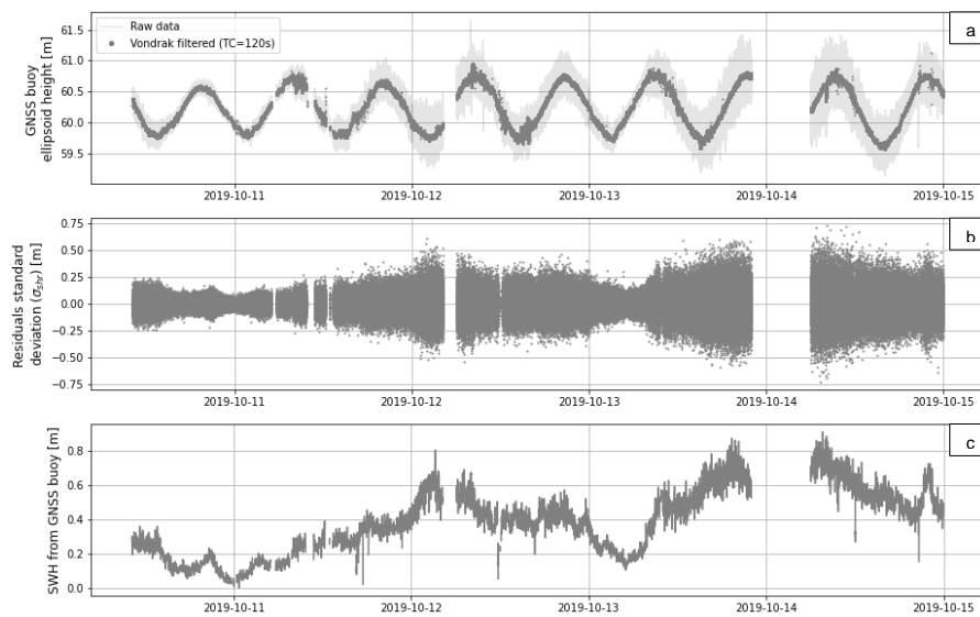
Figure D1. Computation step of the GNSS Buoy SWH / (a) Raw and Vondrak filtered GNSS buoy ellipsoid heights / (b) Standard deviation of the residuals' heights computed on 120s window ( \sigma_{str} ) / (c) Significant Wave Height (SWH) at the buoy position.
