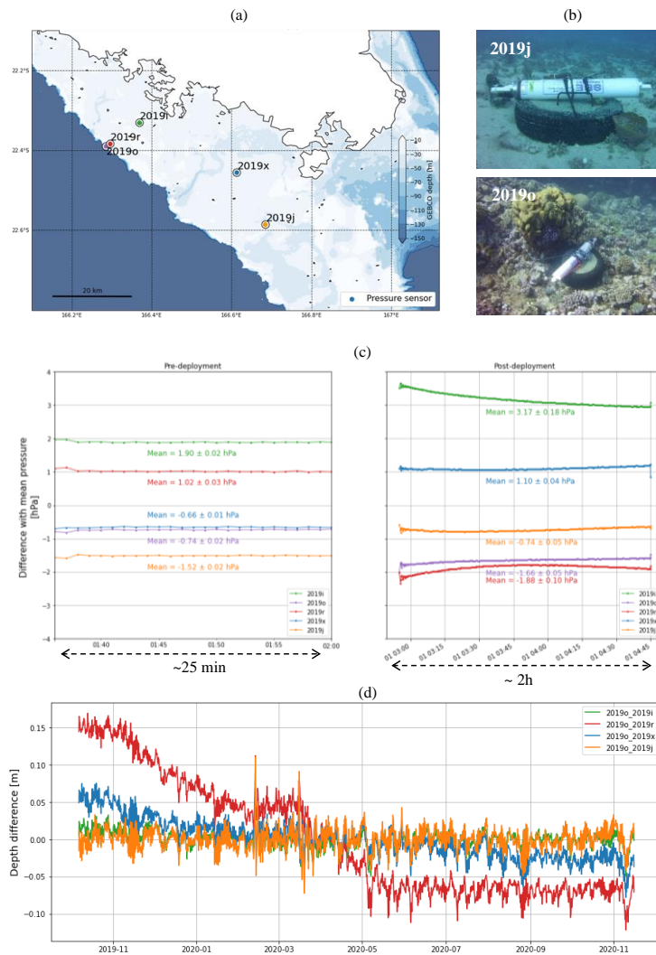
Figure B1. Installation and calibration phase of the pressure gauges / (a) – (b) Location and mooring of the 5 pressure gauges deployed during GEOCEAN-NC campaign. / (c) Hyperbaric chamber calibration results: difference between SBE observations and mean pressure at 10m before (left) and after (right) deployment. For conversion, 1 hPa ~ 1 cm of water. / (d) Difference between the 2019o sensor time series and the other 4 pressure sensors. The pressure time series were transformed into equivalent water depths and then corrected for tide using harmonic analysis. The final differences were filtered with a sliding average (6 h windows, 6 h steps).
