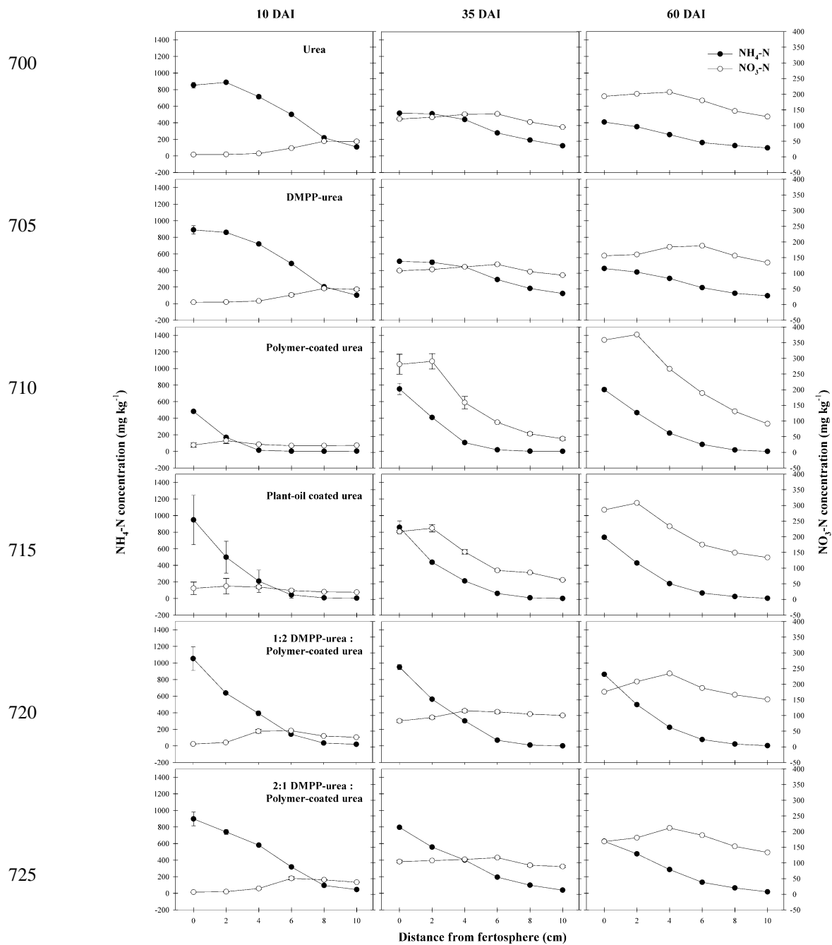
Figure 5. Concentration (mg N kg -1 soil) of mineral N species from N-fertilizer treatments in the Ferralsol during a 60-day incubation (DAI). Vertical bars represent the standard error of the mean.
