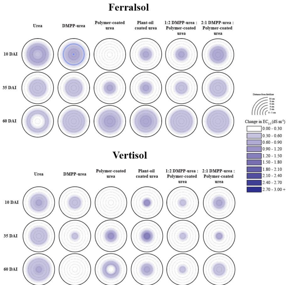
660 Figure 2. Heat maps displaying changes (with respect to untreated soil, Table 1) in electrical conductivity (EC, dS m -1 ) distribution from bands of N-fertilizer treatments in the Ferralsol and Vertisol over time (days after incubation; DAI). Initial EC values were 0.07 dS m -1 (Ferralsol) and 0.35 dS m -1 (Vertisol). Changes in the EC of untreated soil are presented in the Supplementary Material (Part A, Table S1).
