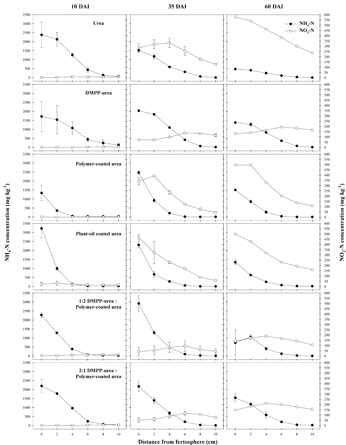
Figure 6. Concentration (mg N \text{kg}^{-1} soil) of mineral N species from N-fertilizer treatments in the Vertisol during a 60-day incubation (DAI). Vertical bars represent the standard error of the mean.
