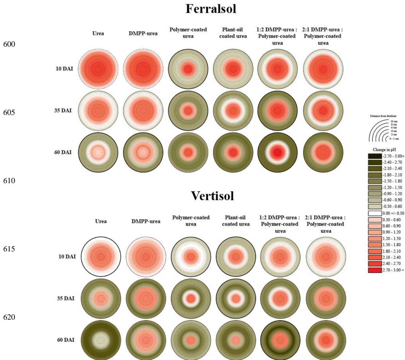
625 Figure 1. Heat maps displaying changes (with respect to untreated soil, Table 1) in pH distribution from bands of N-fertilizer treatments in the Ferralsol and Vertisol over time (days after incubation; DAI). Initial pH values were 6.30 (Ferralsol) and 7.15 (Vertisol). Changes in the pH of untreated soil are presented in the Supplementary Material (Part A, Table S1).
