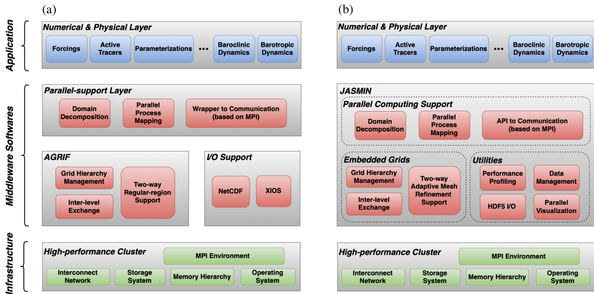
Figure 1. RC1 Model structure of NEMO (a) and OMARE (b).
