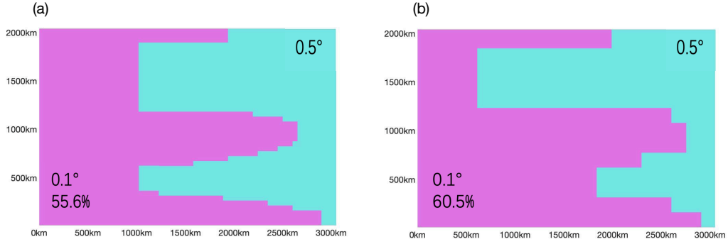
Figure 6. Two regional refinement settings from 0.5^\circ to 0.1^\circ of the Double-Gyre case. RC2 Panel a and b shows L-M-I and L-M-II respectively. The background and the whole ocean basin is by default in 0.5^\circ resolution and marked in cyan, and the region refined to 0.1^\circ in each experiment marked in purple.
