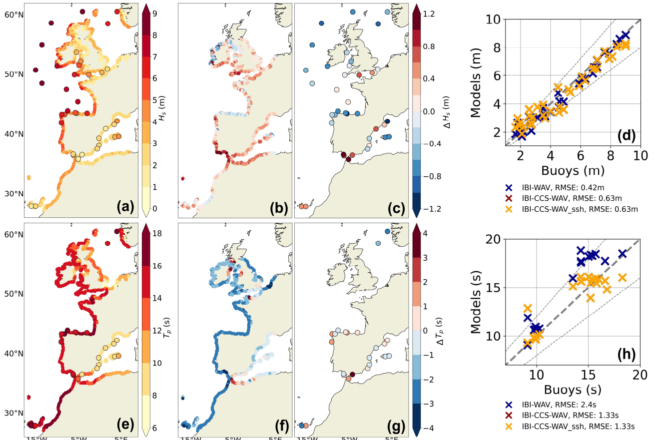
Figure 3: (a), (b), (c) and (d) show the 99 th percentile (based on hourly outputs) coastal significant wave height ( H_s , in m) over the 1993-2014 period for: (a) IBI-CCS-WAV for the domain and wave buoys for the circles. (b) Differences between IBI-CCS-WAV and the reanalysis. (c) Bias between IBI-CCS-WAV and wave buoys at buoys locations. (d) Scatter plot at each wave buoy location of simulations IBI-CCS-WAV (red marks), IBI-CCS-WAV_ssh (yellow marks) and the reanalysis (blue marks) vs observations. (e), (f), (g) and (h) are the corresponding figures for the coastal peak period ( T_p , in s). (h) must be interpreted with caution as the observations are scarce. Note the different color bars in (a) and (b), (c), and in (e) and (f), (g). For (b) and (f) the domain is limited to the domain distributed by
