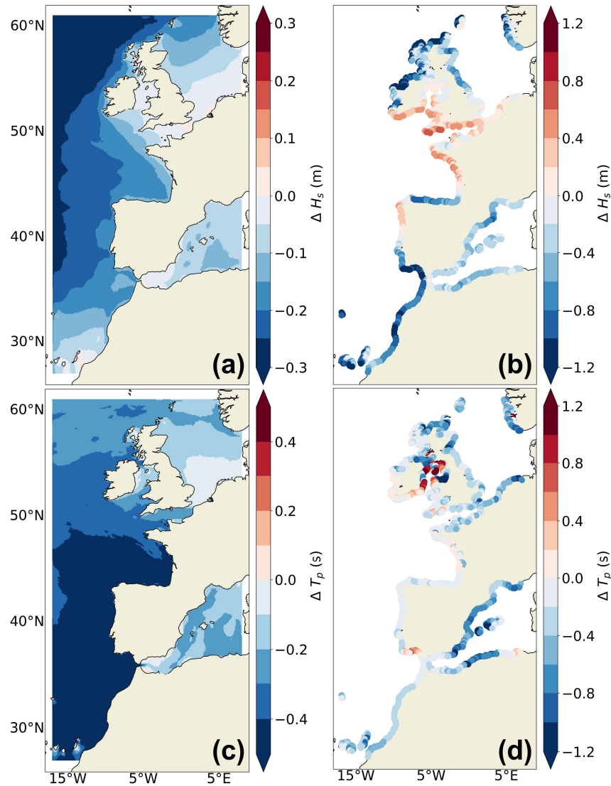
Figure 5: Projected changes in mean (first column) and coastal extreme 1-in-100-year (second column) wave conditions for the 2081-2100 period (relative to 1986-2005) under the SSP5-8.5 climate scenario for (a,b) the significant wave height ( \Delta H_s , in m) and (c,d,) the peak period ( \Delta T_p , in s).
