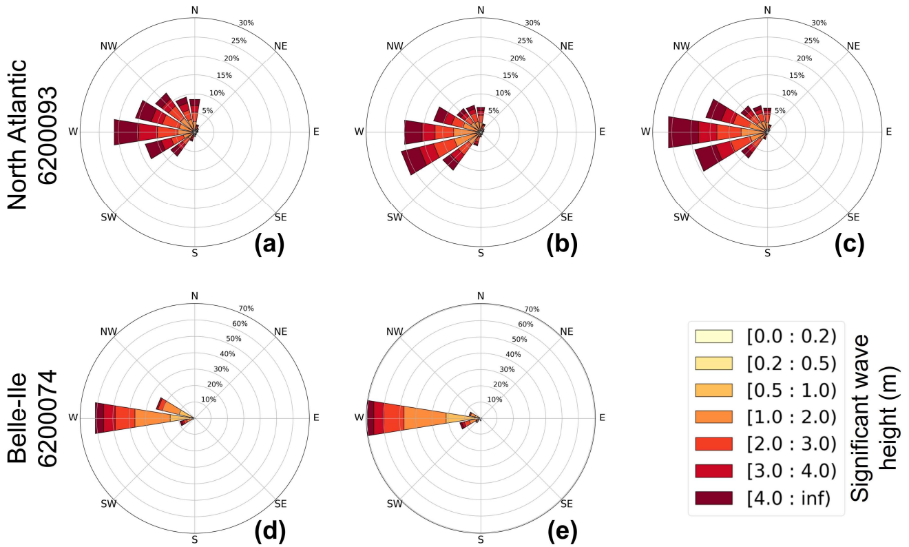
Figure 4: Directional distributions of significant wave height at star locations of Fig. 1a: North Atlantic buoy 6200093 (first row), Belle-Ile buoy 6200074 (French Atlantic coast, second row). First column are the wave roses based on wave buoy data over the (a) 2003-2022 and (d) 2005-2022 periods. Second column (b,e) are the roses for IBI-CCS-WAV over the 1993-2014 period and last column (c) for the reanalysis over the 1993-2014 period. Different periods are chosen for the wave buoys because of the lack of data for the wave direction over the 1993-2014 period. Wave roses at North Atlantic buoy 6200093 location were computed using mean wave direction. Wave roses at Belle-Ile buoy 6200074 location were computed using the wave direction at spectral peak as it was the data provided by the wave buoy. However, this variable was not an output of the reanalysis. Colors indicate the wave height distribution in each direction bin.
