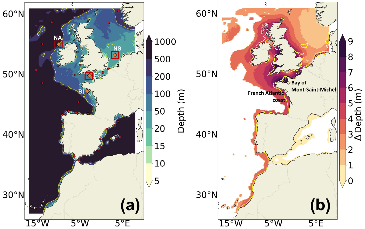
Figure 1: (a) Bathymetry (m) of the IBI domain in the regional wave model. The shelf break (defined by the 200 m isobath) is indicated by the solid yellow line. The yellow dotted lines indicate the areas where the waves start to interact with the bathymetry in IBI-CCS-WAV (intermediate waters that cannot be considered as purely deep water), identified when h < L/2 with h the bathymetry and L the mean wavelength over the 1993-2014 period. The red dots represent the locations of the wave buoys from the Copernicus Marine Service (Wehde et al., 2021) used for the validation in Sect. 3.1. The three red boxes are used in Appendix A to validate extreme winds of the global climate model. Orange diamonds indicate the wave buoys: used for the wave roses calculation of Sect. 3.1.2 and 3.2.2 (North Atlantic (NA) buoy 6200093 and Belle-Ile (BI) buoy 6200074), used for the extreme wind validation in Appendix A (North Atlantic (NA) buoy 6200093, English Channel (EC) buoy 6200103 and North Sea (NS) buoy 6200145). (b) Bathymetric adjustment (Sect. 2.3) that corresponds approximately to the M2 tidal range from the 3D regional ocean model (1993-2014). The lines indicate the areas where the waves start to interact with the bathymetry at low tide (dashed white lines) and at high tide (solid yellow lines). The two yellow diamonds indicate the zones where the impact of including hourly sea level outputs in the wave model is assessed in Sect. 4.
