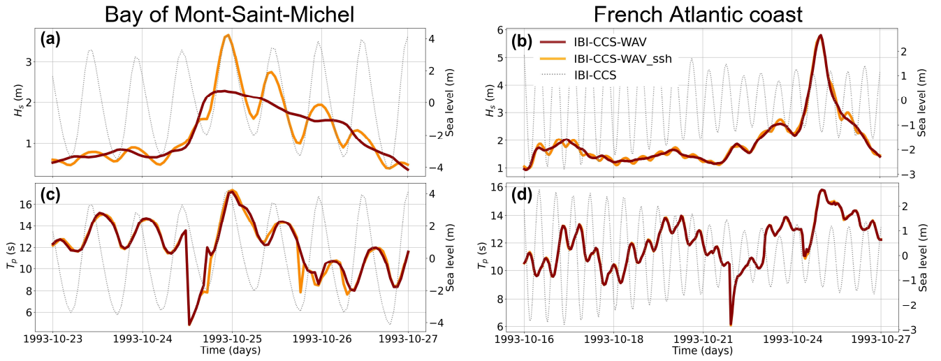
Figure 9: Time series of incoming wave conditions for the Bay of Mont-Saint-Michel (first column) and for the French Atlantic coast (second column) during an extreme significant wave height event of October 1993. The two locations are marked on Fig. 1b. The curves represent IBI-CCS-WAV (dark red curve) and IBI-CCS-WAV_ssh (dark yellow curve) for (a,b) the significant wave height ( H_s , in m), and (c,d) the peak period ( T_p , in s). Sea level variations are shown in thin grey dotted lines, with the right y-axis on each panel.
