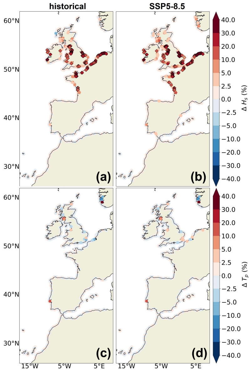
330 Figure 9: Impact of the inclusion of hourly sea level variations in the wave model on the 1-in-100-year return level of (a,b) significant wave height (first row, \Delta H_s , in %) and (c,d) peak period (second row, \Delta T_p , in %). The first column shows the relative differences of the 1-in-100-year return level between IBI-CCS-WAV_ssh and IBI-CCS-WAV for the 1986-2005 period. The second column shows the relative differences of the 1-in-100-year return level between IBI-CCS- WAV_ssh and IBI-CCS-WAV for the 2081-2100 period under the SSP5-8.5 scenario. The large diamonds represent the locations where the differences between both simulations are significant (i.e. where the confidence intervals associated with the 100-year return level calculation are disjoint). Note that the color bars of Figure 8 and 9 are not linear and are identical to facilitate the comparisons between the two figures. 335
