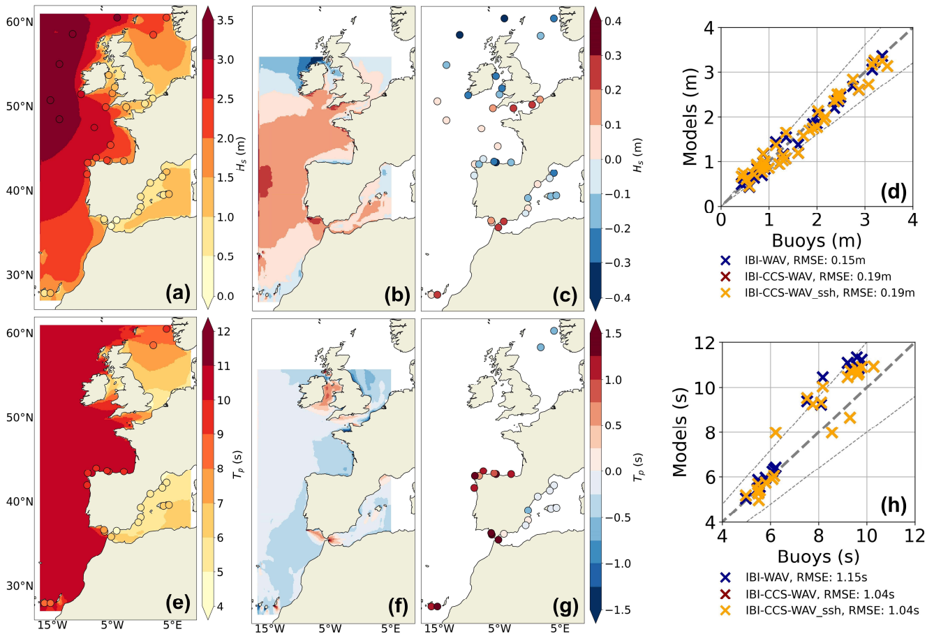
Figure 3: (a), (b), (c) and (d) show the mean significant wave height ( H_s , in m) over the 1993-2014 period for: (a) IBI-CCS-WAV for the domain and wave buoys for the circles. (b) Differences between IBI-CCS-WAV and the reanalysis. (c) Bias between IBI-CCS-WAV and wave buoys at buoys locations. (d) Scatter plot at each wave buoy location of IBI-CCS-WAV (red marks), IBI-CCS-WAV_ssh (yellow marks) and the reanalysis (blue marks) vs observations. (e), (f), (g) and (h) are the corresponding figures for peak period ( T_p , in s). (h) must be interpreted with caution as the observations are scarce. For (b) and (f) the domain is limited to the domain distributed by the Copernicus Marine Service, with a cut in the northern part. In (d) and (h), the thin dashed lines indicate the 20 % error margin. The RMSE is calculated as the root mean squared deviations from the line y=x (spatial RMSE).
