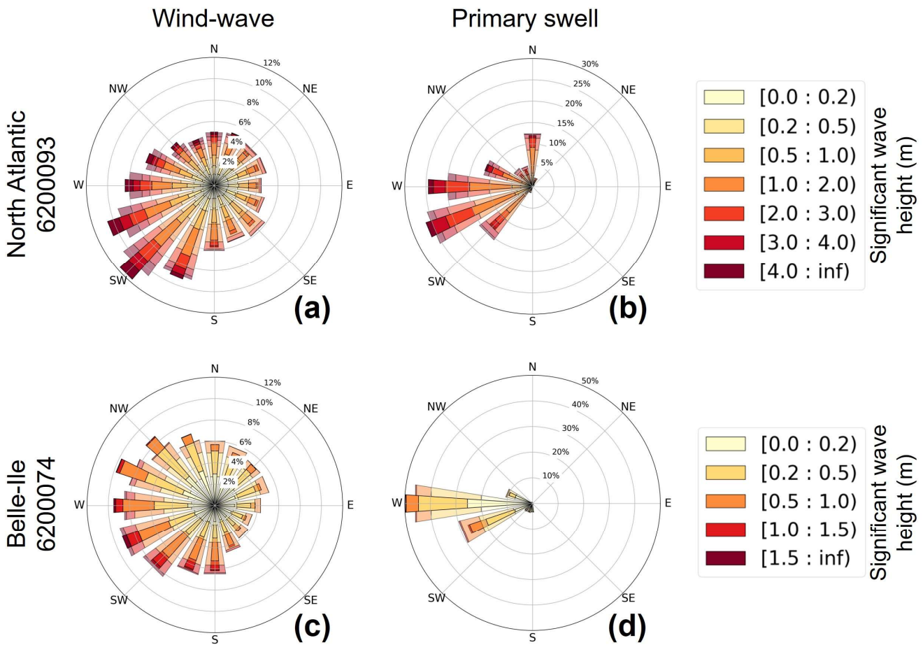
280 Figure 7: Projected changes (SSP5-8.5 scenario) in directional distribution of significant wave height for the 2081-2100 period (narrow angle bins, dark colors) relative to 1986-2005 (wide angle bins, pale colors) in IBI-CCS-WAV at star locations of Fig. 1a: North Atlantic buoy 6200093 (first row) and Belle-Ile buoy 6200074 (second row). The significant wave height and mean wave direction have been classified according to their origin: wind-wave (a,c) and primary swell (b,d). Colors indicate wave height distribution in each direction bin.
