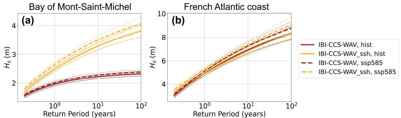
Figure 11: Return period curves of significant wave height ( H_s , in m) for IBI-CCS-WAV (dark red curves) and IBI-CCS-WAV_ssh (dark yellow curves) for (a) the Bay of Mont-Saint-Michel and (b) the French Atlantic coast (Fig. 1b). The solid lines represent the 1985-2006 period and the dashed lines the 2081-2100 period under the SSP5-8.5 scenario. The thin solid and dashed lines are the confidence intervals (corresponding to 1 sigma confidence) associated with the
