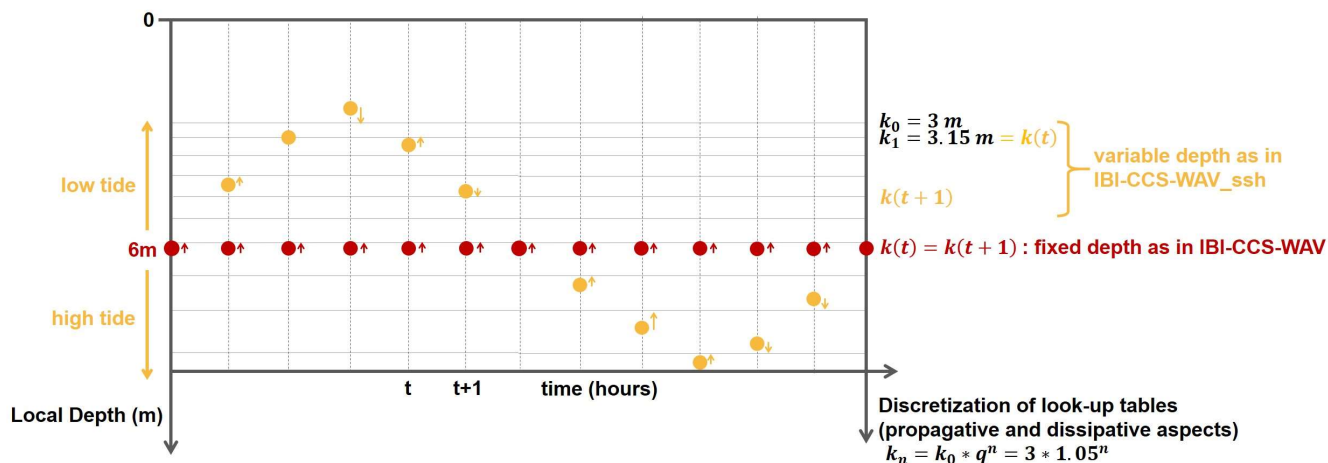
145 Figure 2: Schematic of the inclusion of sea level variations in the wave model for a given coastal point as a function of time. The dots represent the local depths. In red, the local depth is fixed (IBI-CCS-WAV), and in this example the local depth is the minimum allowed. In yellow, an example of the time evolution of the local depth corresponding to the hourly sea level variations (IBI-CCS-WAV_ssh), here dominated by a tidal signal. The q_n terms represent the vertical discretization of the depths used in the look-up tables to obtain parameters needed for wave propagation and source terms. These discretized depths are chosen as close as possible to the local depths estimated from the bathymetry with sea level changes added.
