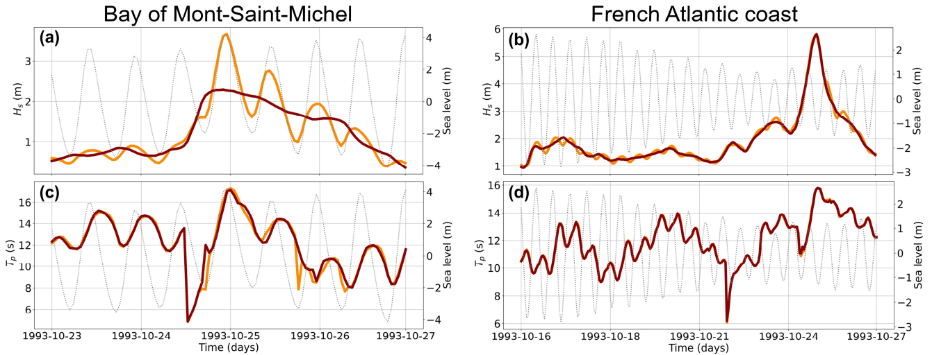
Figure 10: Time series of incoming wave conditions for the Bay of Mont-Saint-Michel (first column) and for the French Atlantic coast (second column) during an extreme significant wave height event of October 1993. The two locations are marked on Fig. 1b. The curves represent IBI-CCS-WAV (dark red curve) and IBI-CCS-WAV_ssh (dark yellow curve) for (a,b) the significant wave height ( H_s , in m), and (c,d) the peak period ( T_p , in s). Sea level variations are shown in thin grey dotted lines, with the right y-axis on each panel.
