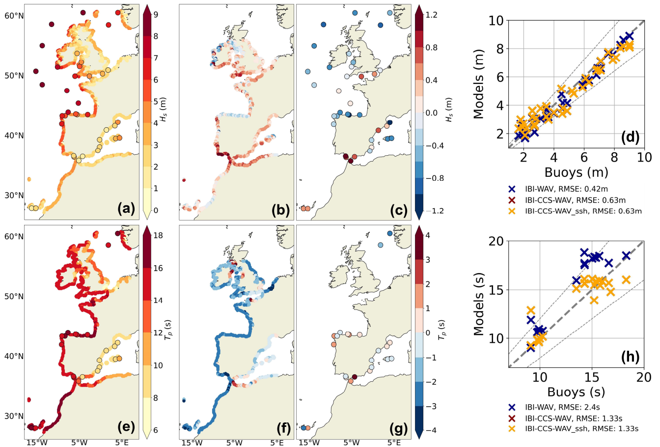
200 Figure 4: (a), (b), (c) and (d) show the 99 th percentile (based on hourly outputs) coastal significant wave height ( H_s , in m) over the 1993-2014 period for: (a) IBI-CCS-WAV for the domain and wave buoys for the circles. (b) Differences between IBI-CCS-WAV and the reanalysis. (c) Bias between IBI-CCS-WAV and wave buoys at buoys locations. (d) Scatter plot at each wave buoy location of simulations IBI-CCS-WAV (red marks), IBI-CCS-WAV_ssh (yellow marks) and the reanalysis (blue marks) vs observations. (e), (f), (g) and (h) are the corresponding figures for the coastal peak period ( T_p , in s). (h) must be interpreted with caution as the observations are scarce. Note the different color bars in (a) and (b), (c), and in (e) and (f), (g). For (b) and (f) the domain is limited to the domain distributed by the Copernicus Marine Service, with a cut in the northern part. In (d) and (h), the thin dashed lines indicate the 20% error margin. The RMSE is calculated as the root mean squared deviations from the line y=x (spatial RMSE). Note that the color scales for the biases are larger than for Figure 3.
