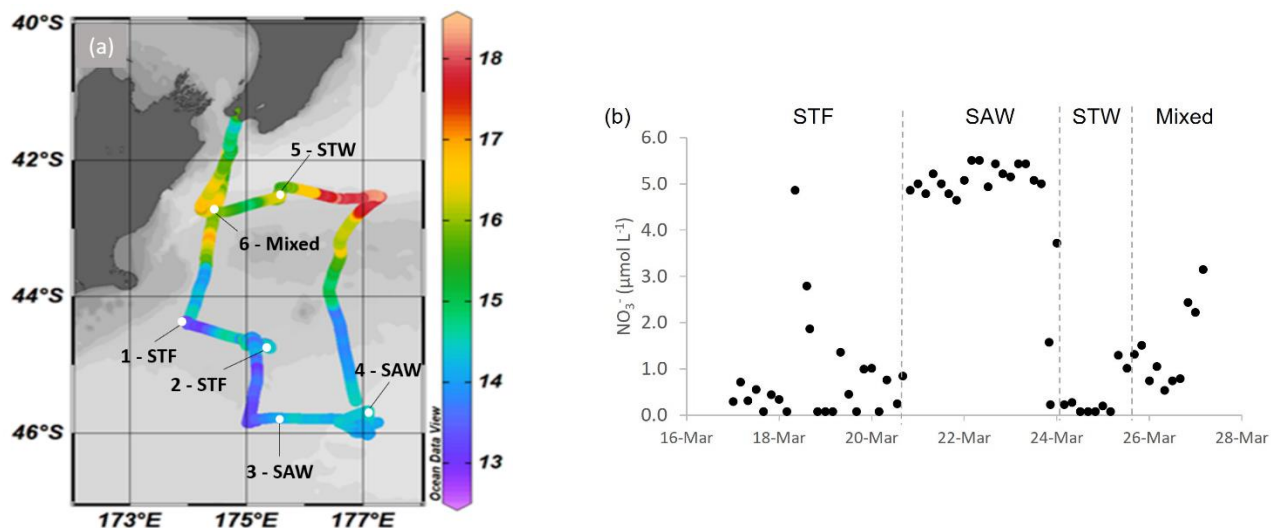
Figure 1: (a) Sea2Cloud voyage track overlain by sea surface temperature ( ^{\circ}\text{C} ), using Ocean Data View (Schlitzer, 2020), with workboat station positions identified. The grey shading shows the undersea topography, with the darker grey band along 43.5^{\circ}\text{S} indicating the Chatham Rise. (b) Nitrate concentration during the Sea2Cloud voyage, measured at 5 m. Water mass type is indicated by the labels at the top of the figure and separated by the grey vertical dashed lines.
