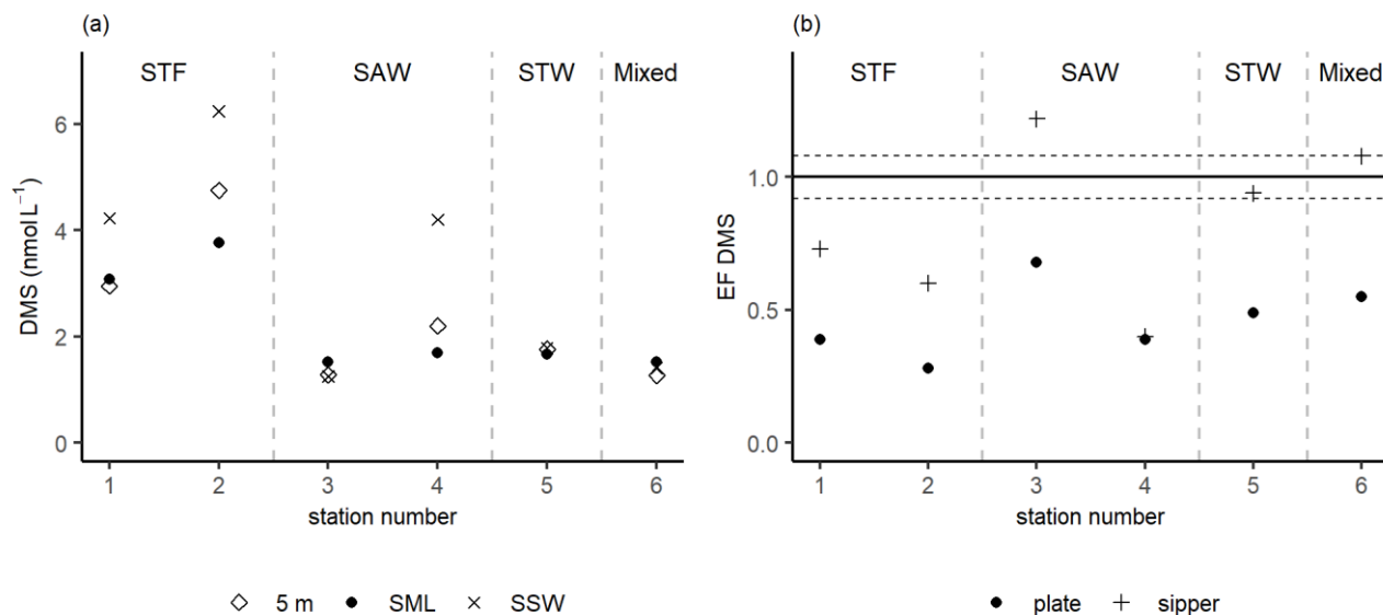
260 Figure 4: (a) DMS concentrations in the SML (from the gas-permeable tube), SSW, and at 5 m depth, and (b) EF DMS determined by the gas-permeable tube and glass plate. The horizontal dashed lines represent the significance threshold determined from the median repeatability of the gas-permeable tube (8%). Water mass type is indicated by the label at the top of the figure and separated by the grey vertical dashed lines.
