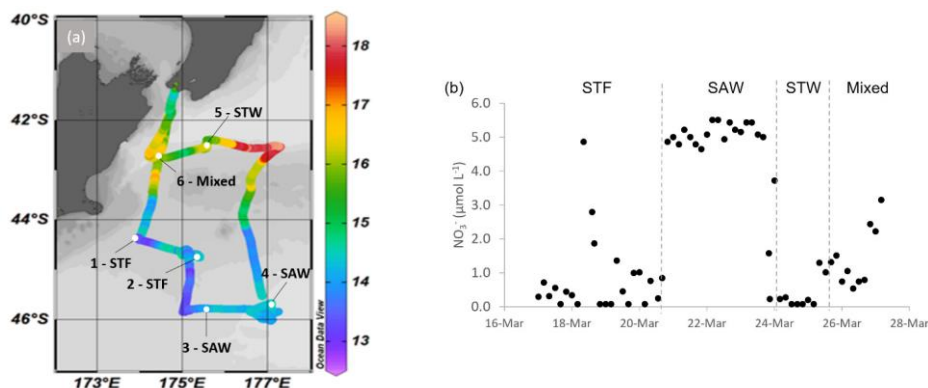
Figure 1: (a) Sea2Cloud voyage track overlain by sea surface temperature ( ^{\circ}\text{C} ), using Ocean Data View (Schlitzer, 2020), with workboat station positions identified. The grey shading shows the undersea topography, with the darker grey band along 43.5^{\circ}\text{S} indicating the Chatham Rise. (b) Nitrate concentration during the Sea2Cloud voyage, measured at 5 m. Water mass type is indicated by the labels at the top of the figure and separated by the grey vertical dashed lines.
