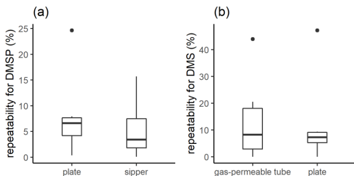
Figure 2: Box plot of the repeatability for (a) DMSP measurements with the plate and the sipper, and (b) DMS measurements with the gas-permeable tube and the plate. The boxplot represents the distribution of the data, with the box corresponding to the interquartile range and the bold horizontal line the median. The limits of the vertical lines represent the upper and lower fences. The outliers are represented by points outside the fences.
