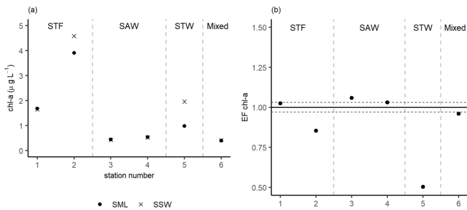
Figure 5: (a) Chl- a concentrations in the SML, and SSW, and (b) EF chl- a , with the horizontal dashed lines representing the significance threshold determined from the repeatability of the sipper (3%). Water mass type is indicated by the label at the top of the figure and separated by the grey vertical dashed lines.
