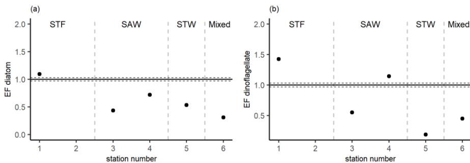
Figure 8: EF phytoplankton carbon content for (a) diatoms and (b) dinoflagellate of >5 μm. The horizontal dashed lines represent the significance threshold determined from the repeatability of the sipper (3%). Water mass type is indicated by the label at the top of the figure and separated by the grey vertical dashed lines.
