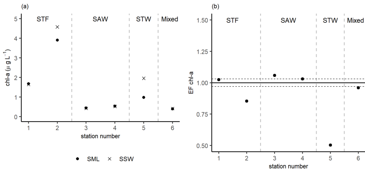
Figure 5: (a) Chl- a concentrations in the SML, and SSW, and 5-m depth, and: (b) EF cChl- a enrichment in the SML relative to the SSW and 5-m, with the horizontal dashed lines representing the significance threshold determined from the reproducibility/repeatability of the sipper (3%). Chl- a enrichment relative to 5-m at 2-STF is off-scale at 2.88 as indicated by the vertical arrow. Water mass type is indicated by the label at the top of the figure and separated by the grey vertical dashed lines also the shading.
