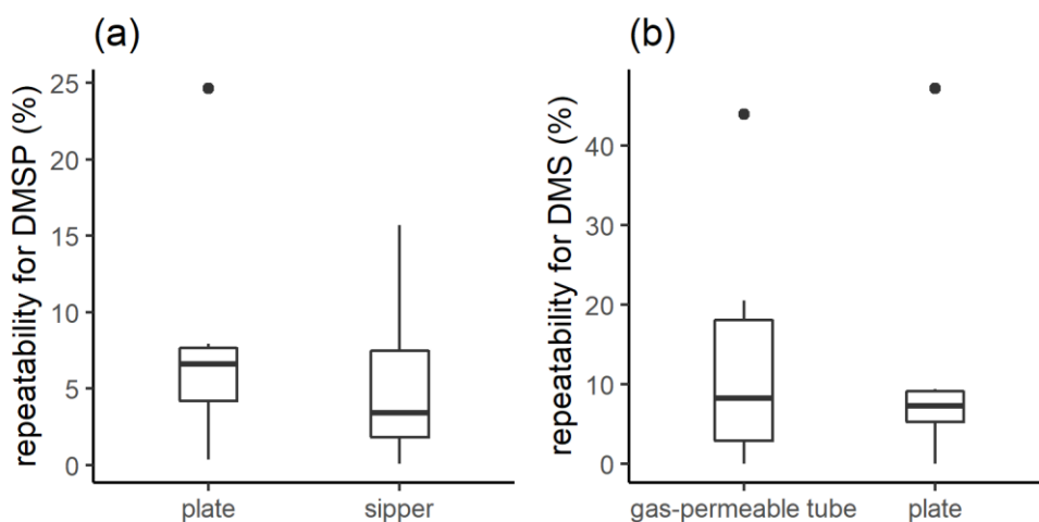
245 Figure 2: Box plot of the reproducibility repeatability for (a) DMSP measurements with the plate and the sipper, and (b) DMS measurements with the gas-permeable tube and the plate. The boxplot represents the distribution of the data, with the box corresponding to the interquartile range and the bold horizontal line the median. The limits of the vertical lines represent the upper and lower fences. The outliers are represented by points outside the fences.
