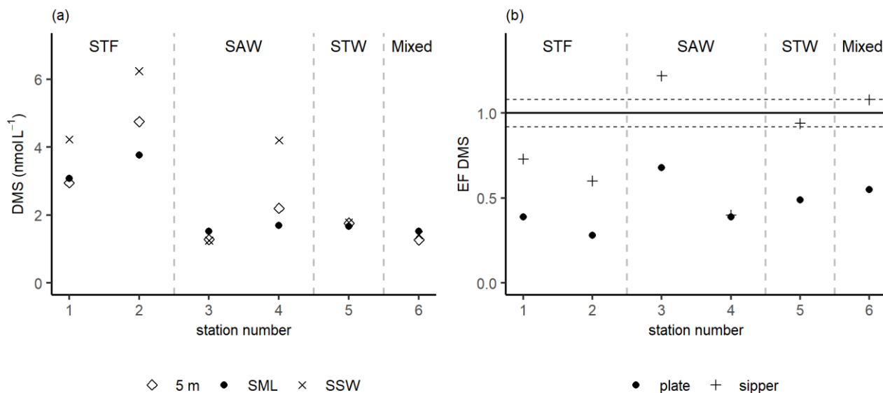
270 Figure 4: (a) DMS concentrations in the SML (from the gas-permeable tube), SSW, and at 5 m depth, and (b) EF DMS determined by the gas-permeable tube and glass plate. The horizontal dashed lines represent the significance threshold determined from the median reproducibility/repeatability of the gas-permeable tube (8%). Water mass type is indicated by the label at the top of the figure and separated by the grey vertical dashed lines also the shading.
