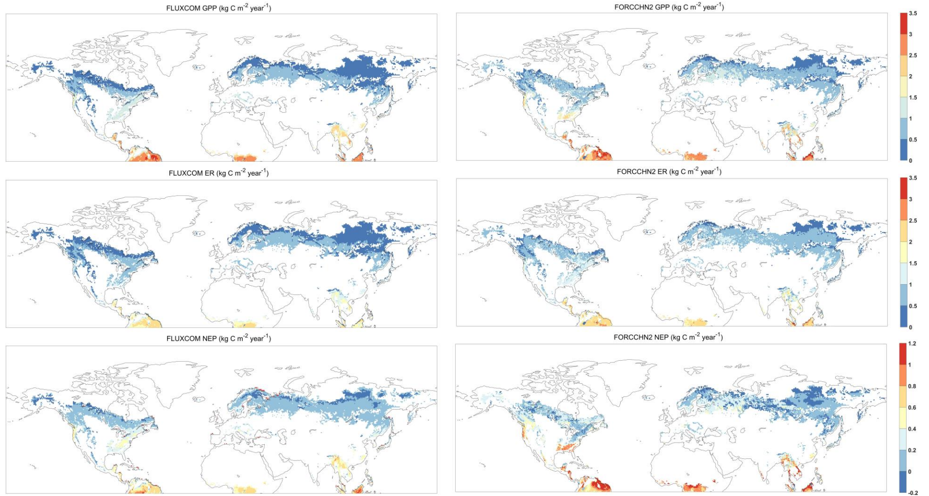
Fig. S3. The mean spatial distribution of FORCCHN2 and FLUXCOM gross primary productivity (GPP), ecosystem respiration (ER), and net ecosystem productivity (NEP) across the Northern Hemisphere during 1980–2013. The fluxes of FLUXCOM are extracted from the ‘RS+METEO’ dataset. The FLUXCOM NEP is equaled to the negative of net ecosystem CO 2 exchange (NEE). The spatial resolution is 0.5°×0.5°.
