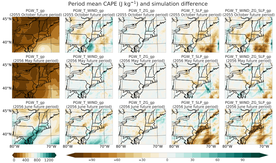
Figure 12. Period mean convective available potential energy (CAPE) ( \text{J kg}^{-1} ) over the whole inner from the simulation with temperature perturbation at each gridpoint, and the differences between the simulations with additional perturbations of wind, geopotential height, sea level pressure and their combination at each gridpoint and the simulation with temperature perturbation only.
