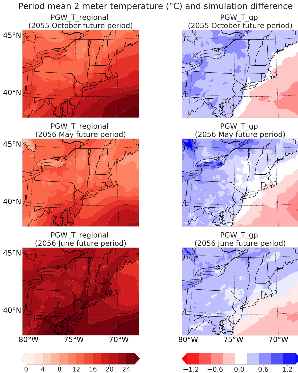
Figure 4. (Left) Period mean 2-meter-2-meter temperature ( ^{\circ}\text{C} ) over the inner domain from the simulation with temperature perturbation at regional mean scale. (Right) Differences between the period mean 2-meter-2-meter temperature ( ^{\circ}\text{C} ) from the simulation with gridpoint perturbation and the simulation with regional mean simulation from perturbation shown on the left column .
