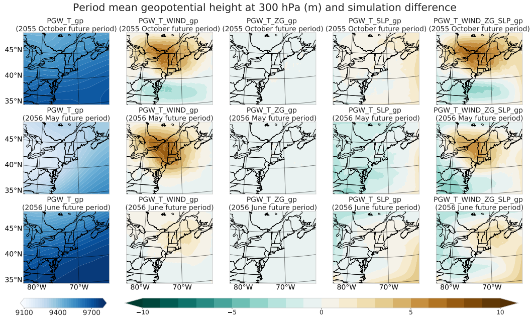
Figure 8. Period mean geopotential height and simulation deltas (m) at 300 hPa over the whole domain from the simulation with temperature perturbation at each gridpoint, and simulated perturbations in the differences between simulations with additional dynamical perturbations of wind, geopotential height, sea level pressure and the combination of them at each gridpoint and the simulation with only temperature perturbation.
