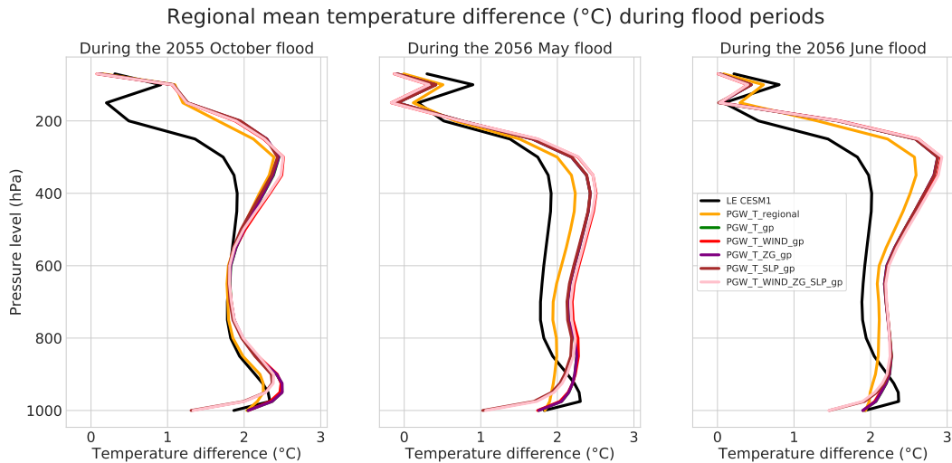
Figure 14. Period regional Regional mean temperature differences ( ^{\circ}\text{C} ) at each pressure levels-level over the inner domain. The baseline is between each PGW simulation of the future and the historical simulation averaged over the flood period.
