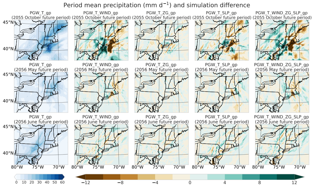
Figure 7. Period mean precipitation (mm d -1 ) over the inner domain from the simulation with only temperature perturbation at each gridpoint, and simulated differences in-the-between simulations with additional dynamical perturbations of wind, geopotential height, sea level pressure and the combination of them at each gridpoint and the simulation with temperature perturbation at each gridpoint only .
