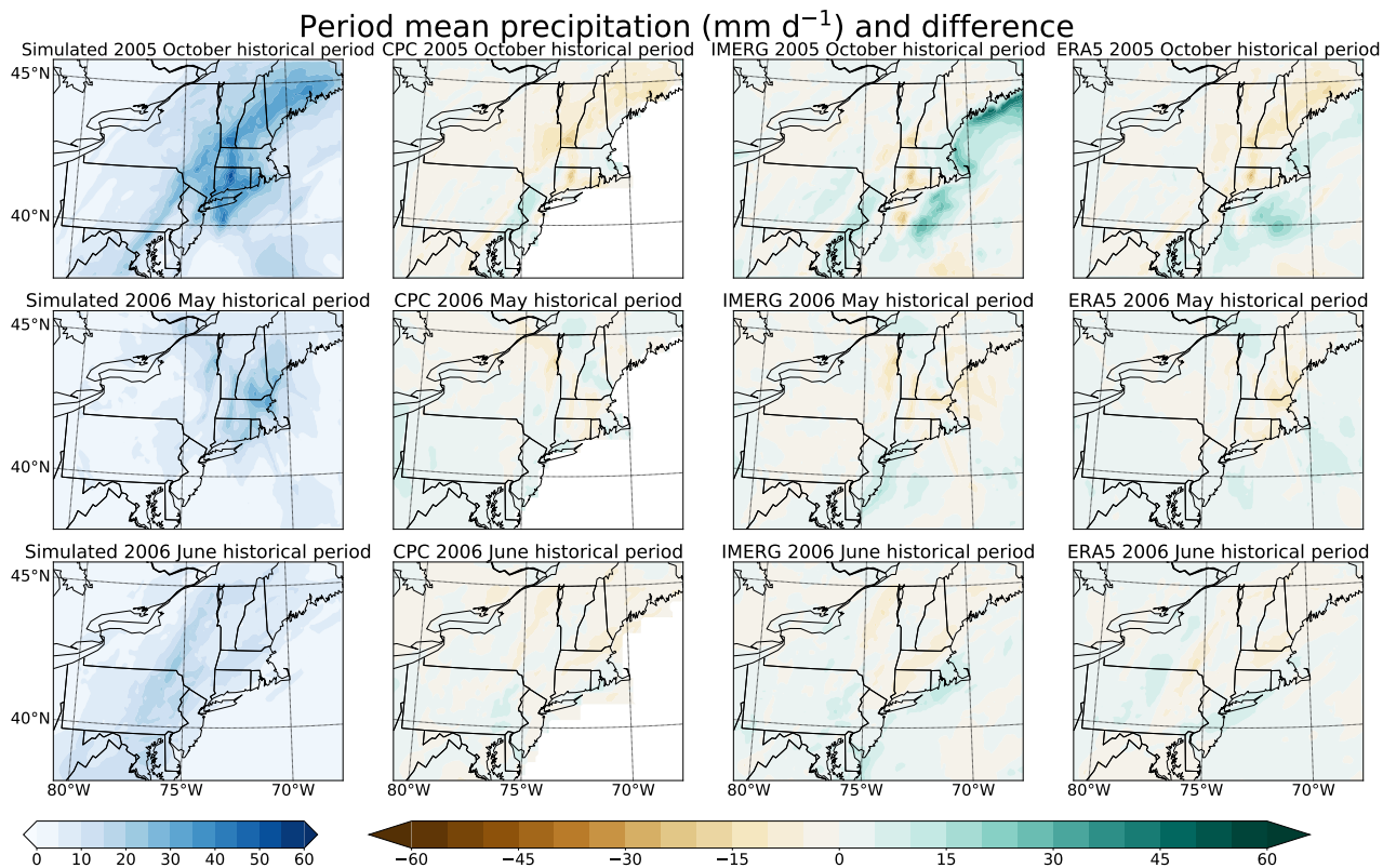
Figure 3. Average (Left) Period mean precipitation (mm d -1 ) over the inner domain from our the historical PGW-simulation, (Right) Differences between the period mean precipitation (mm d -1 ) from the CPC observational data, IMERG and ERA5 reanalysis data from during flood periods, and the historical simulation shown on the left column.
