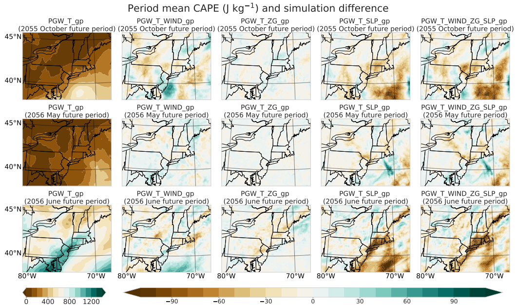
Figure 13. Period mean convective available potential energy (CAPE) and simulation deltas ( \text{J kg}^{-1} ) over the whole domain relative to inner from the simulation with temperature perturbation at each gridpoint, and simulated deltas when performing experiments the differences between the simulations with additional perturbations of wind, geopotential height, sea level pressure and their combination at each gridpoint and the simulation with temperature perturbation only.
