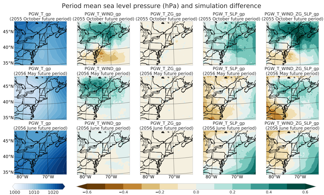
Figure 10. Period mean sea level pressure and simulation deltas ( \text{mm d}^{-1}\text{hPa} ) over the whole domain from the simulation with temperature perturbation at each gridpoint, and simulated-deltas-when-performing-experiments-differences between the simulations with additional perturbations of wind, geopotential height, sea level pressure and their combination at each gridpoint and the simulation with temperature perturbation only.
