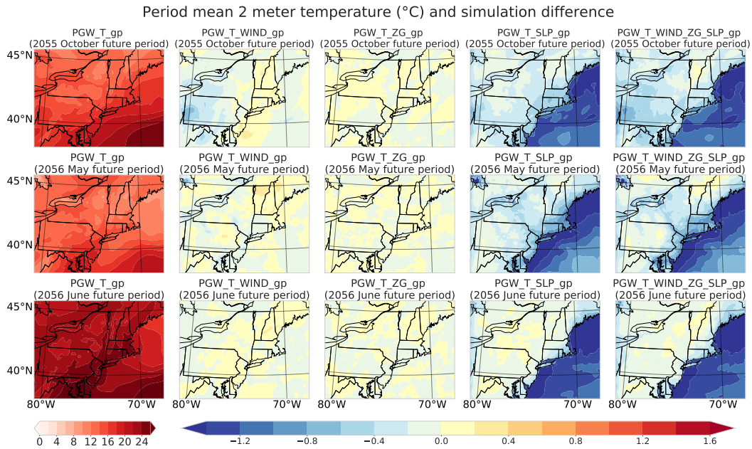
Figure 11. Period mean temperature and simulation deltas ( ^{\circ}\text{C} ) at 2 meter over the whole inner domain relative to from the simulation simulations with temperature perturbation at each gridpoint, and simulated deltas when performing experiments the differences between the simulations with additional perturbations of wind, geopotential height, sea level pressure and their combination at each gridpoint and the simulation with temperature perturbation only.
