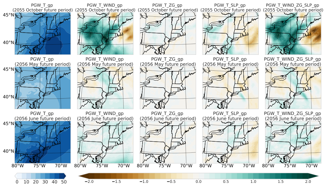
Figure 12. Period mean precipitable water and simulation deltas (mm) over the whole inner domain relative to from the simulation with temperature perturbation at each gridpoint, and simulated deltas when performing experiments the differences between the simulations with additional perturbations of wind, geopotential height, sea level pressure and their combination at each gridpoint and the simulation with temperature perturbation only .
