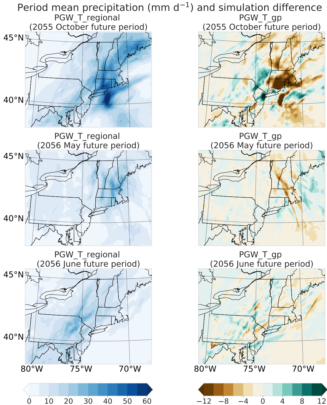
Figure 5. (Left) Period mean precipitation (mm d -1 ) over the inner domain from the simulation with temperature perturbation at regional mean scale. (Right) Differences between the period mean precipitation from the simulation with gridpoint perturbation and simulated perturbations in the simulation with temperature regional mean perturbation at each gridpoint shown on the left column.
