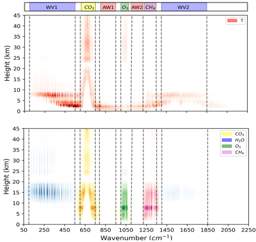
Figure 2. Absolute values of normalized Jacobians computed with \sigma -IASI for a tropical standard atmosphere with respect to the temperature (top panel) and gases concentration (bottom panel). \text{N}_2\text{O} Jacobian is not shown because \text{CH}_4 Jacobian completely overlaps it.
