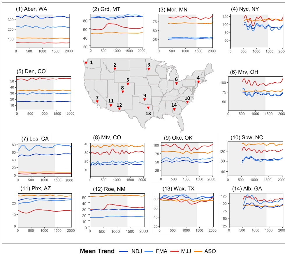
375 Figure 7. Long-term trends of averaged 3 months precipitation(mm/month) for 4 seasons. The periods before 1400 CE are shaded to represent the period with less prediction skills in original NASPA.
