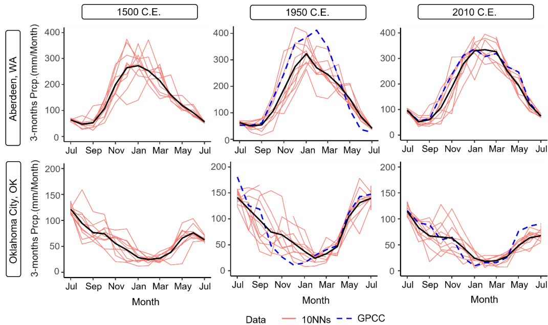
280 Figure 3. Comparing downscaled NASPA (Black), 10 Nearest Neighbors (pink) and GPCC (blue dashed) at Aberdeen, WA (upper) and Oklahoma City, OK (lower). The marked month in X-axis refers the last month of 3months-rolling average.
