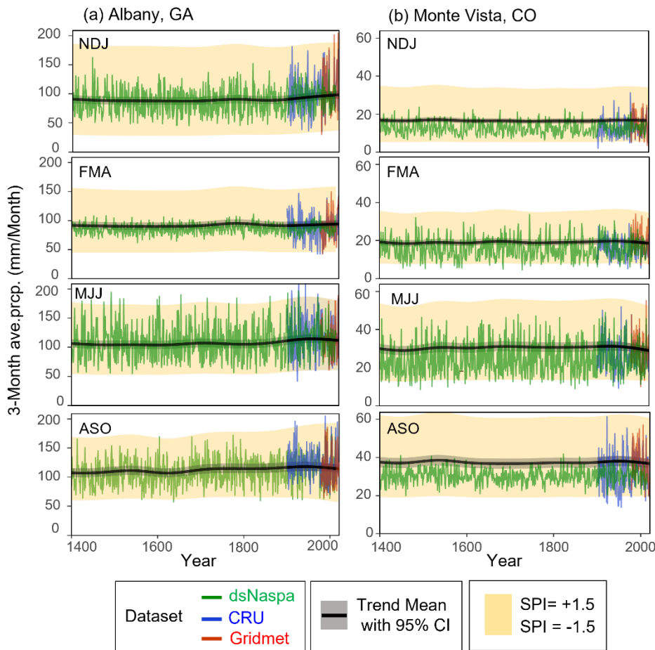
355 Figure 6. Long-term trends in 3 months NSPI (black line) and averaged precipitations in four periods. The yellow shaded area represents the 95% percentile for the Gamma distribution, so that the upper and lower boundary represents SPI 1.5 and -1.5, respectively. Trends in the mean and SPI = -1.5 to +1.5 range are shown using Gridmet as baseline to illustrate bias correction, while the raw data is shown without bias correction for context.
