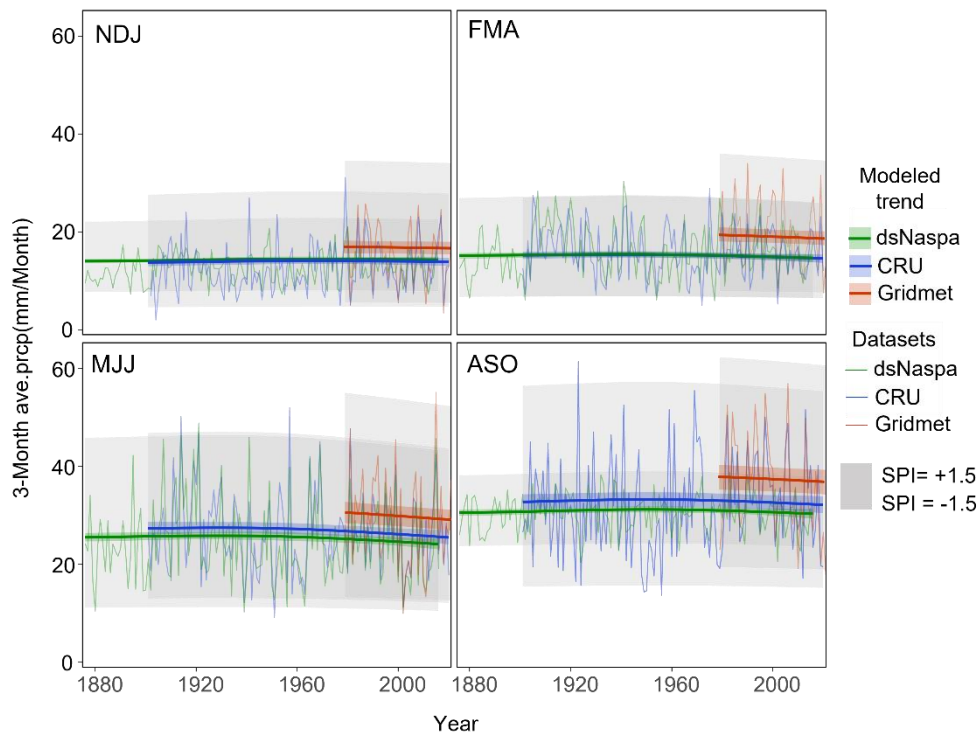
330 Figure 5. Long-term trends of each dataset for 4 periods at Monte Vista, CO. Mean parameter estimates for each dataset are represented as differently colored lines, while the SPI -1.5 to 1.5 range for each dataset is indicated by grey regions.
