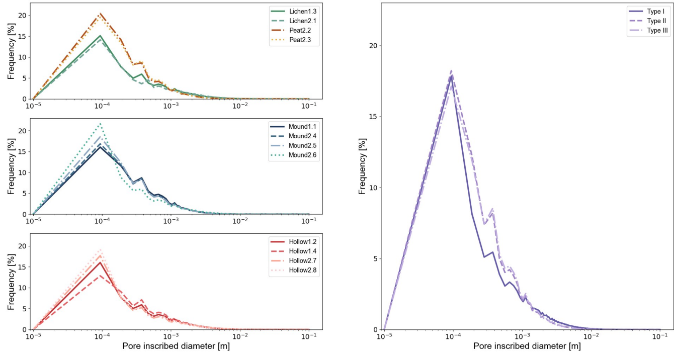
Figure 5: Incribed pore size distribution by classified type using particles' Feret diameter measurement. An averaged value is computed for each sample type, each colour nuance representing each type.
