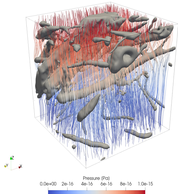
1035 Figure 9: (Left) Pressure field (in Pa) after a single-phase flow simulation thorough a pore network model based on Mound2.5 sample. Spherical pore sizes are represented according to their respective size in the network. (Right) Pressure field lines (in Pa) after a single-phase flow simulation through a sub-sample of Hollow2.8 sample. The gray mesh corresponds to the isolated biological phase.
