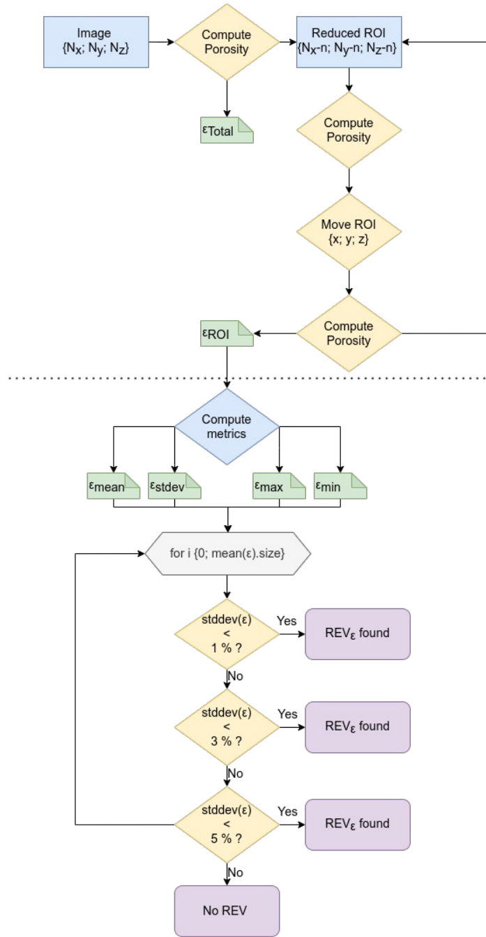
Figure 3: Flowchart of Representative Elementary Volume of Porosity (REV ε ) from binarized image. For each sample, three thresholds are tested (5 %, 3% and 1 % and standard deviation variation).
