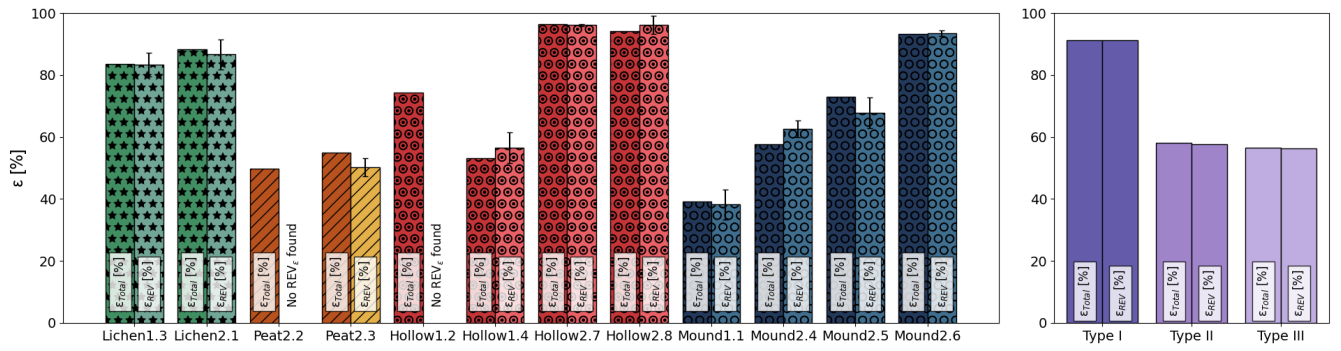
1025 Figure 7: Numerical porosity estimations [in %] for each sample. An averaged value is computed for each identified sample type (I, II, III) with corresponding color nuances. Peat 2.2 and Hollow1.2 did not admit any REV.
