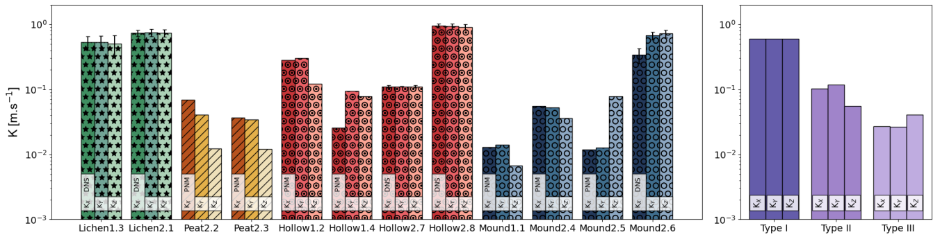
1030 Figure 8: Diagonal components of the hydraulic conductivity tensor (in \text{m.s}^{-1} ) in x ( K_{xx} ), y ( K_{yy} ) and z axis ( K_{zz} ) based on Direct Numerical Simulations (DNS) on Representative Elementary Volume of hydraulic conductivity ( \text{REV}_K ) for Type I samples and with a Pore Network Model (PNM) for Type II and III samples.
