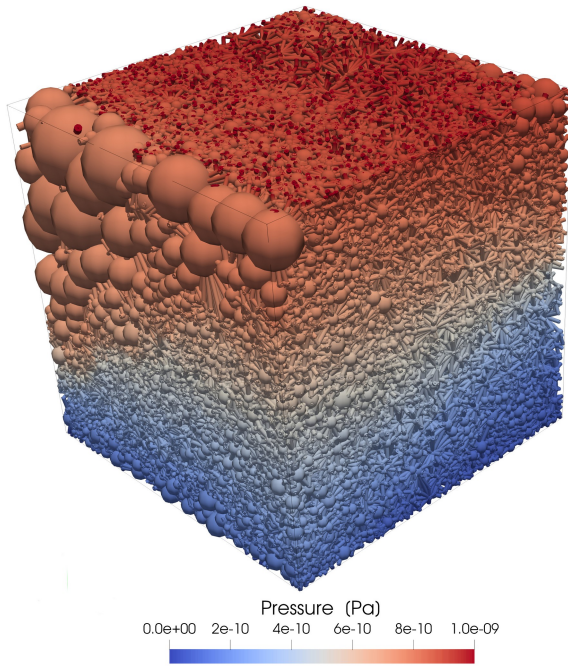
1035 Figure 9: (Left) Pressure field (in Pa) after a single-phase flow simulation thorough a pore network model based on Mound2.5 sample. Spherical pore sizes are represented according to their respective size in the network. (Right) Pressure field lines (in Pa) after a single-phase flow simulation through a sub-sample of Hollow2.8 sample. The gray mesh corresponds to the isolated biological phase.
