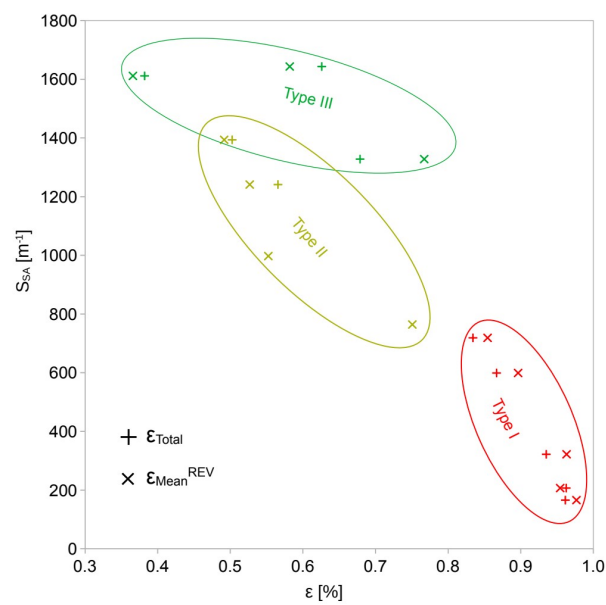
Figure 11: Specific Surface (in m^{-1} ) as a function of total porosity \epsilon_{Total} [%] and Representative Elementary averaged porosity \epsilon_{mean}^{REV} [%].
