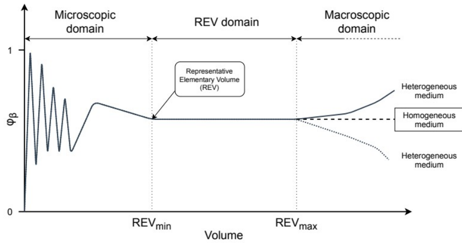
1000 Figure 2: Schematic representation of fluctuations of a generic property \phi_\beta in conjunction with volume (adapted after Brown & Hsieh, 2000).
