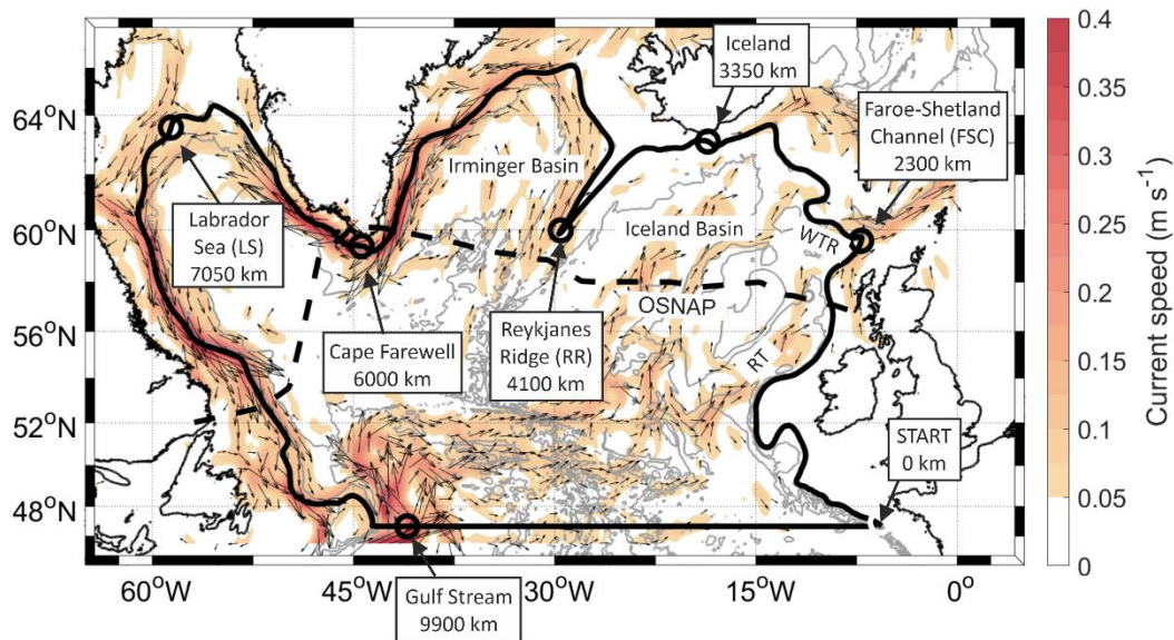
90 Figure 1. Smoothed 1000 m bathymetry contour (solid black line), closed by transect across 47° N. Key locations around contour are labelled; these are used throughout this study. Dashed black line shows OSNAP line. RT: Rockall Trough, WTR: Wyville Thomson Ridge. Mean magnitude and direction of surface currents (2000-2020) derived from AVISO data shown by coloured contours and quiver arrows. Isobaths overlaid at 1000 m increments. Bathymetry contours from GEBCO bathymetry ( http://www.gebco.net/ ). GEBCO = General Bathymetry Chart of the Oceans.
