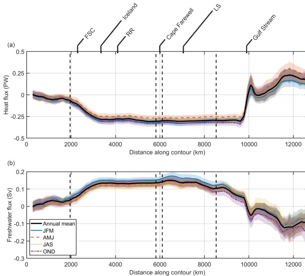
590 Figure 10: Cumulative heat [PW] and fresh water [Sv] fluxes into the SPG between surface and seabed for (a) heat and (b) freshwater, using corrected velocities for sub-1000 m currents. Key locations around boundary labelled as for Fig. 3, vertical dashed lines denote OSNAP crossings.
