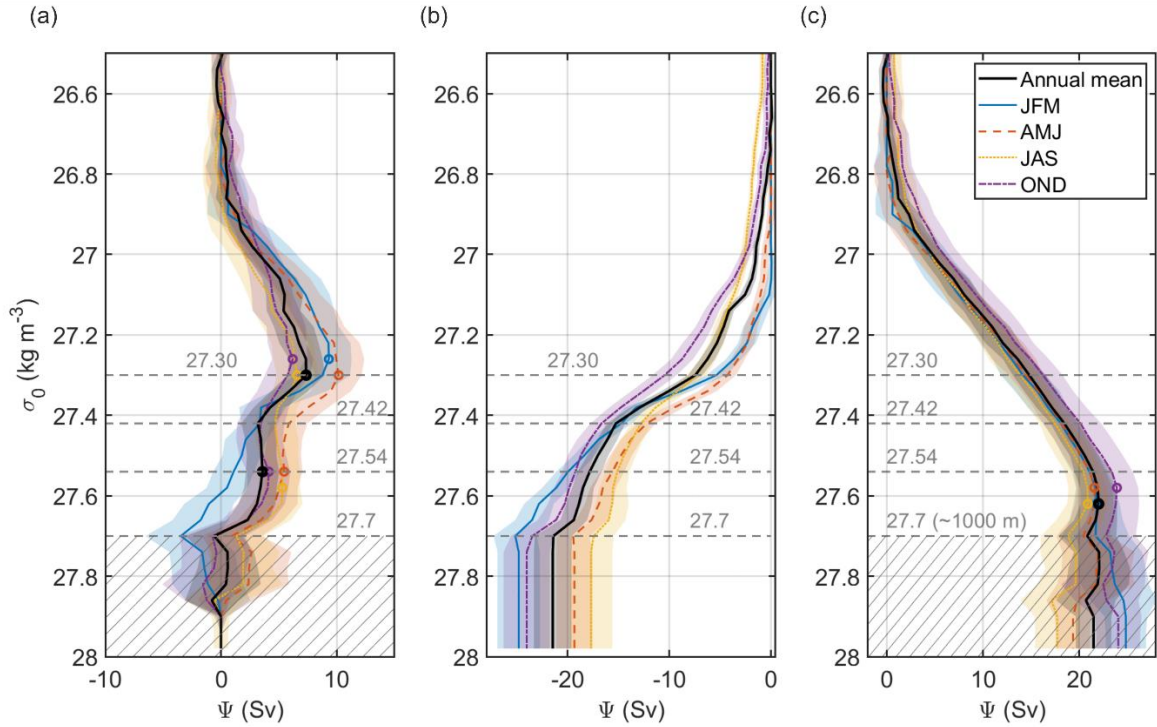
555 Figure 9: (a) Overturning stream function \psi for full SPG boundary in density space between surface and seabed using corrected velocities for sub-1000 m currents. Density of maximum overturning, and that of secondary peak where applicable, highlighted by circles. Densities of mean inflection points marked by horizontal grey dashed lines; these are overlaid on Fig. 3c and d. The hatched area denotes the approximate density space impacted by the sub-1000 m correction velocities (see Supplementary Materials S5 for details). (b) same, but for boundary contour (0-9500 km) only, (c) same, but for 47° N transect (9500 – 12700 km) only.
