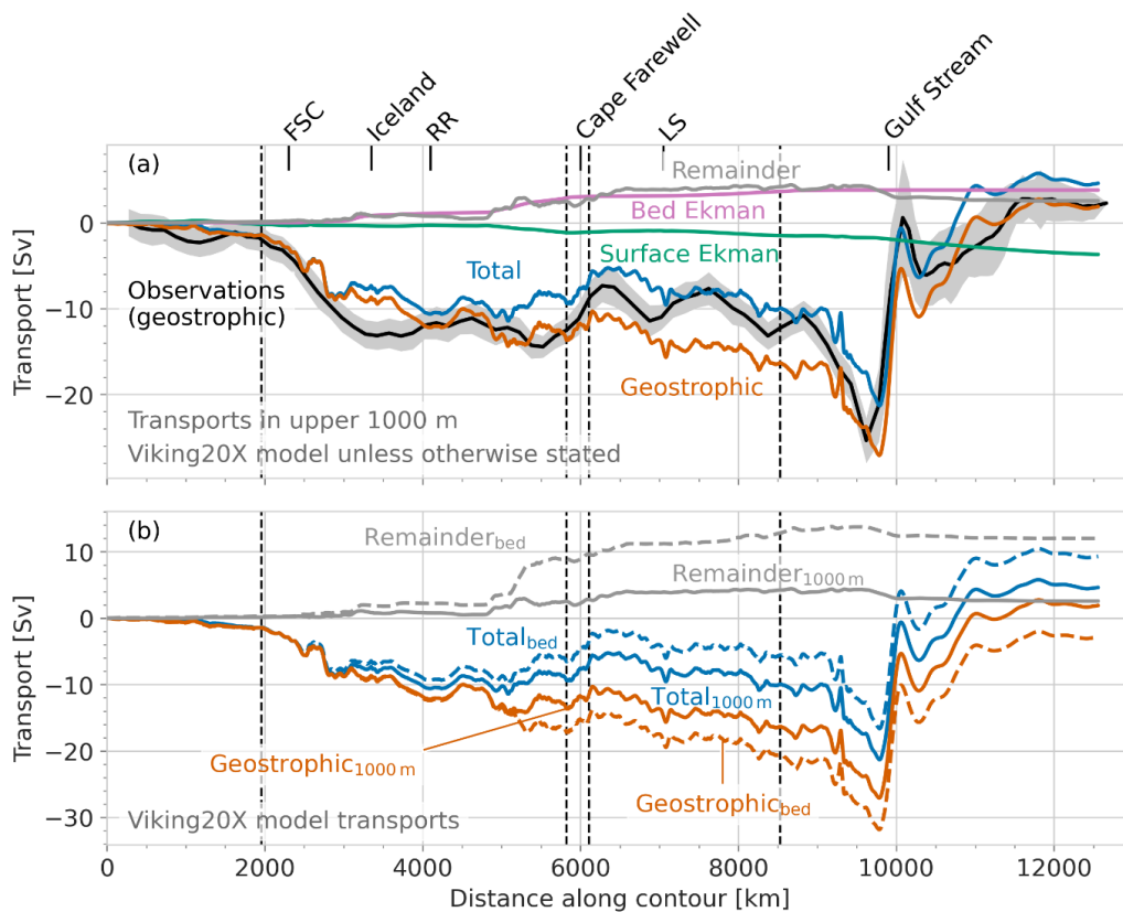
505 Figure 7: (a) Comparison between observed cumulative geostrophic volume transport into the SPG (annual mean) and transport components above 1000 m in VIKING20X. Key locations around boundary labelled as for Fig. 3, vertical dashed lines denote OSNAP crossings. Remainder is calculated as (total – geostrophic - surface Ekman – bed Ekman). (b) Comparison between transports into the SPG in VIKING20X using a strict 1000 m cutoff, and integrating to the bed along the 1000 m contour (but still integrated to 1000 m across 47° N). The difference is due to the stepped model topography and associated inability to follow the 1000m bathymetry precisely.
