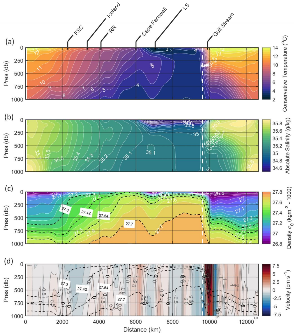
370 Figure 3: Gridded boundary product plotted by distance along the 1000 m contour travelling anti-clockwise around the basin. Annual means shown. (a) conservative temperature ( ^{\circ}\text{C} ), (b) absolute salinity ( \text{g kg}^{-1} ), (c) density ( \sigma_0 , \text{kgm}^{-3} ), (d) geostrophic velocities across the boundary perpendicular to the 1000 m depth contour ( \text{cm s}^{-1} , positive into the interior, negative out of the interior, colour map intervals of 0.25 \text{ cm s}^{-1} with selected contours shown). Density contours relevant to overturning processes (Fig. 9) shown by black dashed lines in 375 (c) and (d) . The transition to the 47^{\circ} N section, and from gridded CTD to EN4 climatology data, is delineated by the dashed white line. Key locations around boundary labelled. FSC: Faroe-Shetland Channel, southernmost point of Iceland, RR: Reykjanes Ridge (southern tip), Cape Farewell, LS: Labrador Sea, Gulf Stream.
