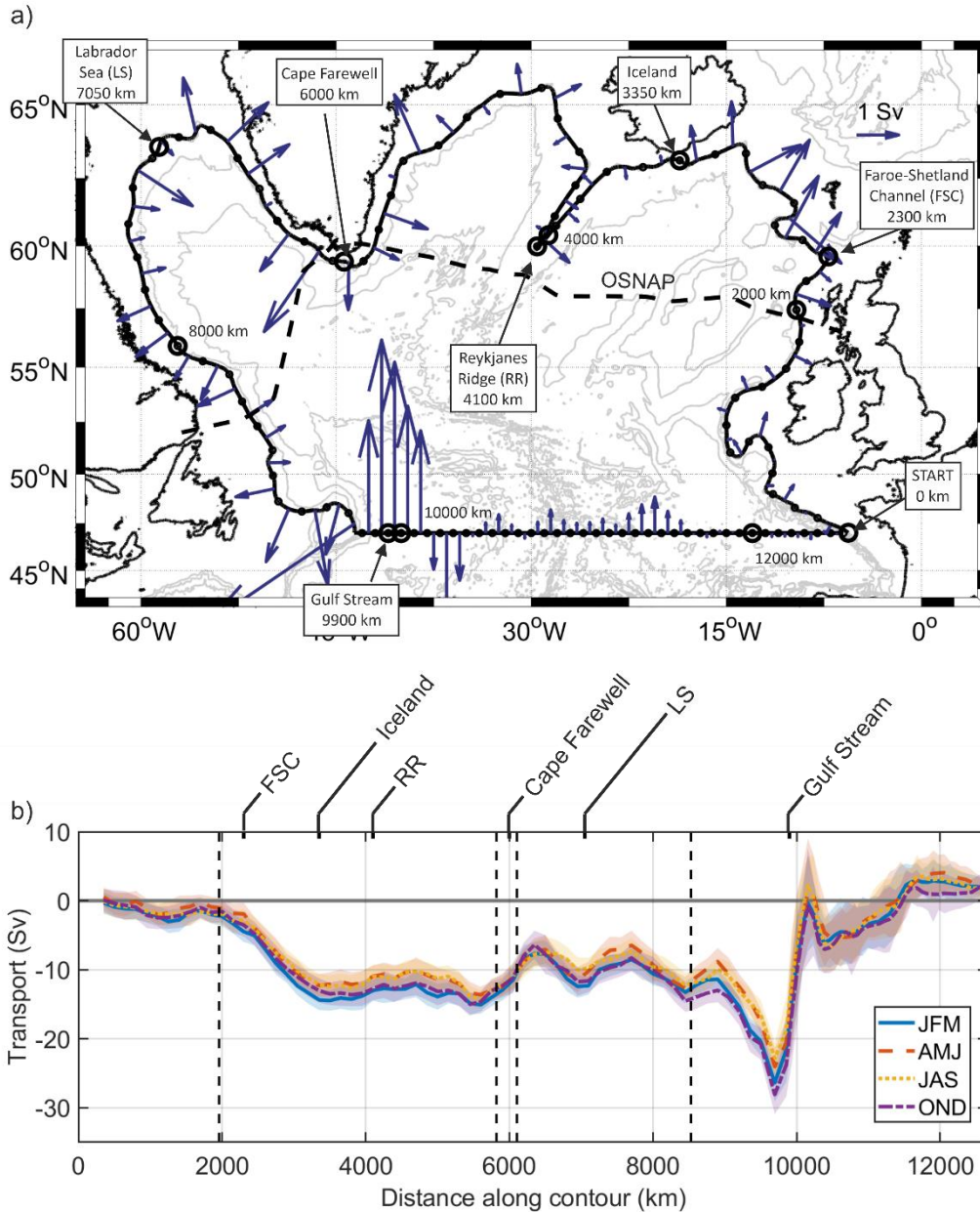
Figure 5: Geostrophic \int_0^{1000} \text{transport perpendicular to contour, into the SPG positive. a) Depth integrated volume transport between 0 and 1000 m for each grid cell (timeseries/annual mean). Quiver arrows show magnitude of transport across grid cell, and are constrained to be perpendicular to the section. Horizontal bins are 150 km apart around the 1000 m contour, and 1° across 47° N. Bathymetry contours from GEBCO bathymetry ( http://www.gebco.net/ ). GEBCO = General Bathymetry Chart of the Oceans. (b) Cumulative volume transport around basin, for each season. Key locations around boundary labelled as for Fig. 3, vertical dashed lines denote OSNAP crossings.
