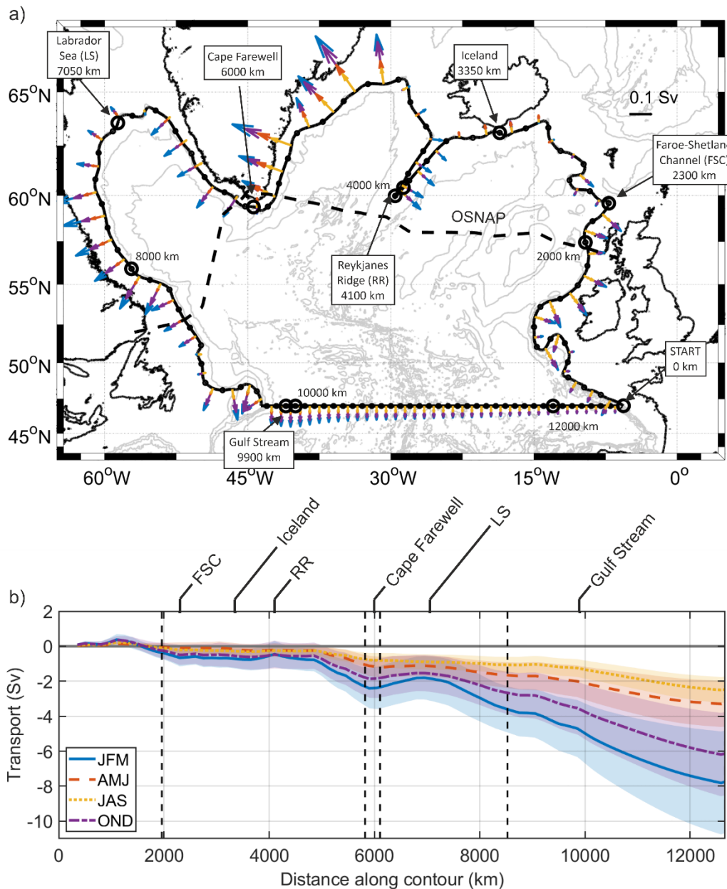
450 Figure 6: Surface Ekman transport perpendicular to contour, into the SPG positive. (a) volume transport between 0 and 1000 m for each grid cell, coloured by season. Quiver arrows show magnitude of transport across grid cell, and are constrained to be perpendicular to the section. Horizontal bins are 150 km apart around the 1000 m contour, and 1° across 47° N. Bathymetry contours from GEBCO bathymetry ( http://www.gebco.net/ ). GEBCO = General Bathymetry Chart of the Oceans. (b) Cumulative volume transport around basin, for each season. Key locations around boundary labelled as for Fig. 3, vertical dashed lines denote OSNAP crossings.
