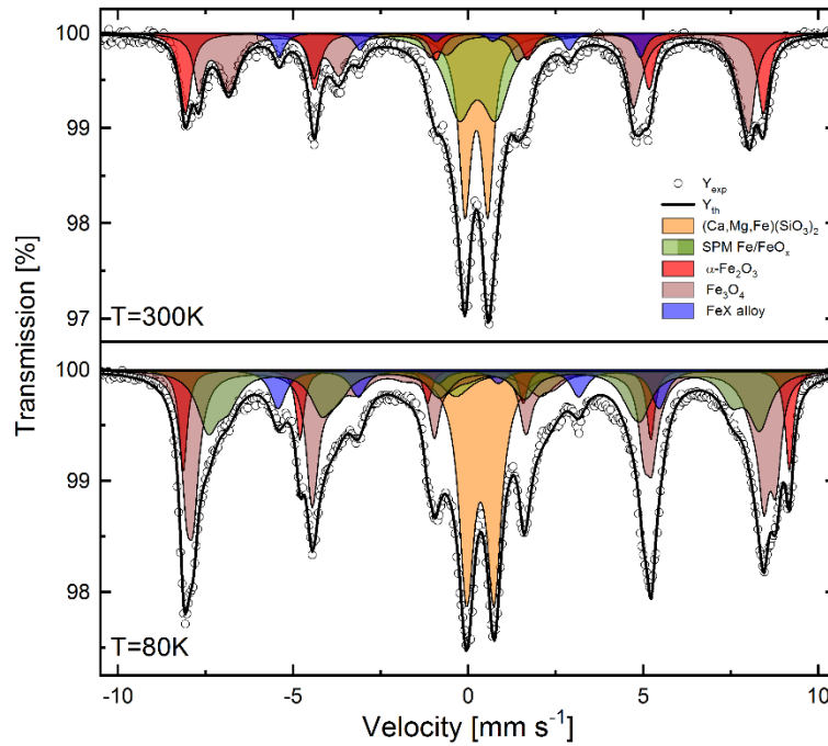
Fig. 7. Mössbauer spectra measured at room temperature (top) and at 80 K (bottom). For detailed explanation and the hyperfine interaction parameter of the components used for fitting the spectra, see the text and Table 2.
