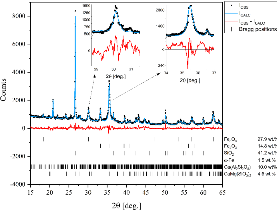
150 Fig. 3. X-ray diffraction pattern measured at room temperature. The black circles stand for measured data, the blue line is calculated spectra obtained assuming material composition as indicated, and the red line denotes the difference between the observed and calculated intensities. Calculated positions of the diffraction peaks for each phase are indicated as bars.
