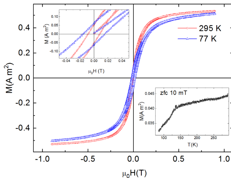
Fig. 8. Magnetic hysteresis loops up to 0.9 T at room temperature (red) and at 77 K (blue). Top-left inset: close-up of the area close to the zero field. Inset bottom right: ZFC curve between 300 K and 77 K.
