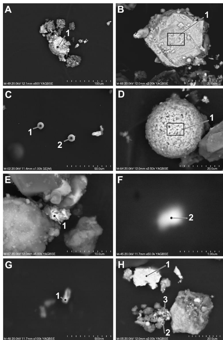
Fig. 5. Size and morphology of Fe-rich particles and particles dominated by other than Fe metals or with high content other elements (SEM; backscattered electron images except C – secondary electrons). A. Irregular particles bigger than 20 μm; B. Irregular particles bigger than 20 μm; C. Aluminosilicate sphere (left) and Fe-dominated sphere (right); D. Spherical particle rich in Ca and Fe; E. Particle rich in Pb; F. Particle rich in Zr; G. Particle rich in Au; H. Particles with high content of other than Fe metals; (see table 1 for the results of the chemical composition measurements of the indicated particles).
