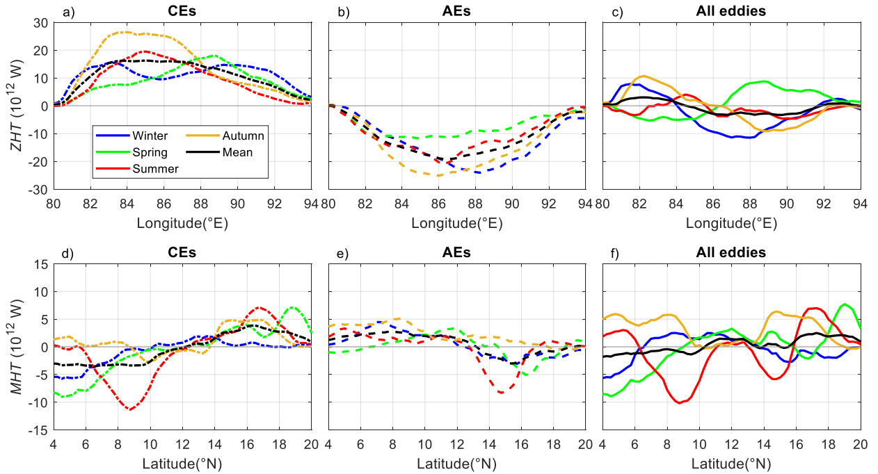
Figure 10: The meridionally integrated zonal heat transport ( ZHT , upper panels) at different longitudes, and the zonally integrated meridional heat transport ( MHT , lower panels) at different latitudes by cyclonic eddies (CEs), anticyclonic eddies (AEs), and all eddies in different seasons in the Bay of Bengal.
