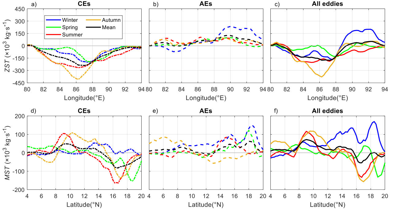
Figure 13: The meridionally integrated zonal salt transport ( ZST , upper panels) at different longitudes, and the zonally integrated meridional salt transport ( MST , lower panels) at different latitudes by cyclonic eddies (CEs), anticyclonic eddies (AEs), and all eddies in different seasons in the Bay of Bengal.
