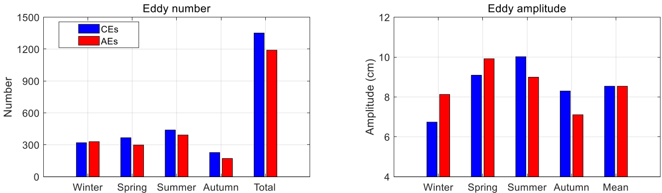
Figure 3: The eddy number and amplitude of monthly cyclones (CEs) and anticyclones (AEs) in different seasons based on monthly averaged sea level anomaly fields from January 1993 to February 2019 in the Bay of Bengal.
