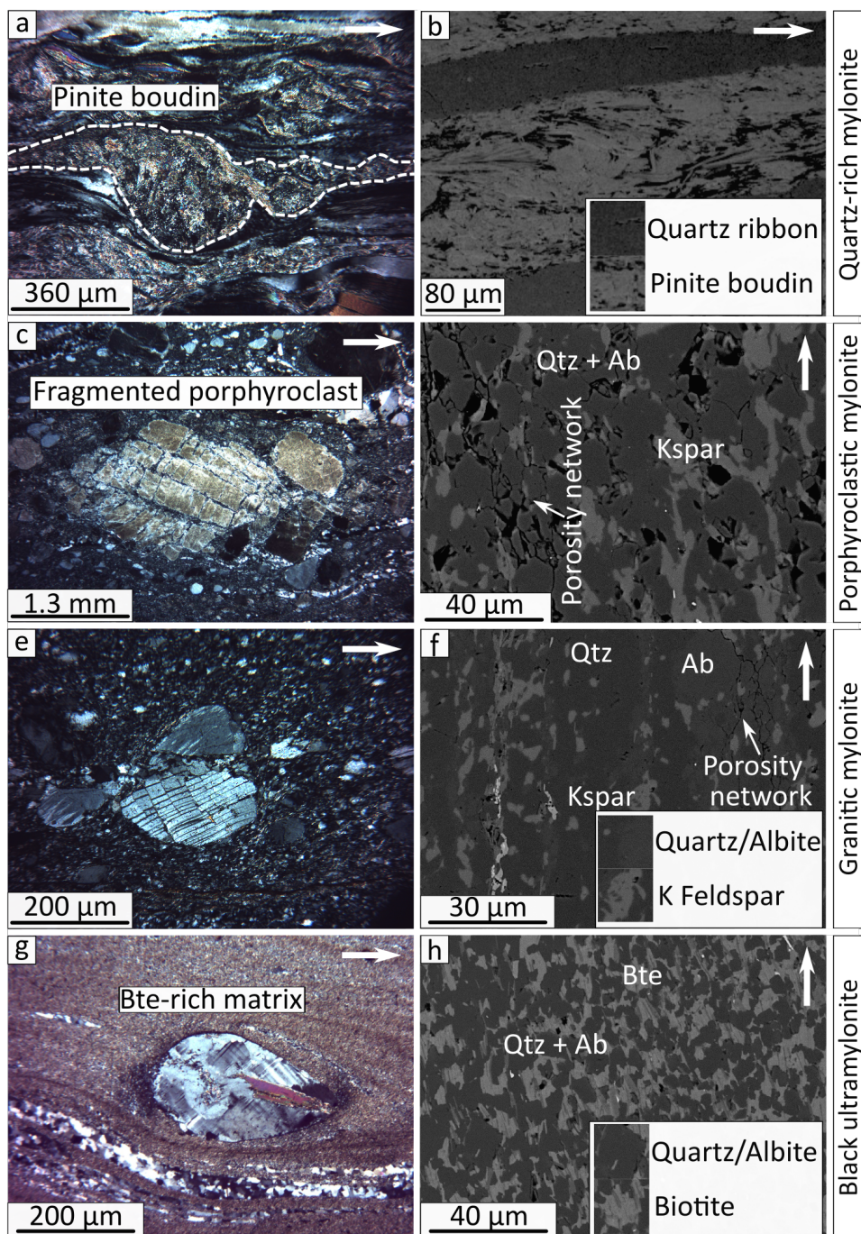
Figure 4. Characteristic microstructure of different Pofadder mylonites (left), with BSE image of fine-grained matrices (right). (a) Pinite pseudomorphing boudinaged cordierite in quartz-rich mylonite. (b) Pinite band bounded by quartz ribbons. (c) Large fragmented porphyroclast of sericite-altered feldspar in porphyroclastic mylonite. (d) Quartz/albite (darker grey) and potassium feldspar (medium grey) in the matrix of porphyroclastic mylonite. Intergranular porosity is black. (e) Fragmented plagioclase porphyroclast in granitic mylonite. (f) Quartz (darkest grey), albite (dark grey) and potassium feldspar (light grey) composing granitic ultramylonite matrix. Intergranular porosity is black and muscovite is white. (g) Rounded porphyroclast in black ultramylonite. (h) Well-distributed biotite (light grey) and quartz/albite (dark grey) matrix in black ultramylonite. Intergranular porosity is black. Thin section orientation is indicated with a white arrow directed to the NW in each panel.
