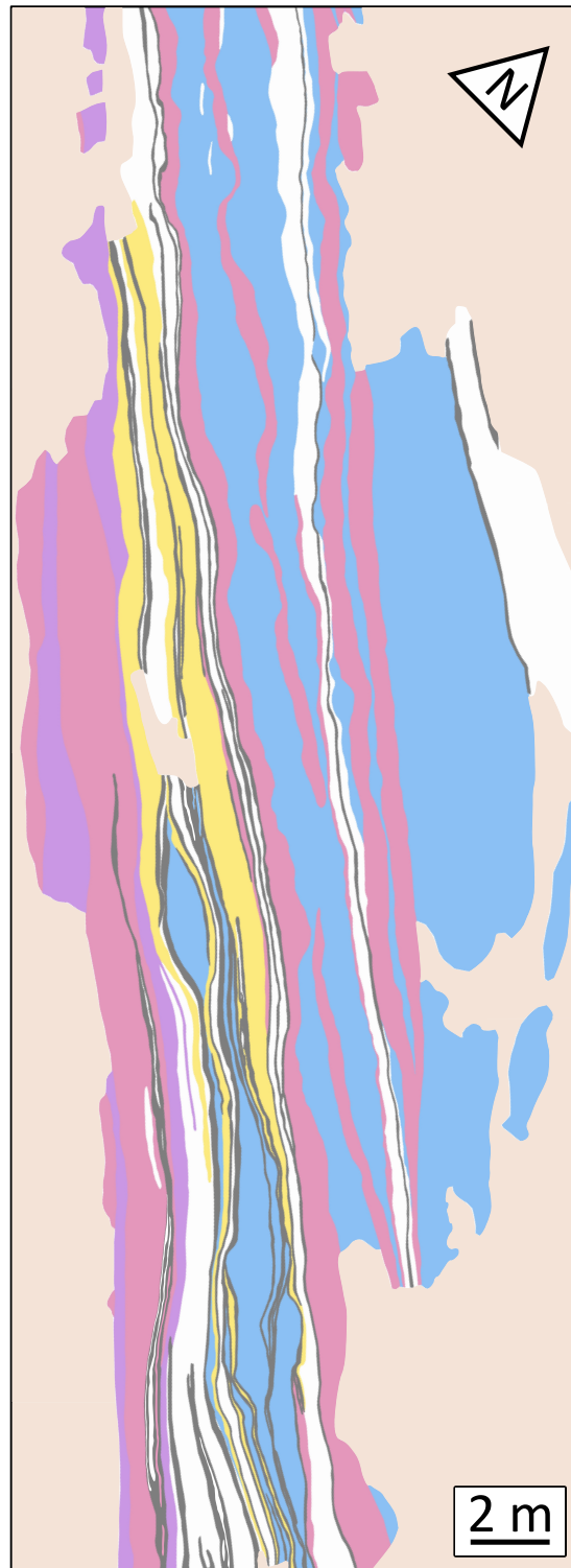
Figure 2. Map of the Coboop Island fault core showing major mylonite units and Quaternary cover. Stereonet is rotated to match the orientation of the map, and contains contoured measurements of poles to foliation (circles) and lineations (triangles). High resolution basemap and map structural measurements are included as supplementary material.
