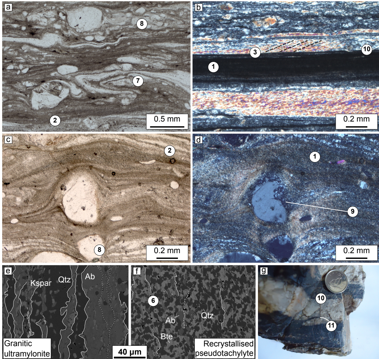
Figure 6. Pseudotachylyte / black ultramylonite microstructures. Numbers in circles highlight microstructural identification criteria listed in the text. a: Flow folds (2) including eddies around polycrystalline (7) and quartz (8) survivor clasts in layered biotite-rich/quartz matrix. b: Isotropic pseudotachylyte (1) sharply cross cuts (10) grain shape preferred orientation in granitic mylonite layer (3). Note the colours are skewed toward brighter interference colours because the section is slightly thicker than 30\ \mu\text{m} , which emphasizes the crystallographic preferred orientation. c-d: Same field of view; c is non-polarized transmitted light and d is cross-polarized. Embayed feldspar survivor grain (8) with mantle of feldspar-rich matrix (9) interpreted as partially melted and dragged along flow banding (2; toward the right side away from the grain) forming a tail of quartz-enriched pseudotachylyte within the mixed-biotite-quartz matrix (1). e-f: SEM backscatter images of granitic ultramylonite ( e ; same as Figure 4f) and black ultramylonite ( f ; same as Figure 4h) matrices. Interconnected porous horizons (annotated with sparse dashed lines) and phase boundaries extending along multiple grain boundaries (annotated with solid lines; 6). g: An injection vein is shown in hand sample.
