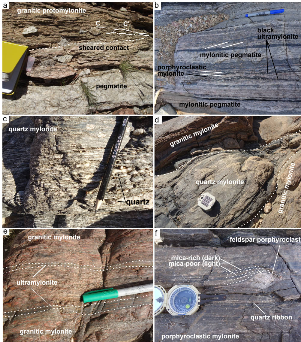
Figure 3. Field photographs of lithologies found in the Coboop Island shear zone core with selected layer interfaces indicated with dotted lines. All photos oriented with NW to the right, SE to the left. (a) Granitic protomylonite with sheared intrusive pegmatite contact. Field notebook edge is 12 cm. (b) Layers of mylonitic pegmatite, porphyroclastic mylonite, and black ultramylonite crosscutting foliation at low angle (white lines). Pen is 10 mm wide. (c) Quartz-rich mylonite with strongly aligned and tailed quartz aggregates, interlayered with aluminosilicate-rich matrix. Pencil is 8 mm wide. (d) Boudinaged quartz-rich mylonite contained between layers of granitic mylonite. Compass is 70 mm wide. (e) Granitic mylonite cut by granitic ultramylonite horizons. Pen is 10 mm wide. (f) Porphyroclastic mylonite with feldspar porphyroclast derived from pegmatite protolith, wrapped by foliation layers of variable mica content. Compass is 70 mm wide.
