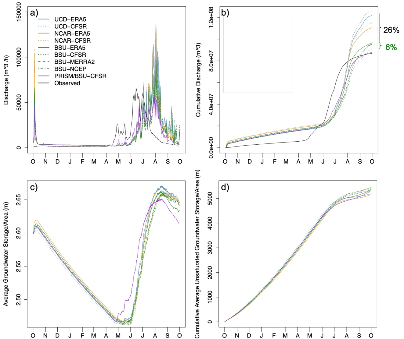
80 Figure 7. Time-series of ParFlow-CLM simulations of discharge rate (a), cumulative discharge (b), groundwater storage per unit area of the watershed (c), and cumulative average unsaturated groundwater storage per area of the watershed (d) for the IPM configurations described in Table 2. The brackets on the far-right indicate the percent difference of cumulative discharge and unsaturated groundwater storage per area (b and d, respectively) for WRF simulations across different meteorological forcings (green) and subgrid-scale physics schemes (black).
