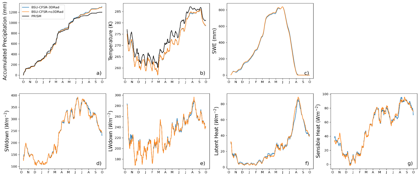
Figure 5. Spatial-average cumulative precipitation, two-meter surface air temperature and snow water equivalent (SWE) (first row), shortwave and longwave radiation, and latent and sensible heat (second row) over the ERW as simulated by the IPM configurations with and without realistic topographic radiation effects, along with, where available, estimates from PRISM. 3DRad indicates a simulation with topo_shading and slope_rad turned on in the WRF inner domain but not the outer WRF domains, no3DRad indicates a simulation with topo_shading and slope_rad turned off in both the inner and outer WRF domains. 10-day moving averages are shown in b) temperature, and radiation variables (d, e, f, g).
